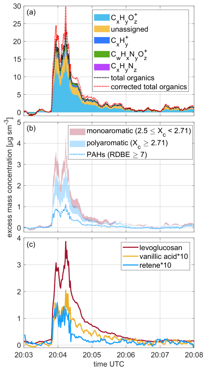
Figure 2. 1-Hz time series of excess mass concentrations of (a) total uncorrected organics and total fragmentation-corrected organics as well as CH, CHO, CHN and CHNO compound classes, (b) monoaromatic and polyaromatic compounds together with PAHs (section 2.5 should be consulted for details and limitations) and (c) levoglucosan, vanillic acid and retene as measured by the CHARON PTR-ToF-MS instrument during a wildfire plume penetration over the Sierra Nevada Mountains in California. A 10-s moving average filter has been applied to data outside the plume.
