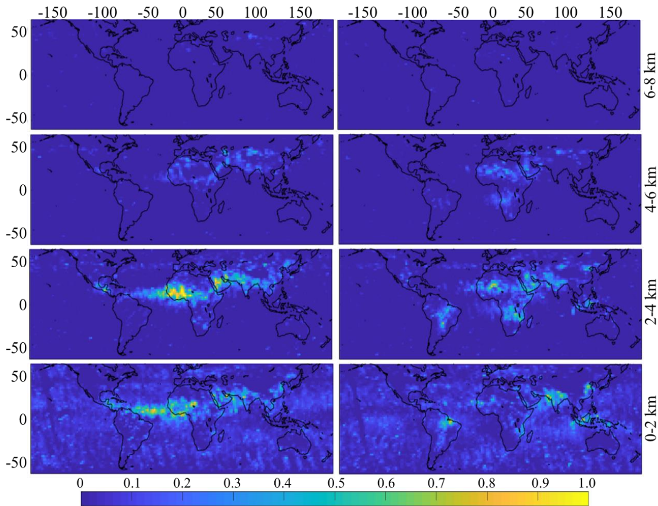
Figure 2 Height-resolved global distributions of aerosol optical depth (AOD) based on construction of RXS expanded 100km on both sides of CALIPSO's ground-track. Left column is for the April dataset and the right column is for September . Data are binned on a 2 °lat/long grid.
