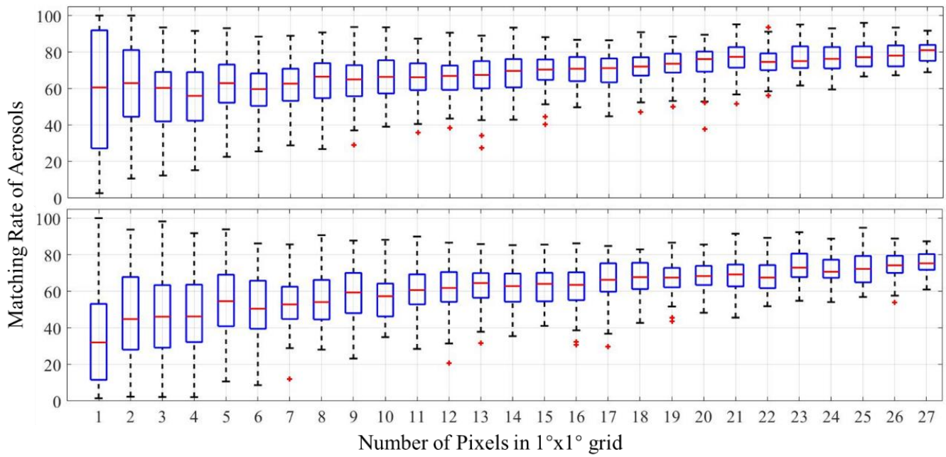
5 Figure 4-3 Matching rates of aerosols as a function of number of samples in 1^\circ grid cells for reconstructions of nadir profiles with 30km dead zone (top) and 100km dead zone (bottom). Boundaries of each box represent the 25th and 75th percentiles of the sample data in the grid, red lines indicate medians, and whiskers correspond to approximately \pm 2.7\sigma (99.3 percent coverage assuming data are distributed normally). Points marked with '+' are extreme outliers.
