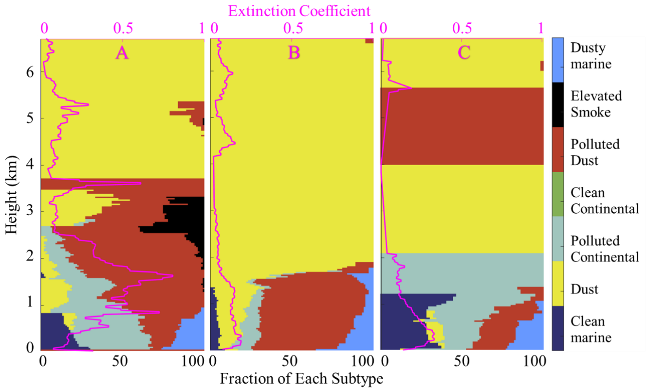
Figure 6-5 Vertical distributions of each aerosol subtypes in region A, B, and C (see Fig.5). Pink lines show profiles of average aerosol extinction coefficient ( \text{km}^{-1} ). The fraction is calculated as the occurrence of each subtype divided by the total occurrence of aerosols in each region.
