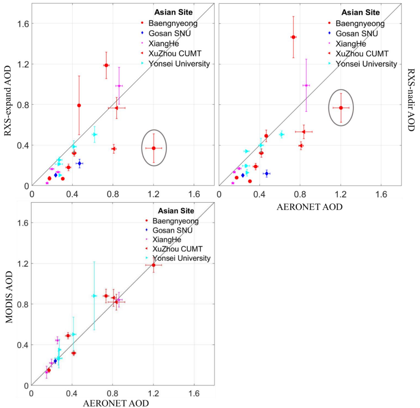
Figure 8 Comparison of collocated measurements of RXS-expand and AERONET (upper left), RXS-nadir and AERONET (upper right), and MODIS and AERONET (lower left). Error bars in y-direction indicate standard deviations of RXS-expand, RXS-nadir or MODIS measurements within 50 km of the site, and in the x-direction AERONET measurements within \pm 2 hour of CALIPSO's passing. Grey circles mark a notable outlier.
