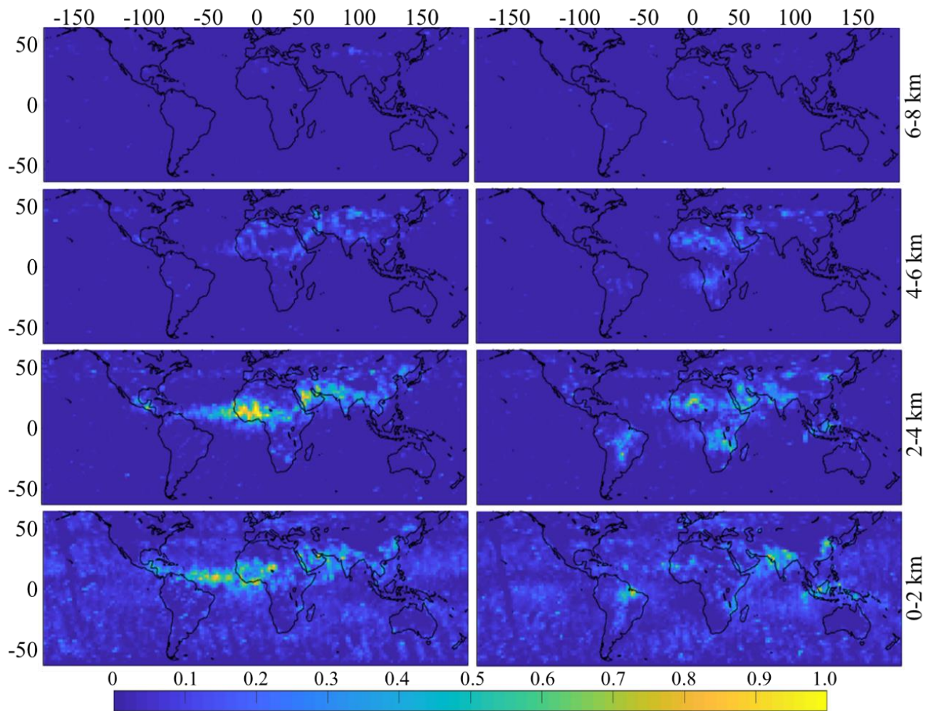
Figure 3 Height-resolved global distributions of aerosol optical depth (AOD) based on construction of RXS expanded 100 km on both sides of CALIPSO's ground-track. Left column is for the April dataset and the right column is for September . Data are binned on a 2°lat/long grid.
