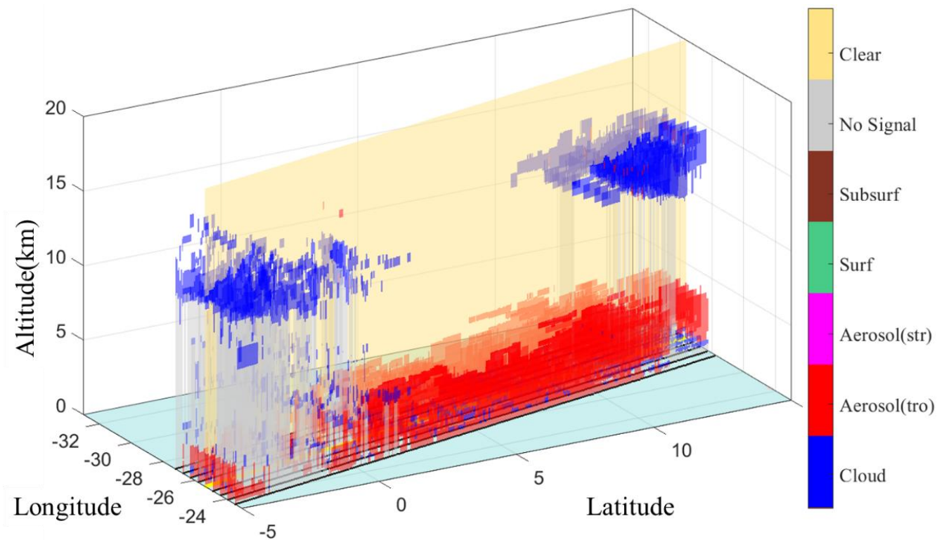
Figure 2 Demonstration of the expansion of the active-passive retrieved cross-section (RXS), which runs through the centre, for a transect near Africa-Atlantic coast between 15 °N and 5 °S on 23 April 2015.
