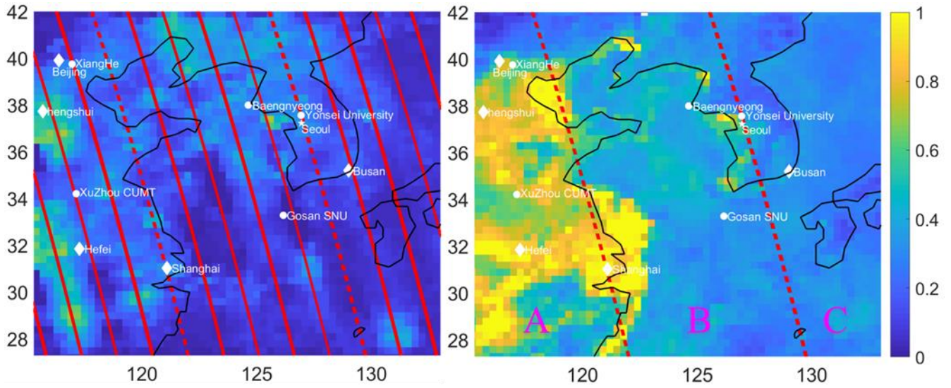
5 Figure 5 Seasonal distribution of aerosol optical depth (AOD) between 117^{\circ}\text{E} - 132^{\circ}\text{E} , 26^{\circ}\text{N} - 41^{\circ}\text{N} for March to May, 2015 based on RRS-expand (left) and MODIS (right). Lines mark CALIPSO ground-tracks. Dotted tracks are used as the boundaries for the analysis of aerosol subtypes in Fig. 6. White circles mark AERONET sites. Star marks the AD-Net site at Seoul. Diamonds mark some major cities.
