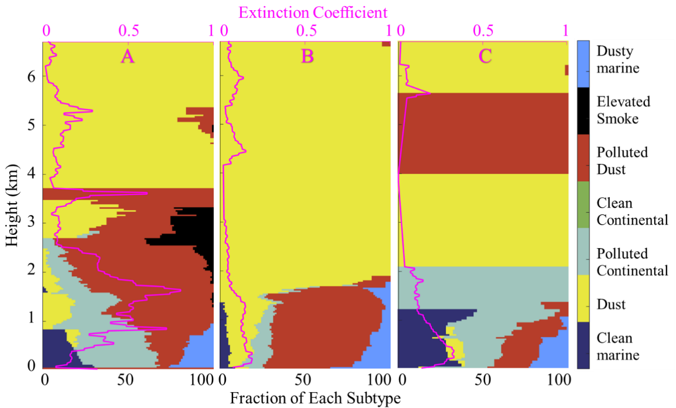
Figure 6 Vertical distributions of each aerosol subtypes in region A, B, and C (see Fig. 5). Pink lines show profiles of average aerosol extinction coefficient (km -1 ). The fraction is calculated as the occurrence of each subtype divided by the total occurrence of aerosols in each region.
