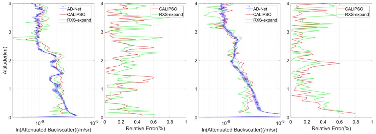
Figure 7 Comparisons among ground-based lidar profiles of 532 nm attenuated backscatter coefficient products (units: \text{m}^{-1}\text{sr}^{-1} , averaged 2 hours within satellite overpass), CALIPSO profiles at shortest distance and RXS-expand profiles averaged 25 km around the location of Seoul station. The two plots on the left are from 7 March 2015, and the two plots on the right are from 24 April 2015.
