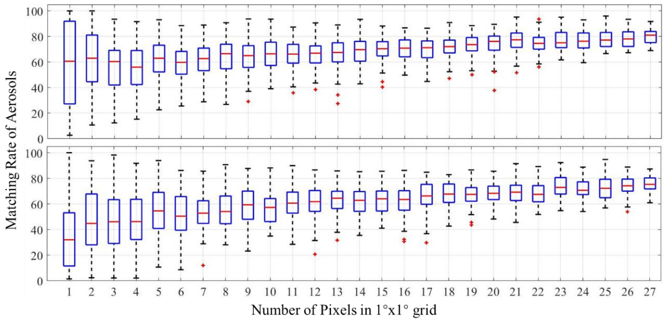
Figure 4 Matching rates of aerosols as a function of number of samples in 1^\circ grid cells for reconstructions of nadir profiles with 30 km dead zone (top) and 100 km dead zone (bottom). Boundaries of each box represent the 25th and 75th percentiles of the sample data in the grid, red lines indicate medians, and whiskers correspond to approximately \pm 2.7\sigma (99.3 percent coverage assuming data are distributed normally). Points marked with '+' are extreme outliers.
