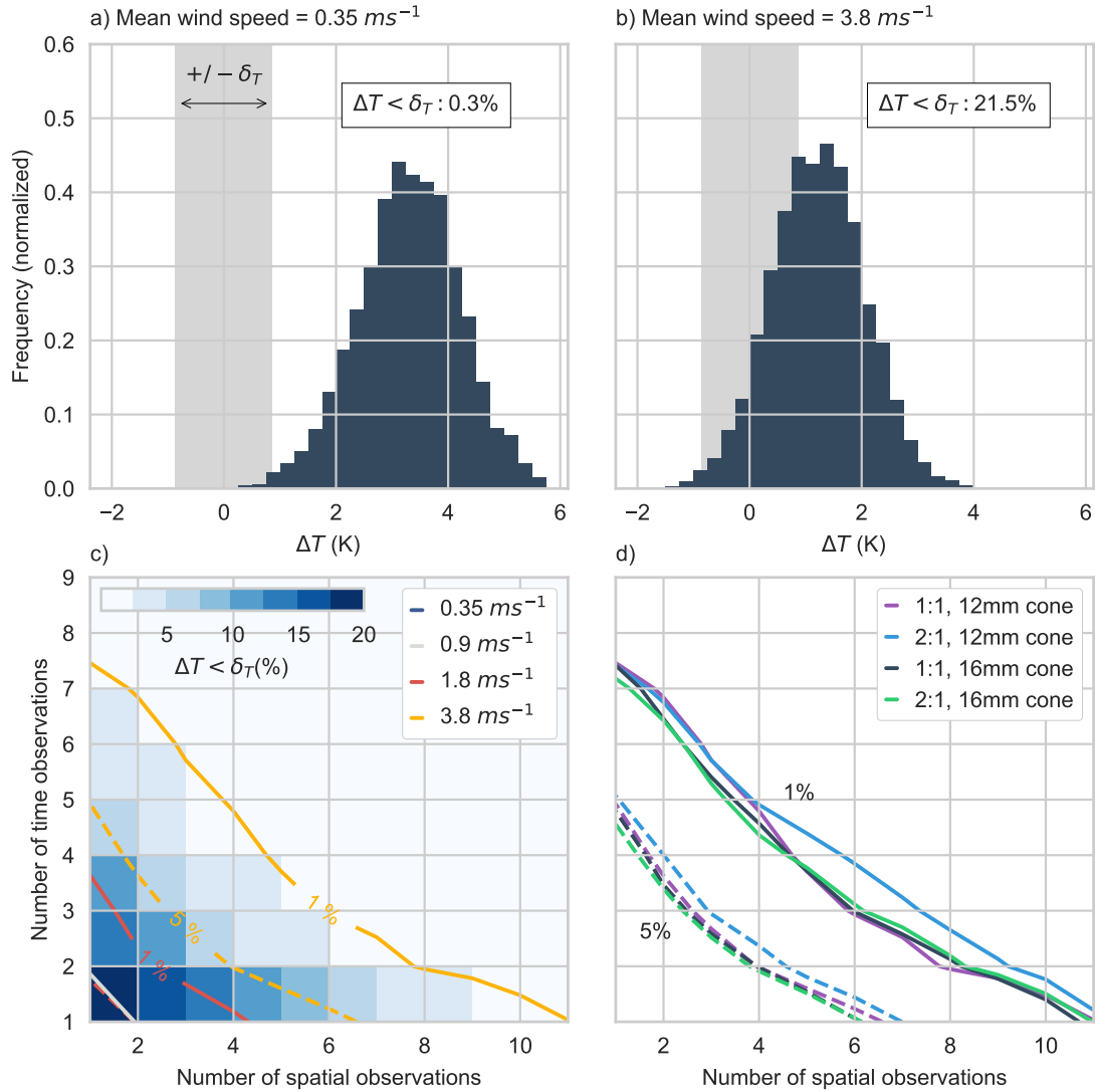
Figure 4. The distribution of temperature differences between cables with opposing cone orientations for the 16mm, 1:1 cones with 2cm spacing and a heating rate of 2.5Wm^{-1} for (a) a wind speed of 0.35ms^{-1} and (b) a wind speed of 3.8ms^{-1} . The grey region indicates the uncertainty, \delta_T . The percentage of observations with \Delta T < \delta_T is indicated. (c) A two-dimensional histogram of the percentage of \Delta T < \delta_T as a function of averaging interval in time and space for the highest wind speed (same data as in b). The contours for the 1% and 5% thresholds are indicated for each wind speed. Note that the 0.35ms^{-1} wind speed is always below the 1% threshold. (d) The 1% and 5% contours for the acceptable cone aspect ratios and sizes at the highest wind speed.
