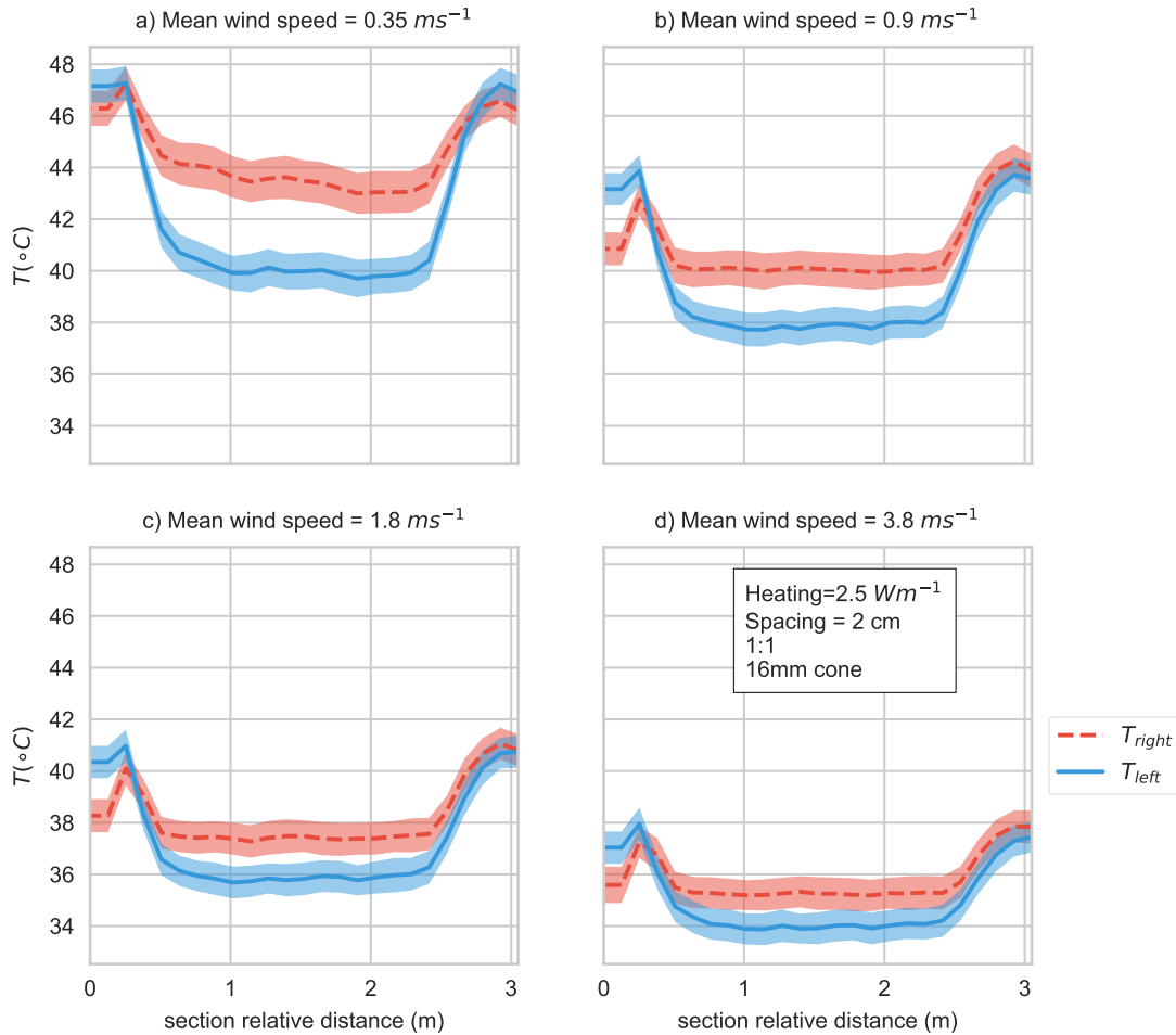
Figure 2. Time-averaged temperature along the test section in the wind tunnel for a horizontal wind speed of (a) 0.35\text{ms}^{-1} , (b) 0.9\text{ms}^{-1} , (c) 1.8\text{ms}^{-1} , (d) 3.8\text{ms}^{-1} for the parameters listed in the Figure. The standard deviation of temperature in time for each point along the FOC is shown in the filled colors. The cones are only present between 0.75m and 2.25 of the tunnel section. The mean wind direction is in the positive x-direction.
