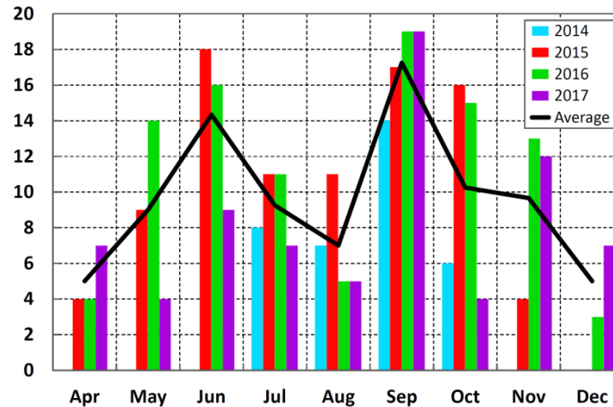
Figure 9: Monthly number of lightning days in the 240 \text{ km} \times 240 \text{ km} domain of better detection accuracy centered on Corsica for 2014 to 2017 years.
