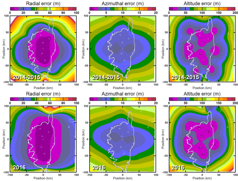
Figure 3: Radial, azimuthal and altitude errors computed with the geometrical model of Thomas et al. (2004) for VHF sources located at 10-km altitude seen from 12 stations. Top: initial SAETTA network in 2014 and 2015; bottom: new SAETTA network since 2016. Stations location is indicated by white squares.
