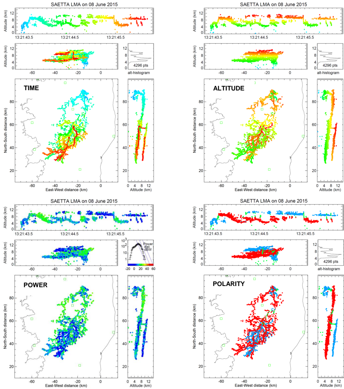
Figure 13: High altitude discharge in the stratiform region during the MCS event of 8 June 2015 at 13:21:43 UT. VHF sources displayed by dots with color scale corresponding to time (top left), altitude (top right), power (bottom left), and cloud charge polarity with positive in red, negative in blue (bottom right).
