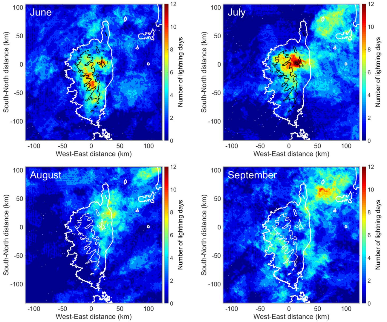
5 Figure 8: Maps of monthly number of lightning days in the 240 \text{ km} \times 240 \text{ km} domain of better detection accuracy centered on Corsica from June to September for 2014 to 2016 years. Isocontours at 1000 m altitude are indicated by black or white lines inside Corsica.
