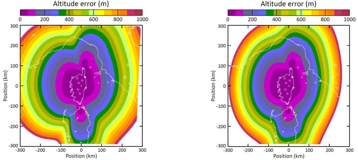
Figure 4: Altitude error computed with the geometrical model of Thomas et al. (2014) for VHF sources at 10 km of altitude seen from 12 stations in a large domain: analysis for the 2016 network (left) and for the same network considered flat with an average altitude of about 863 m (right).
