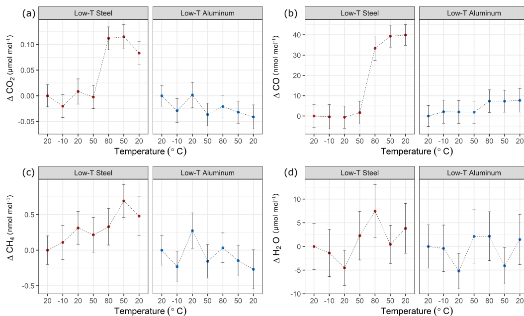
Figure 8. Temperature experiments until 80^\circ\text{C} using steel (red) and aluminum (blue) cylinder for species (a) \text{CO}_2 , (b) \text{CO} , (c) \text{CH}_4 and (d) \text{H}_2\text{O} . x-axis corresponds to a temperature cycle, whereas the y axis shows the amount fraction differences relative to the measurements at 20^\circ\text{C} . Error bars indicate standard deviation of the measurements included in the mean.
