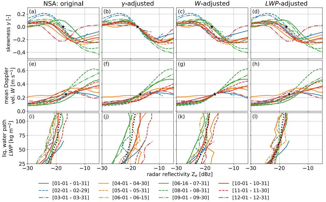
Figure 5. Observed reflectivity Z_e - skewness \gamma (a), Z_e - mean Doppler-velocity W (e), and liquid water path LWP\text{-max}(Z_e) (i) relationships for the North Slope of Alaska (NSA). The data has been calibration corrected using the \gamma method (second column), the W method (third column), and the LWP method (fourth column). The colored lines indicate the various calibration periods of 2016. The black stars (rows 1 to 2) show the reference point used for calibration; the dotted black line (row 3) is the reference LWP\text{-max}(Z_e) relationship obtained from the mean of the monthly relationships weighted by the number of observations.
