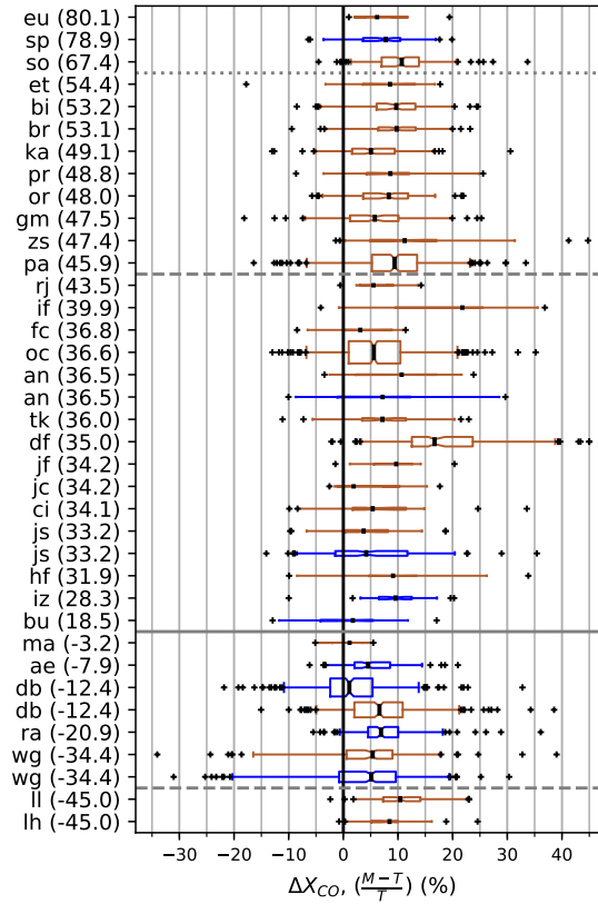
Figure 6. Boxplots of the MOPITT-TCCON percent difference at the TCCON sites (using method II), ordered by latitude (degrees north in parenthesis). Blue boxes are MOPITT soundings over water, brown boxes are over land. Whiskers represent the inner 95 % of data. Notches are 95 % confidence intervals of the median. Box heights represent the relative number of observations. The solid horizontal line is the equator, dashed lines are \pm 45^\circ , and the dotted line is 60^\circ\text{N} .
