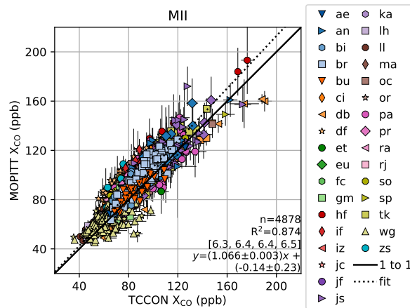
Figure 5. One-to-one plot comparing MOPITT and TCCON, following method II (similar to Wunch et al., 2011b, SM Sect. 6). MOPITT data were adjusted to the TCCON a priori ( \hat{c}'_M ) and MOPITT averaging kernels were applied to TCCON data ( \hat{c}_{M \leftarrow T} ). Error bars represent standard deviations of the weighted averages. Triangles represent soundings over water, other shapes are over land. Text is number of points or days n , coefficient of determination for ordinary least squares regression R^2 , bias (in %) at 50, 75, 100, and 150 ppb using the shown fit, and equation for the shown fit using the methods of York et al. (2004).
