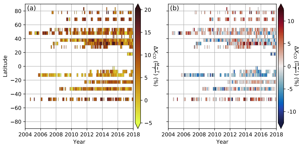
Figure 7. Rotated Hovmöller diagram of the mean percent differences between binned MOPITT and TCCON data using method II (SM Sect 6.1). Latitude bins are 5° zonal bands, and temporal bins are monthly. Left plot is using standard TCCON data. Right plot is without the TCCON scaling to aircraft (WMO scale - see SM Sect. S2).
