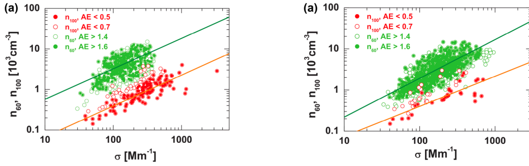
90 Figure R1. Figure 4(a) (left) and Figure 5(a) (right) in the paper of Mamouri and Ansmann (2016).
