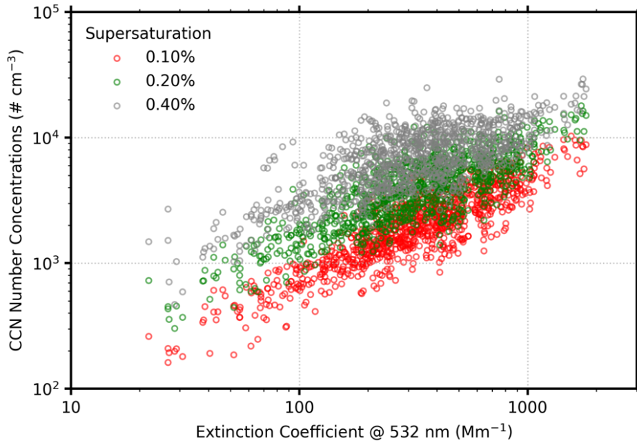
96 Figure R3. Relationship between dry extinction coefficient at 532 nm and CCN number 97 concentrations at supersaturations of 0.10% (red), 0.20% (green), and 0.40% (grey).
