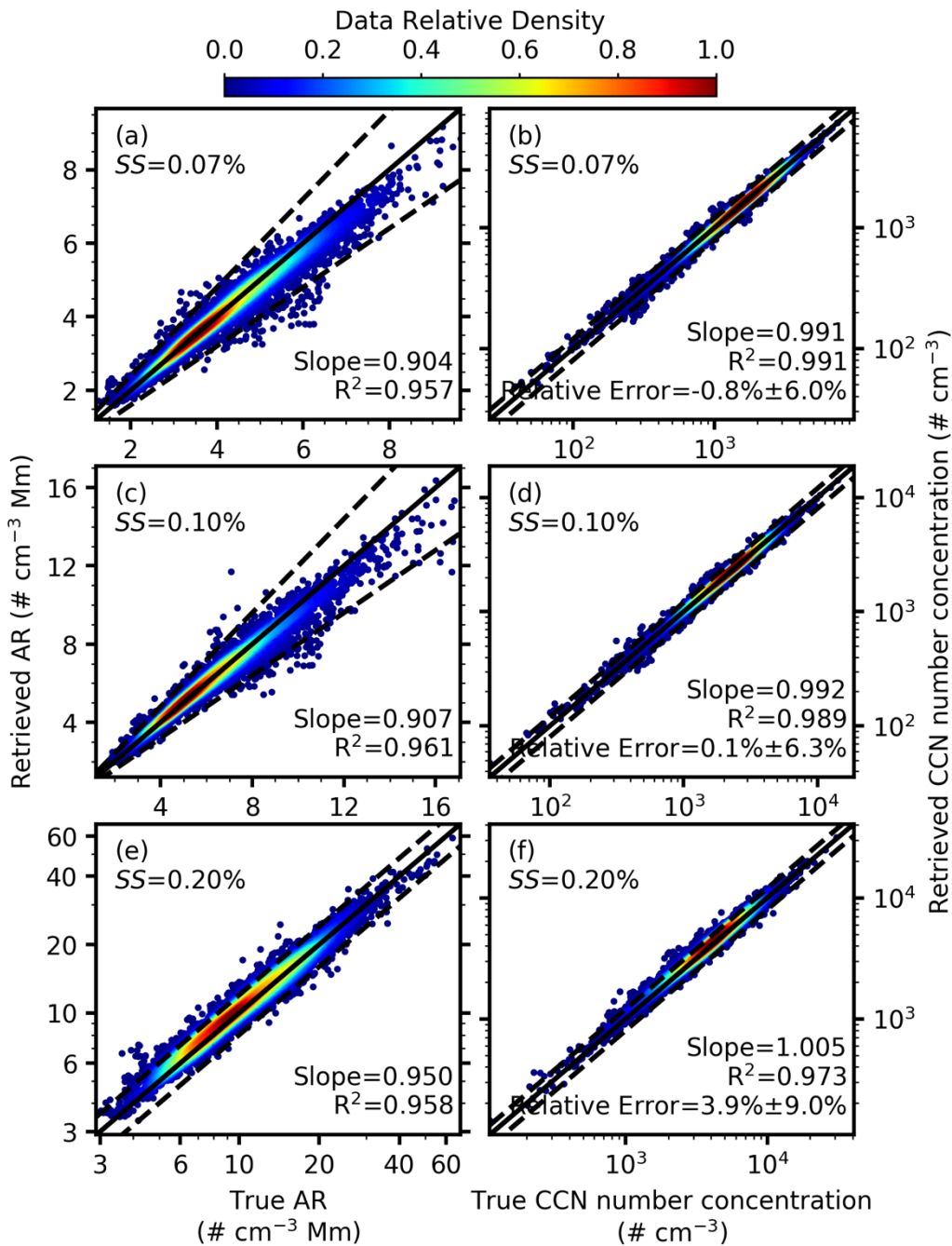
125 Figure R5. Comparison of the theoretical calculated extinction-related CCN activation ratio at 532 126 nm (true AR) and the model predicted extinction-related CCN activation ratios at 532 nm (retrieved 127 AR) at supersaturations of (a) 0.07%, (c) 0.10%, and (e) 0.20%, and of the theoretical calculated 128 CCN number concentrations (true CCN number concentration) and the retrieved CCN number 129 concentrations at supersaturations of (b) 0.07%, (d) 0.10%, and (f) 0.20%. A total of 80575 pairs of 130 data calculated from campaign C5 are used. The solid line is 1:1 line, and the dashed lines are 20% 131 relative difference lines. Colors represent the relative density of the data points normalized by the 132 maximum data density of each panel. The relative error shown in the figure is mean value \pm one 133 standard deviation.
