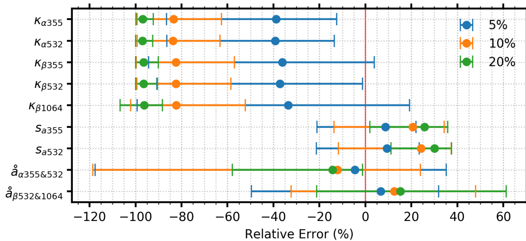
111 Figure R4. Relative errors in fitted and calculated parameters with 10% random errors for 112 backscatter and extinction and 5% (blue), 10% (orange), and 20% (green) random error for relative 113 humidity. The dots are the median values, and the error bars denote the 5th and 95th percentiles. 114 The dashed red line marks the position of zero.
