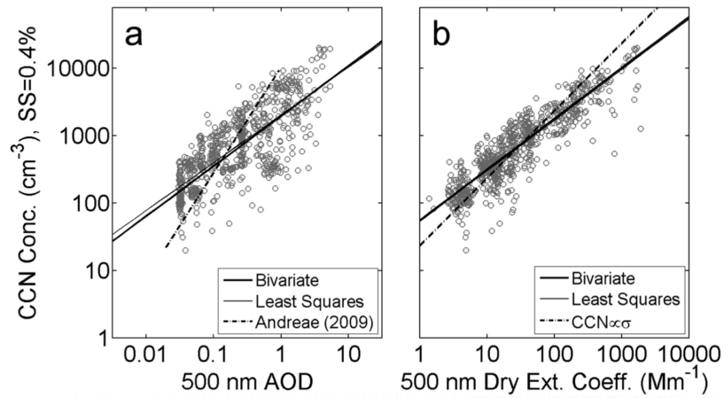
93 Figure R2. Figure 1 in the paper of Shinozuka et al. (2015)
