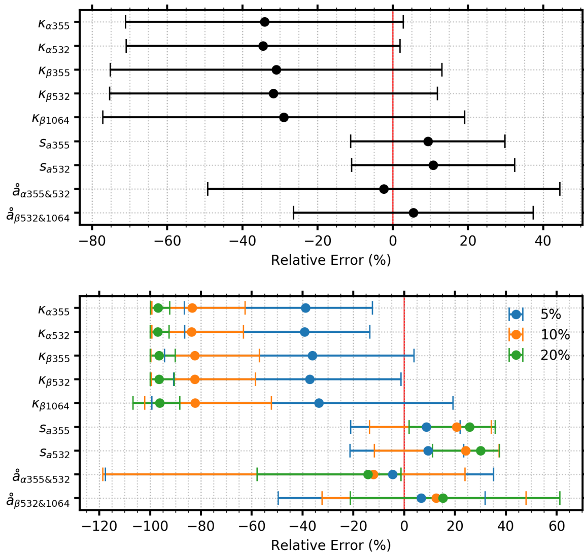
Figure 8. Relative errors in fitted and calculated parameters with 10% random errors for backscatter and extinction and 5% (blue), 10% (orange), and 20% (green) random error for relative humidity. The dots are the mean median values, and the error bars denote the 5th and 95th percentiles standard deviations . The dashed red line marks the position of zero.
