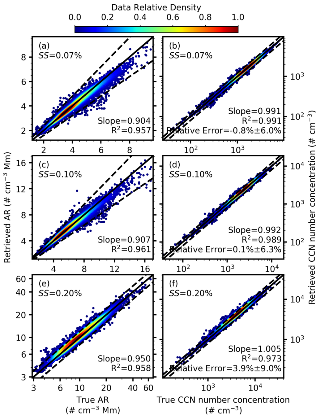
Figure 4. Comparison of the theoretical calculated extinction-related CCN activation ratio at 532 nm ( true AR ) and the model predicted extinction-related CCN activation ratios at 532 nm ( retrieved AR ) at supersaturations of (a) 0.07%, (c) 0.10%, and (e) 0.20%, and of the theoretical calculated CCN number concentrations ( true CCN number concentration ) and the retrieved
