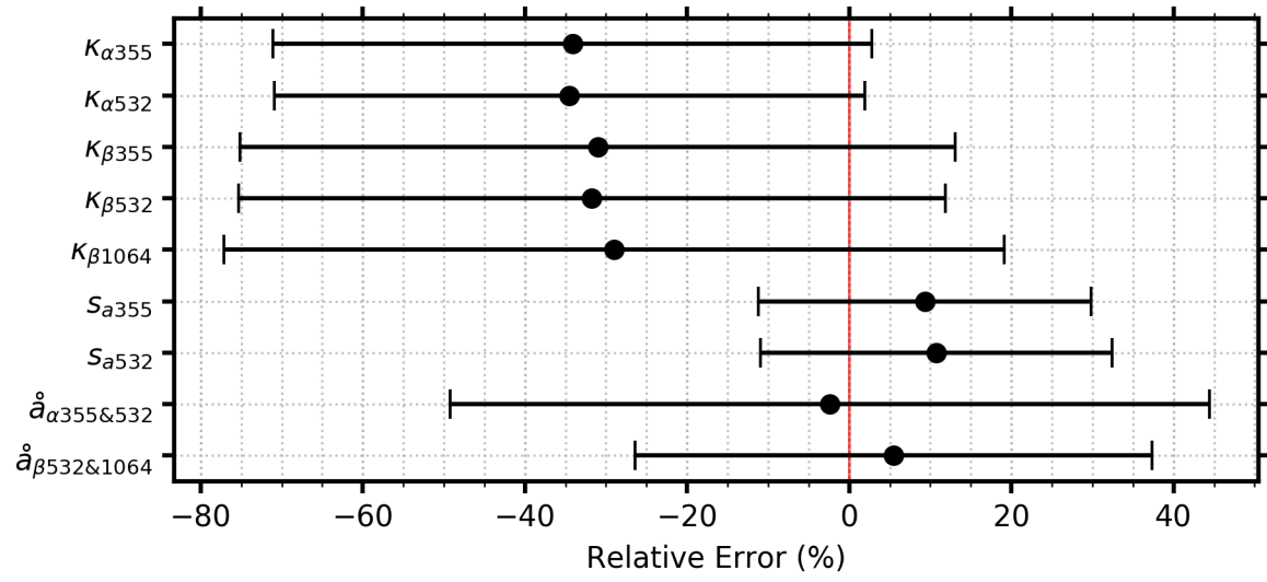
Figure 8. Relative errors in fitted and calculated parameters with 10% random errors for backscatter and extinction and 5% random error for relative humidity. The dots are the mean values, and the error bars denote the standard deviations.
