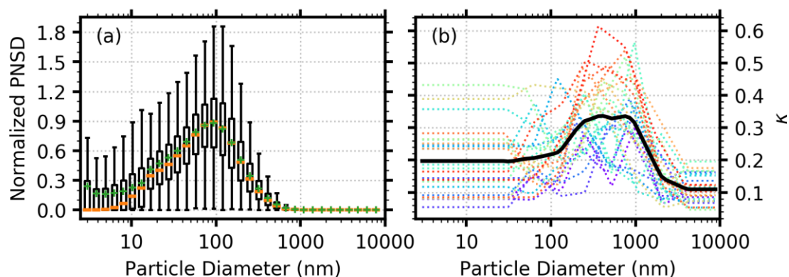
Figure 1. (a) Boxplot of particle number size distributions (PNSDs) in the datasets from five field campaigns. Each PNSD is normalized by its number concentration of total particles. Green markers “+” represent the mean value of each diameter. The boxes extend from the lower to upper quartile values, with orange lines at the median. The whiskers extend from the box to the minimum/maximum values or extend from the box by 1.5 times of interquartile range. The flyers are not shown in the plot. (b) Twenty-five typical size-resolved \kappa distributions. Each dotted line with color represents one size-resolved \kappa distribution. The solid black line represents the mean value of the size-resolved \kappa distributions.
