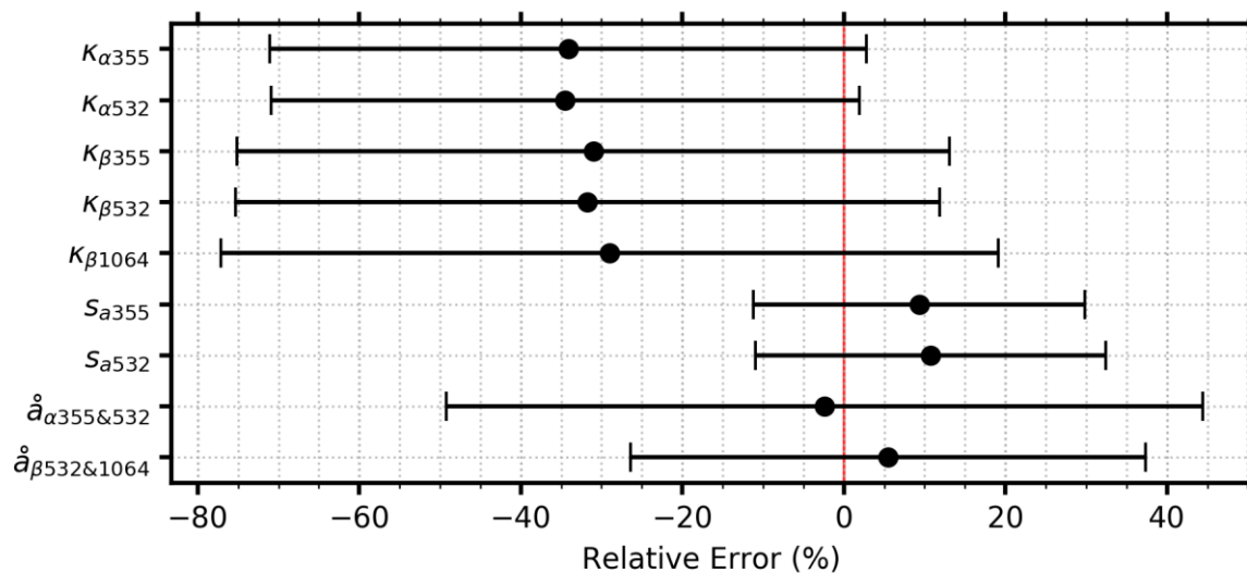
Figure 8. Relative errors in fitted and calculated parameters with 10% random errors for backscatter/extinction and 5% random error for relative humidity. The dots are the mean values, and the error bars denote the standard deviations.
