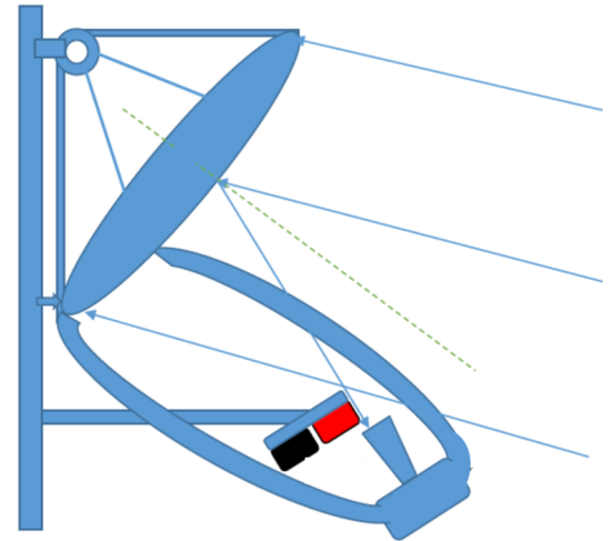
Figure 1. The schematic diagram of TALIS payload. The reflector, feeds, and receivers are formed into a whole. The scan driver controls the scan angle. The calibration system is fixed in the satellite. At the beginning, the feeds are covered by calibration targets. Then it will scan the limb. When the system rotates to the top, it will view the cold space.
