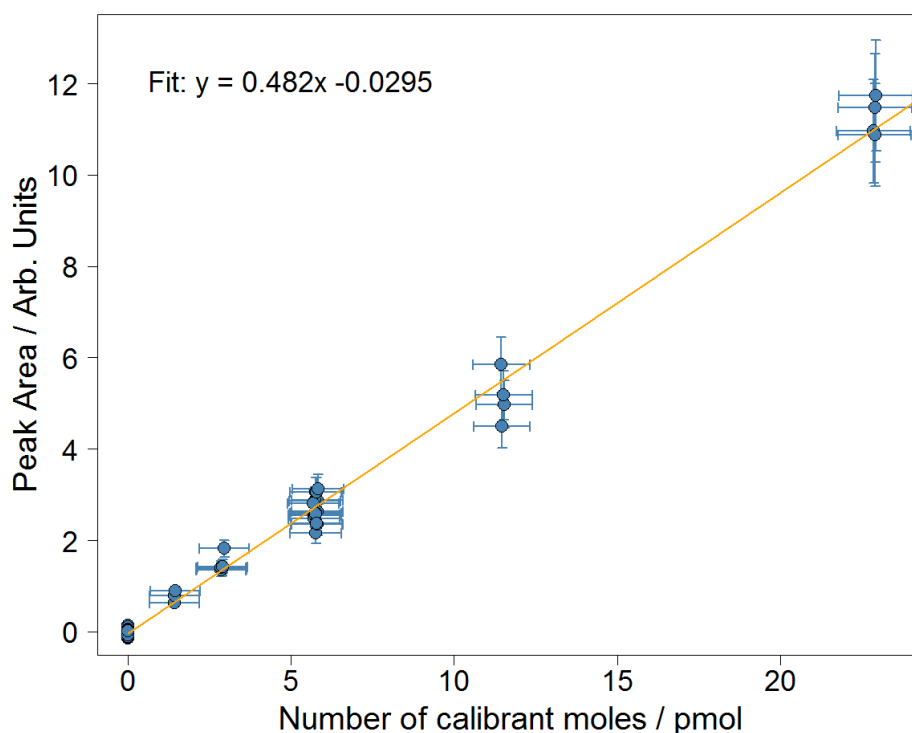
Figure 7: Calibration plot for isoprene for the week of 02-08/07/2018 from the Wytham field campaign. Error bars in the area correspond to the precision of the measurement ( \pm 10.4\% ). Error bars in the calibrant moles are estimated from the uncertainties in the secondary standard used and in the volume of gas sampled.
