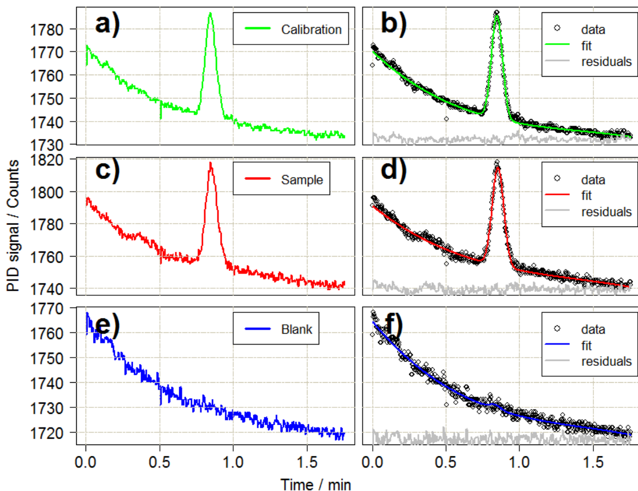
Figure 3: Typical chromatograms for a) calibration, c) sample, and e) blank runs. The isoprene peak detected by the PID is around the 0.8 min mark. Panels b), d) and f) show the combined baseline and Gaussian fits to the observed data for each run type. Residuals are offset for clarity. All the chromatograms are from the deployment in Wytham Woods (see Section 5.3). The calibration run is for 12 mL of a 11.6 ppb standard of isoprene in a nitrogen balance. The sample run is for a 150 mL ambient air sample (later quantified as 1.5 ppb isoprene). The blank run is for a 12 mL sample of Grade 5.0 nitrogen.
