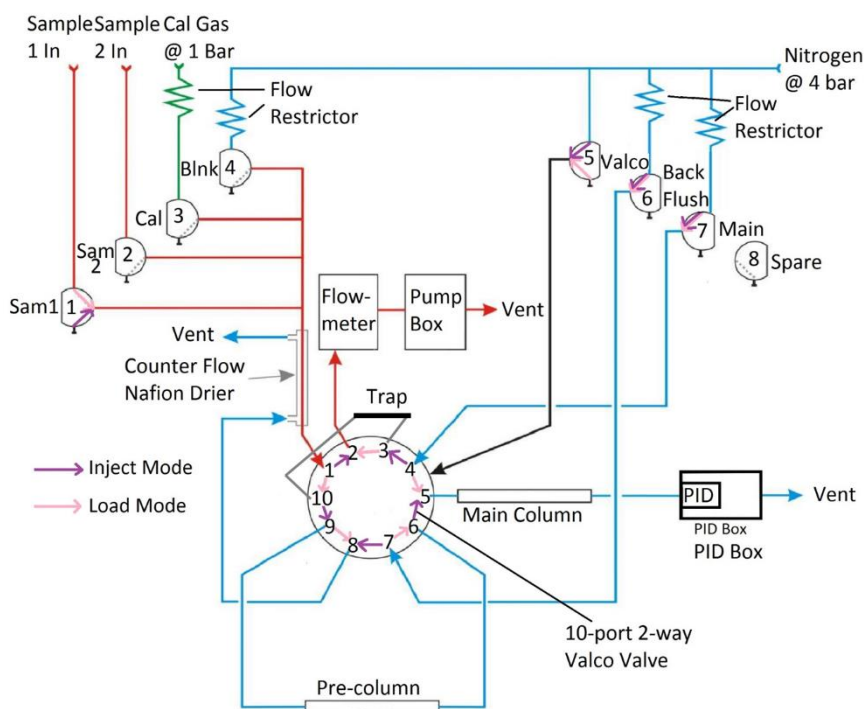
Figure 2: Schematic representation of the iDirac operation. When in Load Mode (valve 5 off - pink), the contents of a gas source chosen between valves 1-4 are pre-concentrated on the adsorbent trap. In Inject Mode (valve 5 on - purple), the VOCs in the trap are injected into the dual-column system for separation and, eventually, detection.
