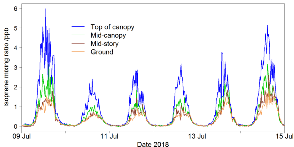
Figure 15: Portion of the isoprene mixing ratio time series measured at Wytham Woods (UK) at four heights within a forest canopy in the summer of 2018.
