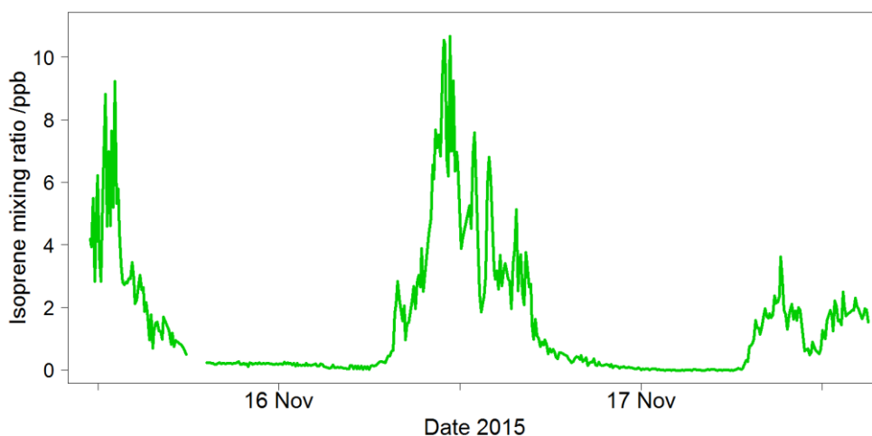
Figure 14: Time series for isoprene at secondary forest site in Sabah (Malaysian Borneo) in 2015
