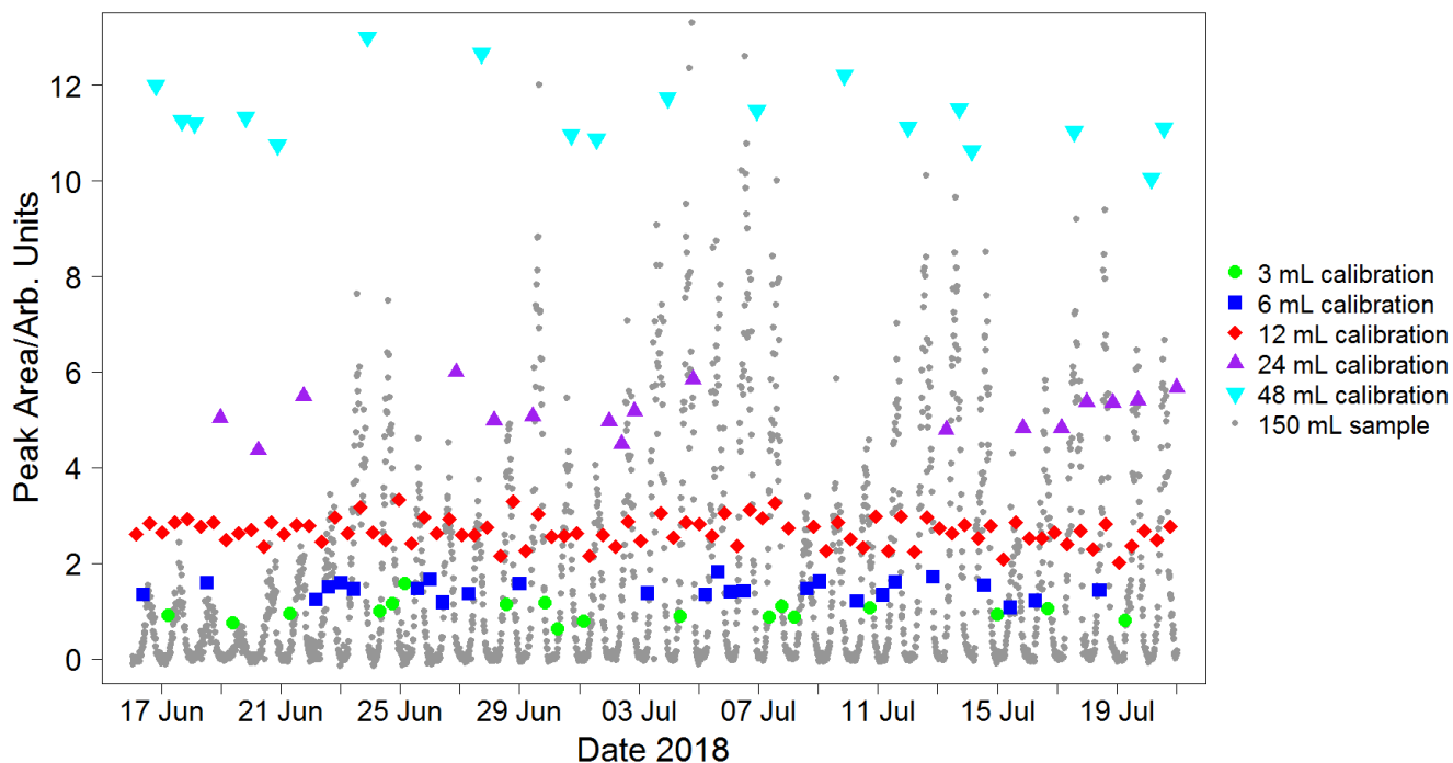
Figure 6: Typical sequence of isoprene peak areas for runs with varying calibration volumes. These, once split into weekly segments, are used to produce a calibration curve (see Figure 7). The calibration runs with the standard user-specified sampled volume (red data points) are used to calculate the instrument precision on a weekly basis (see Section 4.2). Peak areas from sample runs (grey data points) are also shown to illustrate how the calibration peak areas span the entire range of sample values, minimising the need for extrapolation. This plot was produced using data from the Wytham field campaign (see Section 5.2).
