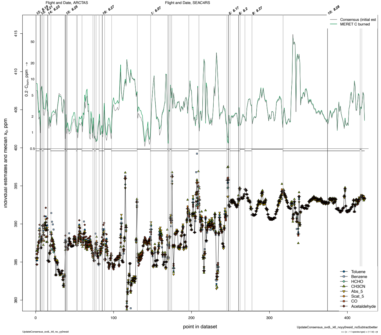
Figure 8. (Lower panel). Estimates of the 422 background \hat{x}_i^0 = \text{CO}_2 + \text{CO} concentrations implied based on the 8 fire tracers indicated in the legend. Contributing individual estimates \hat{x}_{ij}^0 are shown by overlapping colored points, with the median estimate \hat{x}_i^0 indicated by a black bar. Usually the colored points overlap closely, this indicates strong agreement (Upper panel) Estimates of C_{\text{burn}} = x_i - \hat{x}_i^0 indicators of fuel carbon burned, in the heavy green line. The preliminary estimate of C_{\text{burn}} based on the consensus of tracer deviations (without variable EnR estimates) is also shown in a light line. A scale factor, maximizing overlap with the heavy line, was necessarily estimated by regression. Flight days are indicated by the days marked on the top axes, and individual plumes, separated by non-plume concentrations of longer than 10 minutes, are shown as vertical separator lines. A set of horizontal lines at \sim 400 ppm indicates selected intervals for optimizing numerics (see text, Section 6.3, item 7).
