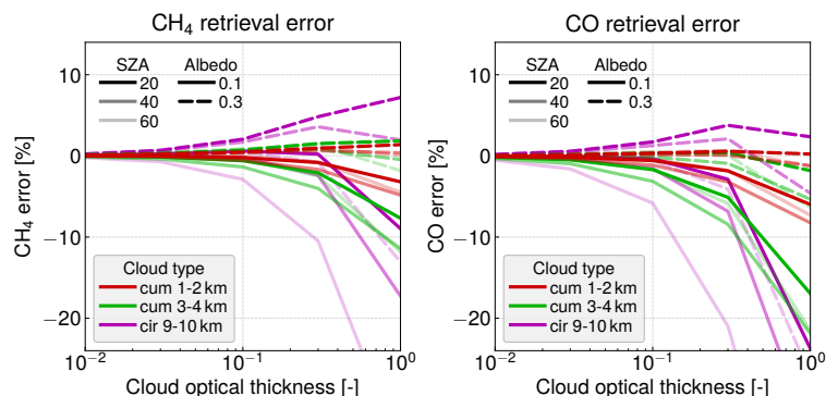
Figure 5. Systematic retrieval errors for different water and ice clouds under various conditions.
