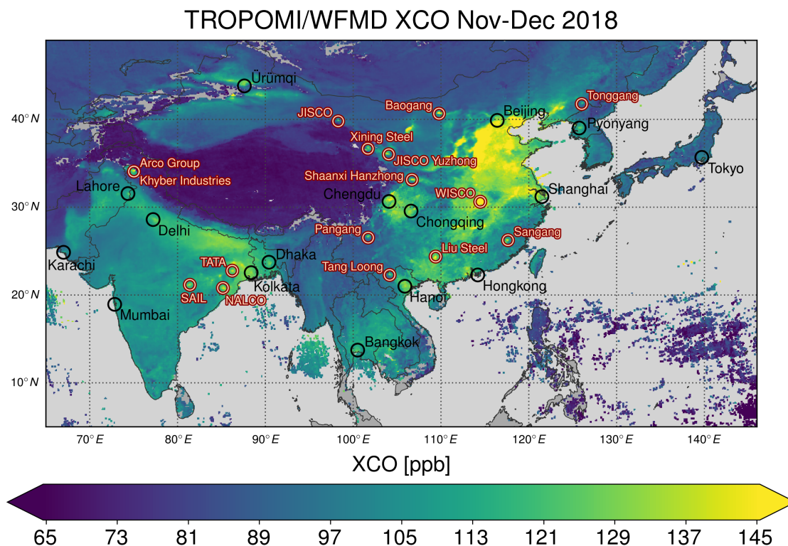
Figure 18. Carbon monoxide distribution for November and December 2018 over China, India, and Southeast Asia highlighting emissions of congested urban areas and industrial facilities.
