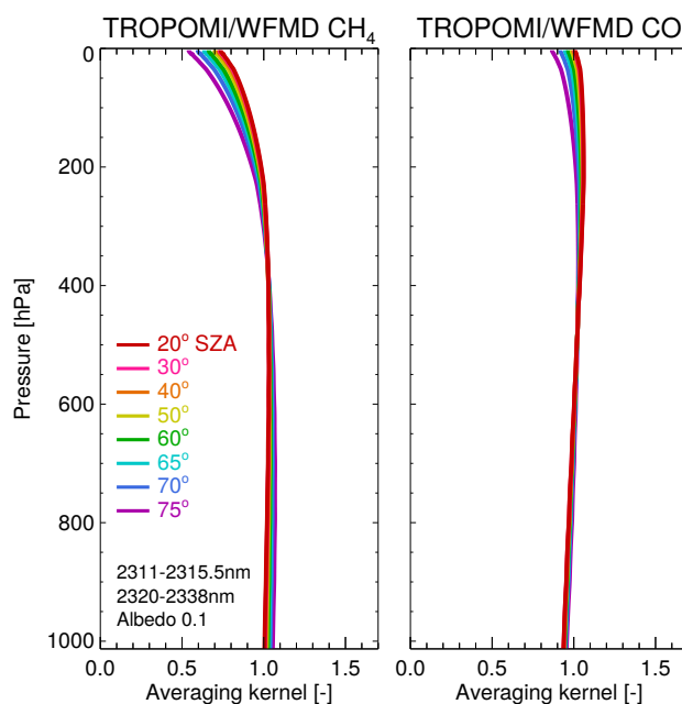
Figure 2. CH 4 and CO column averaging kernels reflecting the altitude sensitivity of the retrievals.
