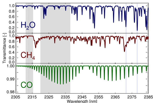
Figure 1. Fitting windows (grey) and trace gas transmittances for the SWIR bands of TROPOMI for U.S. Standard atmosphere concentrations. The strong H 2 O absorption lines between 2370 and 2380 nm used to obtain cloud information are shown in light blue. The apparent albedo is retrieved in the continuum at 2313 nm (dashed line).
