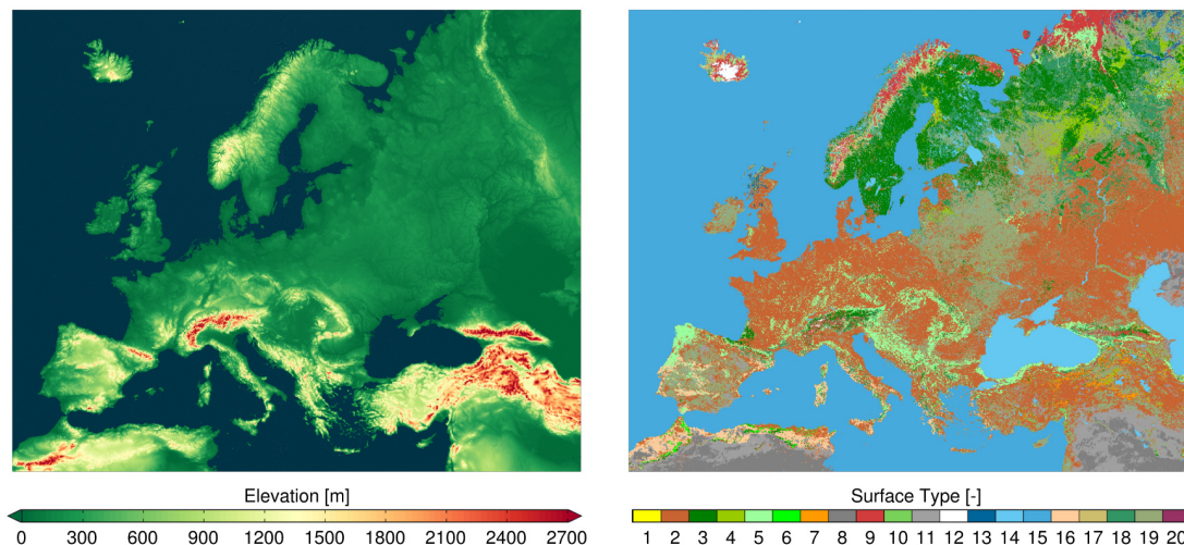
Figure 6. USGS GMTED2010 elevation and GLCC surface type (Biosphere Atmosphere Transfer Scheme Legend) with 0.05^\circ resolution using the example of Europe. In the GMTED2010 data set, ocean areas have been assigned a value of 0 (shown in dark blue).
