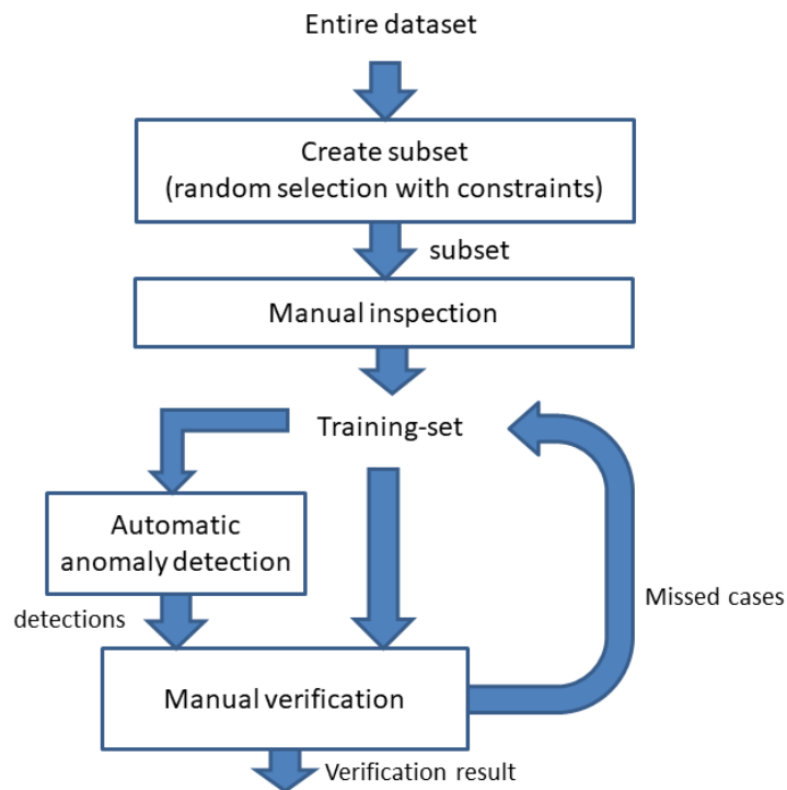
Fig. 1. Update Figure 1 (Training set issue)
