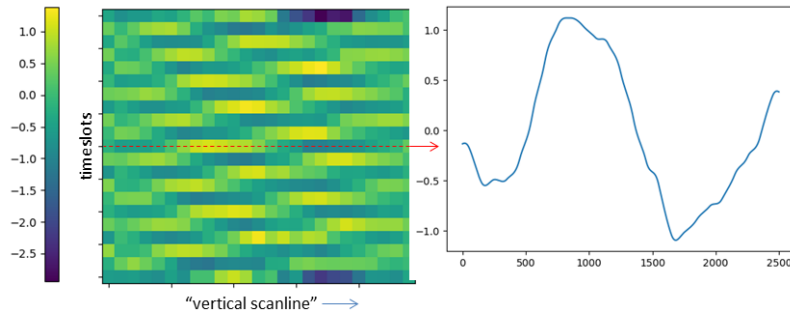
Figure 10. Example of the Meteosat 5 optical hardware issue in time, where the left image shows the anomaly's bias for consecutive images across the scanlines. The right image is for a particular timeslot and shows the anomaly's bias across the scanlines. Taken from METEOSAT5-MVIRI-MTP10-NA-NA-19960515120000 and channel IR.
