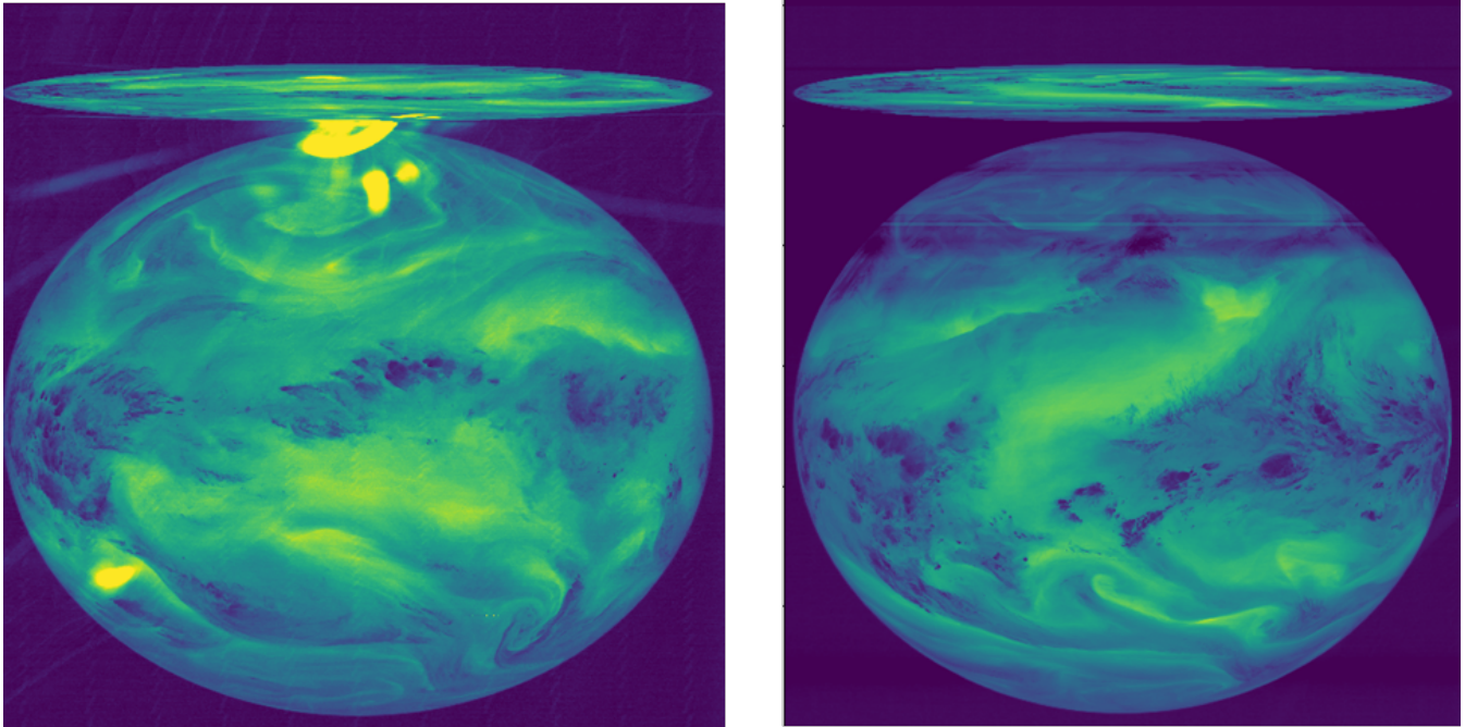
Figure 4. Left: image affected by a stray light anomaly (file: METEOSAT4-MVIRI-MTP10-NA-NA-19900415003000, channel: WV). Right: several hours later, still showing follow-on effects after the stray light anomaly (file: METEOSAT5-MVIRI-MTP10-NA-NA-20060317213000, channel: WV). The pixels values are the raw digital counts, see also Figure 2.
