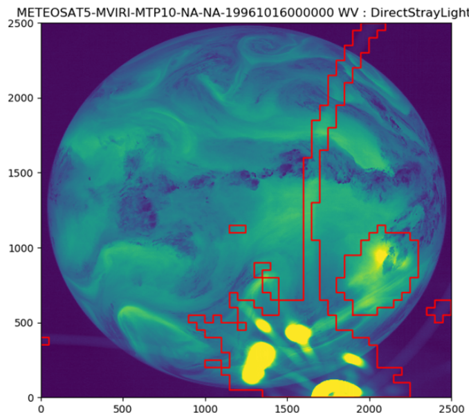
Figure 9. Segmentation result of the direct straylight anomaly detection. Taken from METEOSAT5-MVIRI-MTP10-NA-NA19961016000000 and channel WV. The pixels values are the raw digital counts, see also Figure 2.
