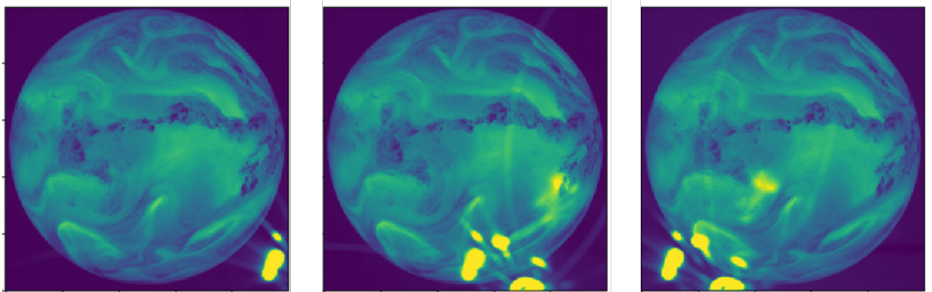
Figure 8. Three sequential images affected by the direct straylight anomaly. Left: Taken from file METEOSAT5-MVIRI-MTP10-NA-NA19961015300000 and channel WV. Center: Taken from file METEOSAT5-MVIRI-MTP10-NA-NA19961016000000 and channel WV. Right: Taken from file METEOSAT5-MVIRI-MTP10-NA-NA19961016300000 and channel WV. The pixels values are the raw digital counts, see also Figure 2.
