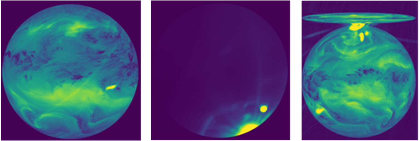
Figure 7. Three examples of the direct straylight effect anomaly. Left: Taken from file METEOSAT7-MVIRI-MTP15-NA-NA-20130717210000 and channel WV. Center: Taken from file METEOSAT7-MVIRI-MTP15-NA-NA-19991016003000 and channel VIS. Right: Taken from file METEOSAT4-MVIRI-MTP10-NA-NA-19900415003000 and channel WV. The pixels values are the raw digital counts, see also Figure 2.
