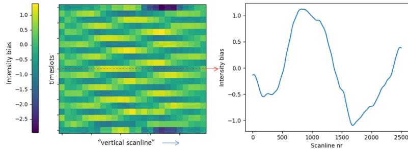
Figure 10. Example of the Meteosat 5 optical hardware issue in time, where the left image shows the anomaly's bias for consecutive images across the scanlines. The right image is for a particular timeslot and shows the anomaly's bias across the scanlines. Taken from METEOSAT5-MVIRI-MTP10-NA-NA-19960515120000 and channel IR.
