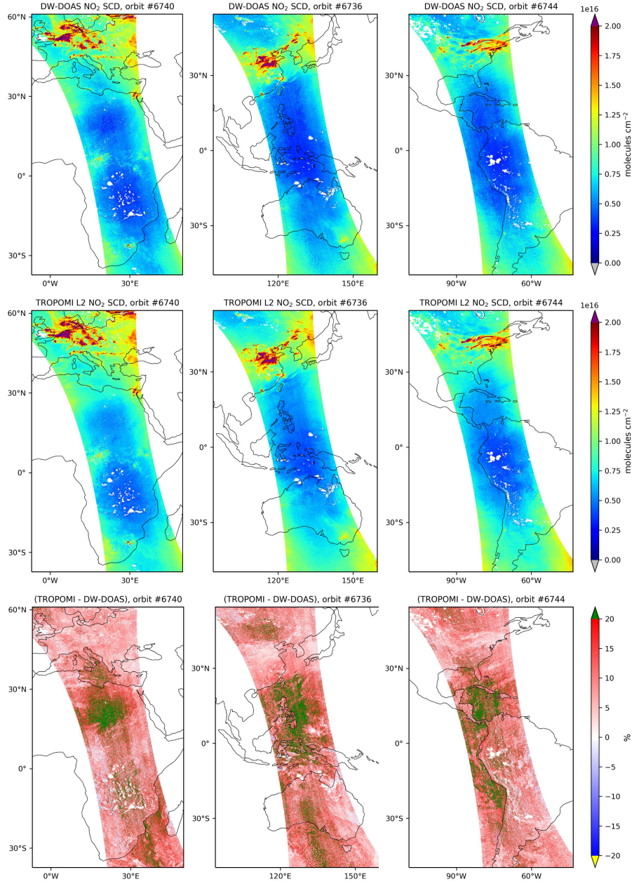
Figure 7. (top) NO 2 SCDs retrieved by DW-DOAS for selected orbits of 31/01/2019, (middle) corresponding TROPOMI NO 2 SCDs, and (bottom) the relative differences between them calculated as (TROPOMI - DW-DOAS)/TROPOMI and expressed in %. All the data are screened using the QA flag ( qa > 0.5 ) from the TROPOMI NO 2 level 2 dataset, which includes all-sky pixels.
