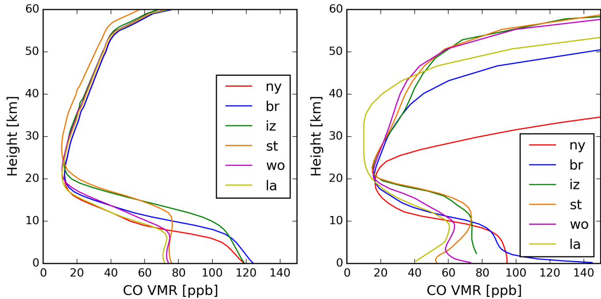
Figure 3. The CO a priori VMR profiles for TCCON (left) and NDACC (right) at six sites (ny: Ny-Ålesund; br: Bremen; iz: Izaña; st: St Denis; wo: Wollongong; la: Lauder). As TCCON a priori profiles change every day, the mean profiles in 2013 are shown here.
