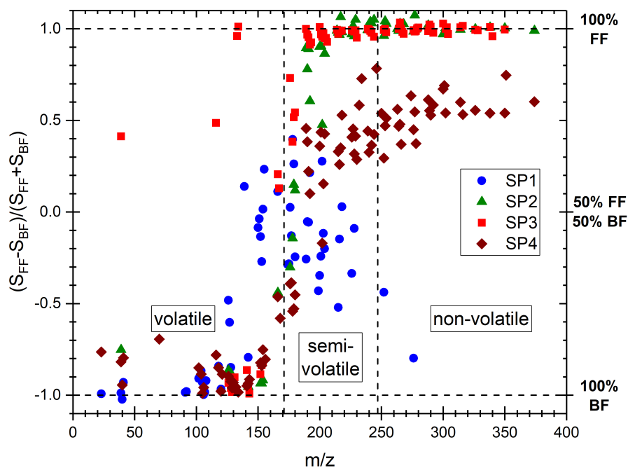
Fig. 1. “Contrast plot” representing the variation in PAH signal detected with L2MS at \lambda_i = 266 nm for the 4 CAST set points.
