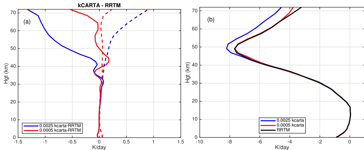
Figure 5. Heating rates for the 630-1180 \text{cm}^{-1} region computed using low ( 0.0025 \text{ cm}^{-1} ; blue curves) and high ( 0.0005 \text{ cm}^{-1} ; red curves) resolution kCARTA databases for 49 spanning Earth atmosphere profiles, compared to RRTM-LW. (a) The left panel shows differences in the heating rates, while (b) the right panel shows the mean heating rates.
