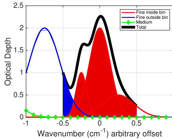
Figure 1. Line-by-line calculations from UMBC-LBL. The bin of interest is at (-0.5, +0.5) \text{ cm}^{-1} . Lineshapes whose line centers are within this bin (red) and within \pm 1 \text{ cm}^{-1} of the bin edge (blue) are computed using high spectral resolution; line centers that are further out (green) have the lineshapes computed at medium resolution and then interpolated to a higher resolution; line centers even further away (not shown) are computed at coarse resolution. The black curve is the sum over all the line contributions within that bin.
