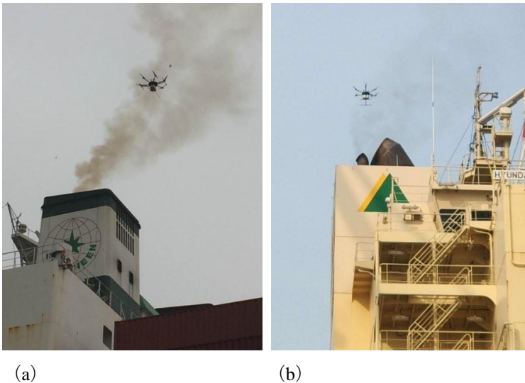
Figure 4. Photographs showing the flight of the UAV during measurements. The UAV platform was flown close to the funnel of ship for collecting exhaust gas and detection at Waigaoqiao pier.
