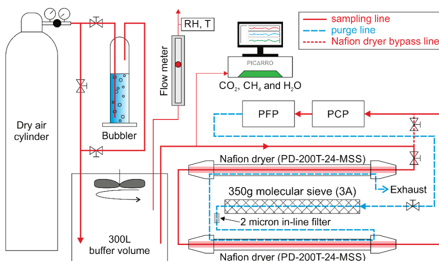
Figure 5. Schematic of the setup used at INSTAAR to determine the effect of the Nafion Air Dryer on the mole fraction determination of \text{CO} , \text{CH}_4 , \text{N}_2\text{O} and \text{SF}_6 along with \text{CO}_2 and its singly-substituted isotopologues. Dry sample from a calibrated cylinder was flushed into a buffer volume either directly or through a bubbler to humidify it up to \sim 1.4\% water vapour by volume at an average temperature of 23^\circ\text{C} . A NOAA-ESRL PCP-PFP system could be flushed with either dry or humidified cylinder air including or by-passing the NAD. Flow from the cylinder was adjusted such that there was always an overflow of air from the buffer volume, where relative humidity of the sample was constantly monitored. A Picarro analyser was used to monitor the stability of \text{CO}_2 , \text{CH}_4 and \text{H}_2\text{O} mole fractions in the gas exiting the buffer volume, during all the tested experimental conditions, a summary of which is shown in Figure 6.
