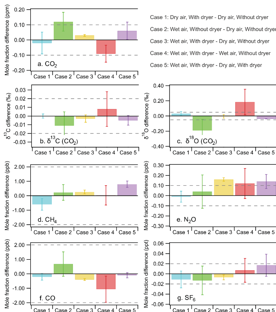
Figure 6. Overview of results to determine the effect of the NAD on the mole fraction determination of \text{CO} , \text{CH}_4 , \text{N}_2\text{O} and \text{SF}_6 along with \text{CO}_2 and isotopic composition of its two singly-substituted isotopologues ( ^{16}\text{O}^{13}\text{C}^{16}\text{O} and ^{16}\text{O}^{12}\text{C}^{18}\text{O} ). The dashed lines denote the WMO network compatibility goals for the different species. We note that the compatibility goal for \text{N}_2\text{O} should be seen as a lower limit target value. We present 5 test cases to illustrate the measurement biases introduced if samples are not sufficiently dried. Case 1 shows the effect of the NAD in dry conditions, whereas cases 3 and 5 show the difference in sampling of wet sample air dried with the NAD before being compressed into the sample flask with respect to dry air sampling. The worst sampling conditions with the largest bias are associated with using humidified sample air (without NAD) shown in cases 2 and 4. When the difference remain within the WMO network compatibility goals, we concluded that the measured difference is not significant (notably for cases 1, 3 and 5 for most species).
