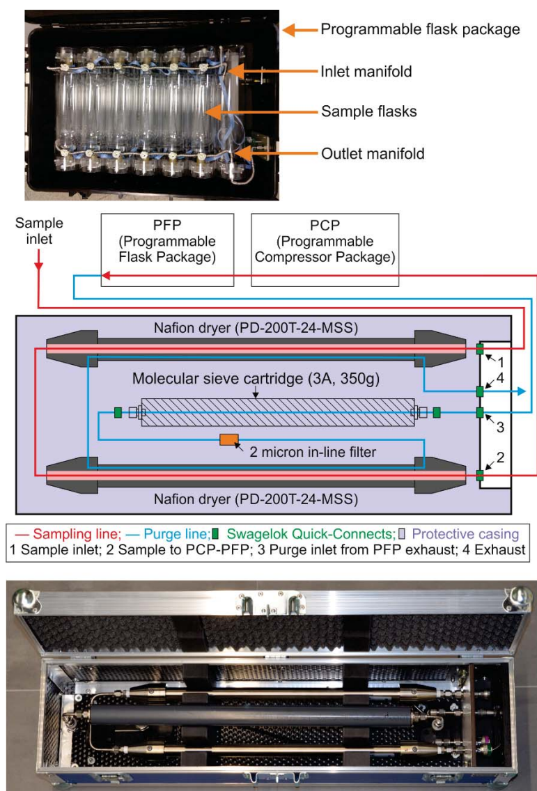
Figure 1: Top: A programmable flask package showing the flasks and the inlet/outlet manifolds. Middle: A schematic showing the Nafion dryer system, which is housed inside a custom-built box, and the sampling or purge lines. The Nafion dryer system comprises of two Nafion dryers (Perma Pure PD-200T-24-MSS), a molecular sieve cartridge, a 2 micron in-line filter, and various Swagelok connectors and tubing. Ambient air first passes through the two pre-conditioned Nafion dryers connected in series (red line), drying the incoming air. It then goes through the PCP, which pushes the sample through the PFP. The exhaust of the PFP is connected to the molecular sieve cartridge in the NAD which removes any residual moisture
