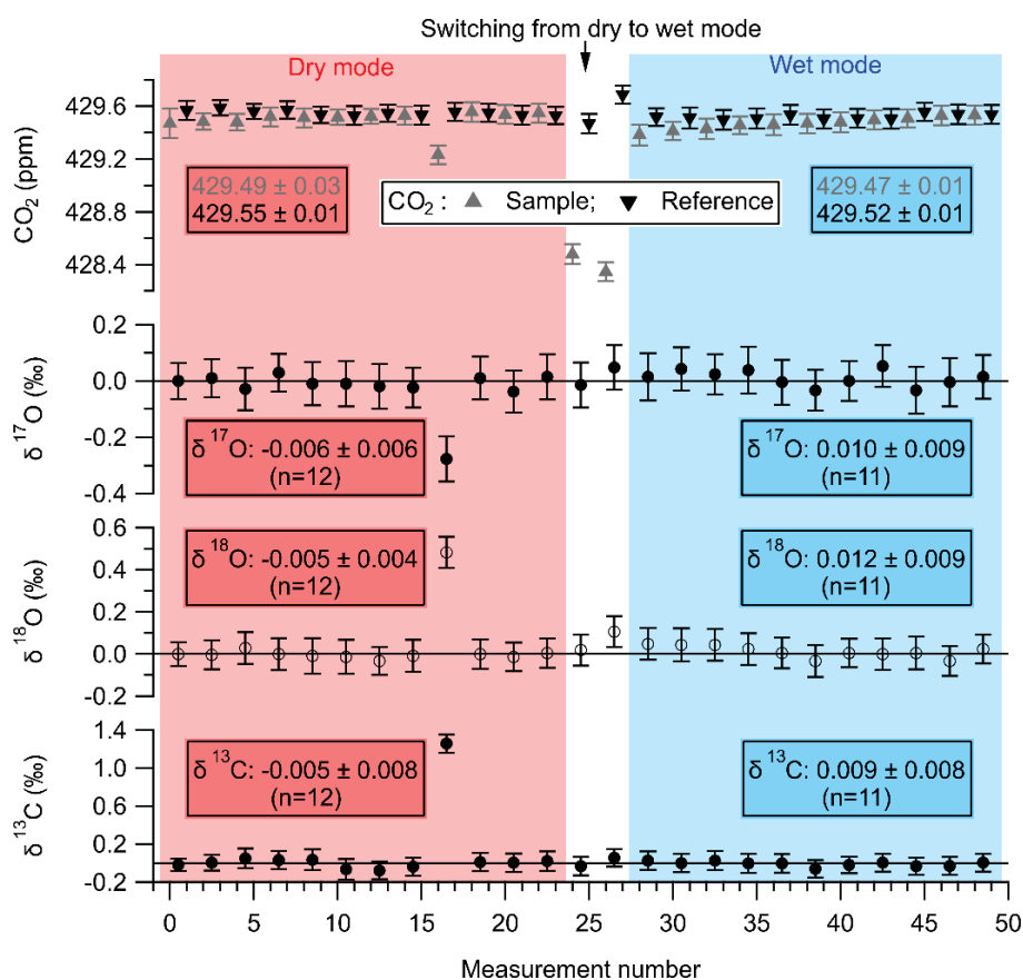
Figure 4. A zero-enrichment experiment performed with the TILDAS-SICAS to test the effect of the NAD on the CO 2 mole fraction and the stable isotopes of CO 2 . The top panel shows the CO 2 mole fraction, where the grey triangles represent the sample measurements and the black inverted triangles represent the reference measurements. The other three panels show the isotopic composition of the sample gas determined with respect to the reference gas. The reference gas is identical to the sample gas, the only difference being that the sample gas was measured after it had passed through the NAD. The first part of the experiment represents dry mode (shown in red background) where, for sample measurements, dry air from a cylinder was passed through a preconditioned NAD and was then introduced into the TILDAS-SICAS for measurements. In the latter
