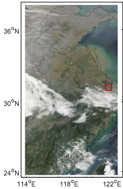
Fig. S2. MODIS Terra true color map composed by 1, 4, and 3 channels on October 18, 2014 ( https://worldview.earthdata.nasa.gov/ ). The red rectangle box (40*40km) is the MODIS AOD average window in Baoshan pyranometers site.
