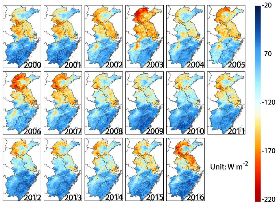
Figure 6: (a) Annual Yearly mean ADRF distributions during 2000-2016 over East China (unit: \text{W m}^{-2} ). (b) The changes of annual regional mean ADRF during 2000-2016 over East China.
