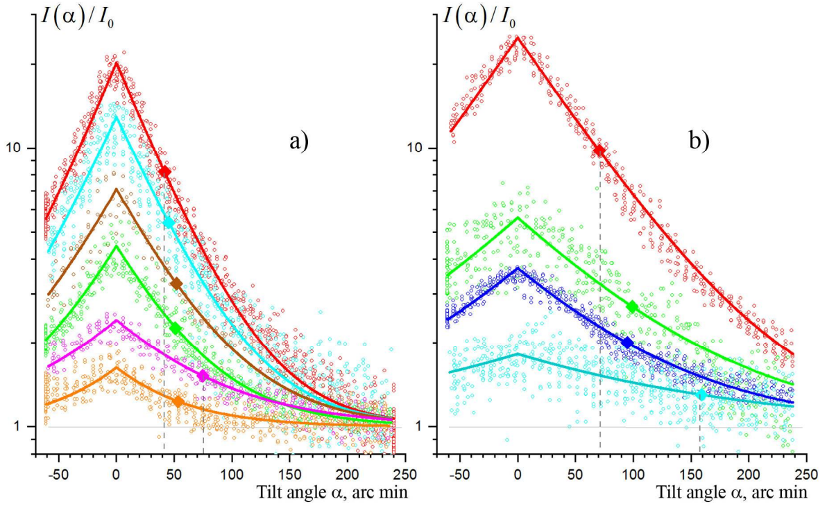
Figure 11. Selected cases of observed distributions I_{co}^{Circ} . For all curves the values of intensity are normalized to the values I_0 , obtained by fitting according to the Eq. (1). Squares indicate the tilt angles, corresponding to the distribution width w . The left frame shows cases of a fairly narrow distribution, w is within 40-75 arc minutes. The ratio I(4^\circ)/I_0 is less then 1.1. The right frame shows cases with I(4^\circ)/I_0 > 1.1 , among these cases there are distributions with a large (up to 159 arc min) width.
