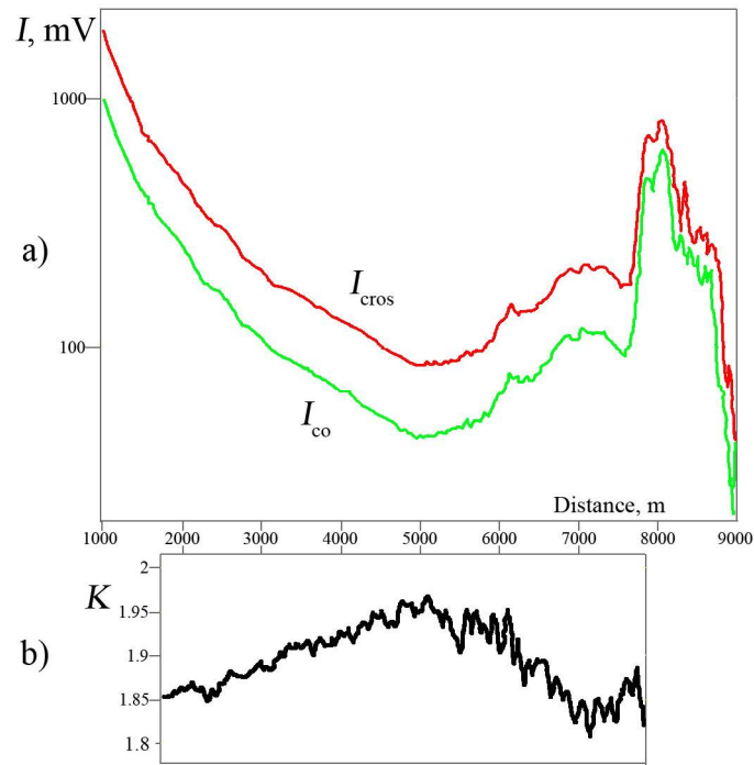
Figure 6. Channel calibration procedure. (a) The record of a signal (1064 nm) integrated by the plate rotation angle, components I_{co} (green) and I_{cros} (red). Integration was carried out during four revolutions of the plate. (b) the value of calibration constant K , calculated in the height range of 1800-8000 m. The mean value K=1.91 .
