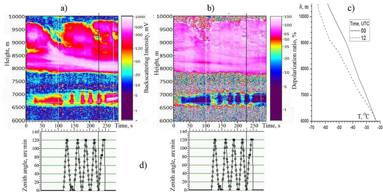
Figure 7. Lidar data on 6 April 2018, 10:25 LST (UTC+7) for the initial circular polarization. (a) Intensity of I_{co}^{Circ} component; (b) depolarization ratio \delta^{Circ} = I_{cros}^{Circ} / I_{co}^{Circ} ; (c) weather sounding data (Novosibirsk station, 07:00 and 19:00 LST); (d) zenith tilt angle (arc min), time axis is aligned with 7a and 7b.
