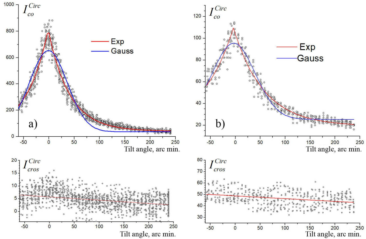
Figure 10. Typical angular dependences of the intensity of polarization components, 2 June 2018. Top frames – co-polarized components I_{co}^{Circ} , bottom frames – I_{cros}^{Circ} . (a) 12:00 LST, averaging over the layer from 11470m to 11600m. (b) 10:00 LST, the layer 10980-11270 m. The record (a) shows low depolarization ratio and narrow ( w=42 arc min.) distribution. The record (b) has a wider distribution ( w=82 arc min.) and large depolarization
