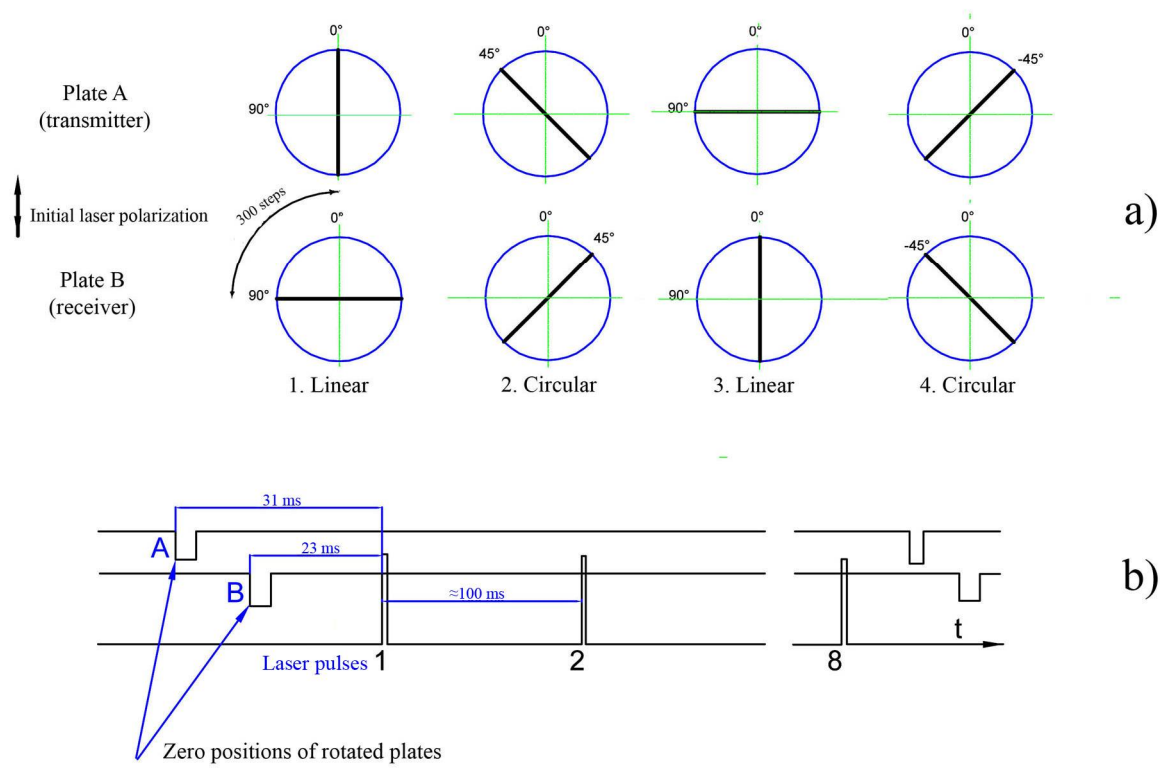
Figure 4. (a) Diagram of the rotation of the phase plates. Plate mounting angles for the four consecutive laser pulses are shown. The bold line shows the direction of a fast axis of the plates. (b) The time position of the laser pulses relative to the zero positions of the plates. The situation repeats every 8 pulses.
