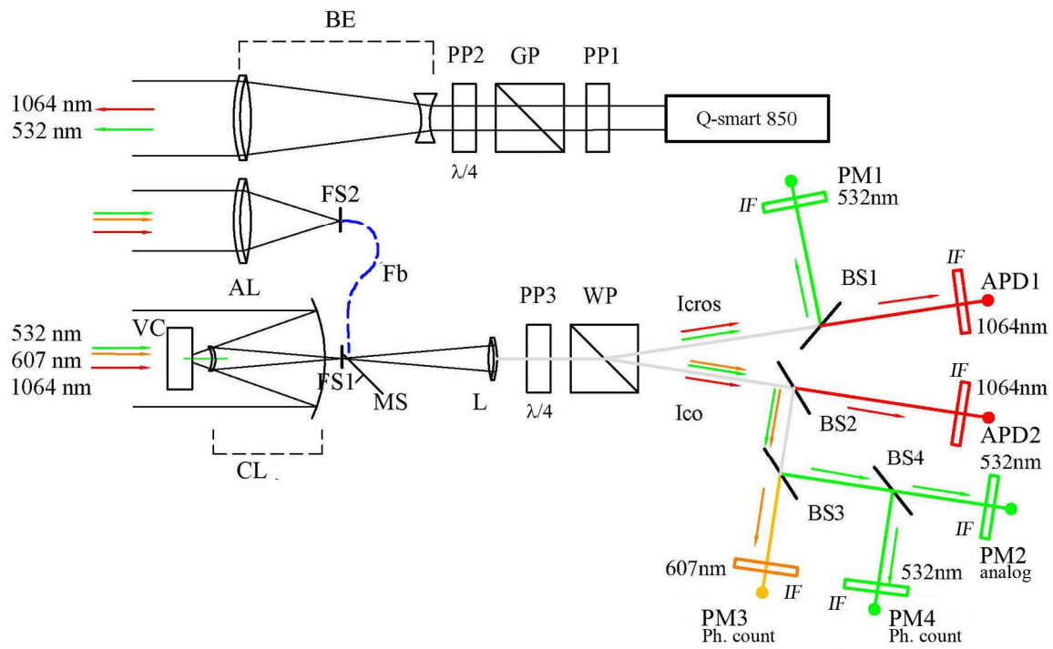
Figure 2. Optical circuit of the LOSA-M3 lidar
