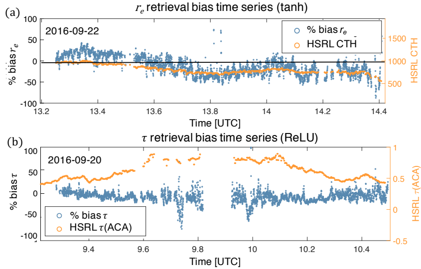
Figure 8. Panel (a) is a time series of the percent bias of r_e(\text{NN}) with respect to r_e(\text{PP}) plotted along with the accompanying HSRL-2 CTH time series overtop. The solid line going through the center of the figure indicates both zero bias and the CTH assumption of 1 km. Panel (b) shows the time series of the percent bias of \tau(\text{NN}) with respect to \tau(\text{PP}) plotted along with the accompanying HSRL-2 \tau_{\text{ACA}} . Note that these biases are shown for datasets on different days.
