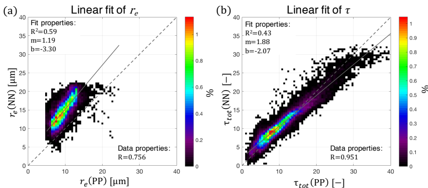
Figure 4. Density regression plots demonstrating behavior of raw NN retrieval output for r_e ( \tanh network) and \tau ( \text{ReLU} network). The dashed gray line in each plot indicate the 1:1 line, while the solid gray line indicates the linear best fit line for the dataset.
