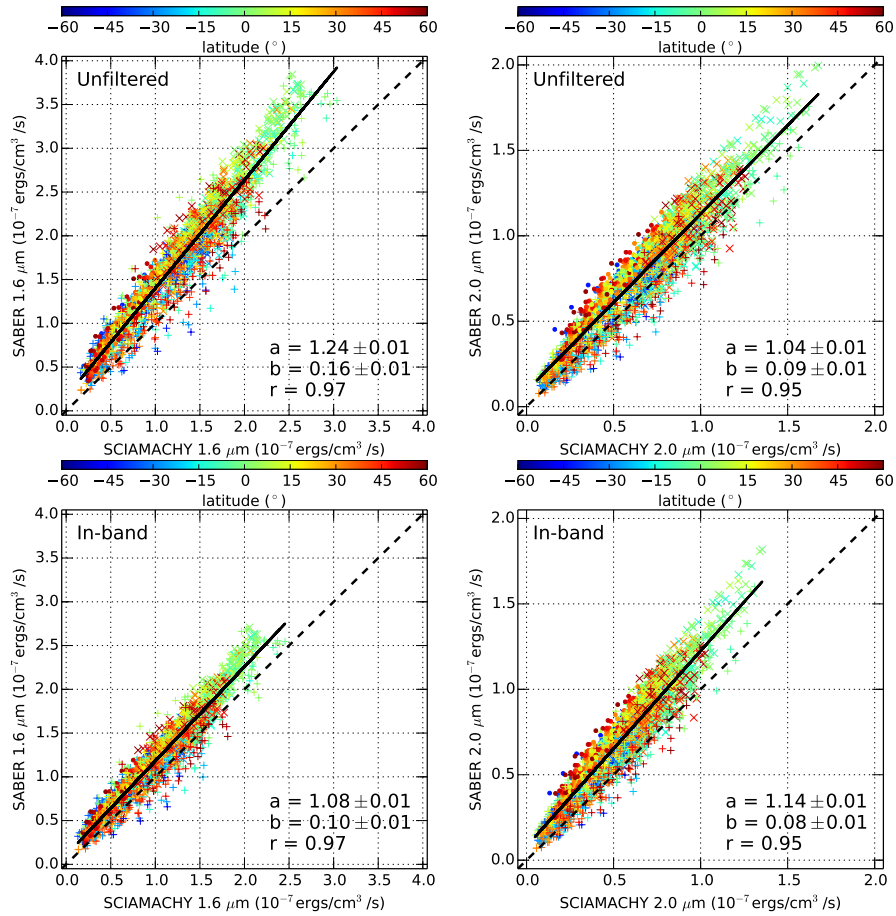
Figure 6. Scatter plots of SABER 1.6 μm (left) and 2.0 μm (right) volume emission rates versus the corresponding simulations using SCIAMACHY data for the year 2007. The color bar shows the latitude. The plus marker indicates the data at 80-85 km, the x marker represents the data at 86-90 km, and the point marker shows the data at 91-95 km. The solid line shows the linear fit to the data. a and b represent the slope and y-intercept of the fitting line, respectively. r represents the correlation coefficient of the fitting.
