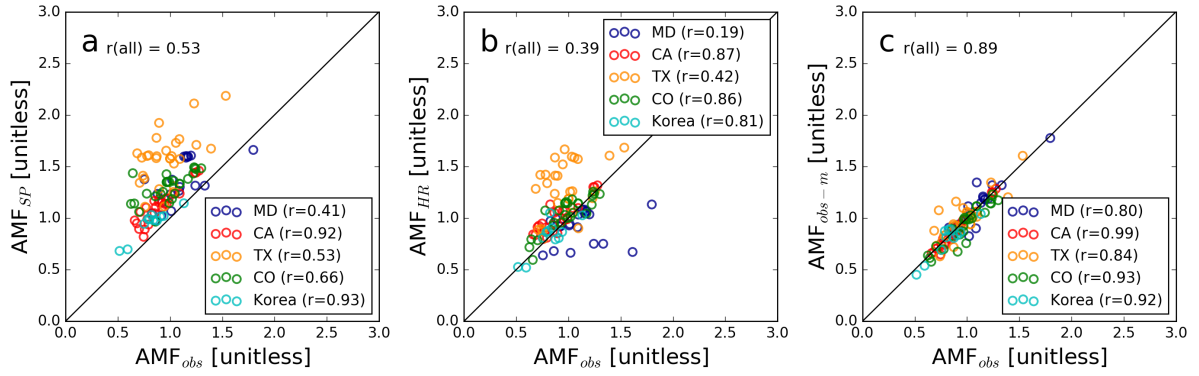
Figure 3. Comparison of AMFs calculated using observed NO_2 profiles ( AMF_{obs} ) with tropospheric AMFs in the OMI standard product ( AMF_{SP} , 3a), and those calculated using NO_2 profiles from high-resolution model simulations ( AMF_{HR} , 3b). The right panel (3c) compares tropospheric AMFs using daily versus campaign-average profiles ( AMF_{obs-m} ). The symbols are color-coded by campaign locations.
