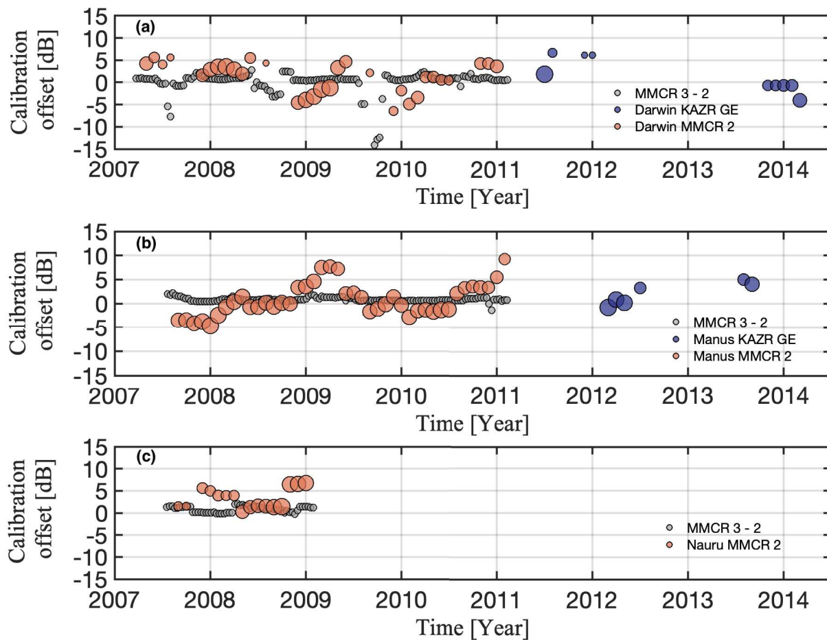
Figure 9: The calibration offset for the MMCR mode 2 and KAZR GE mode at the Tropical Western Pacific (TWP) sites of (a) Darwin, (b) Manus and (c) Nauru based on the ARM – CloudSat comparison. The size of the circles indicates the ratio of the sample size of the CloudSat columns for any given calibration offset estimate relative to the maximum sample size of CloudSat columns observed during the same period by the same mode. The gray circles indicate the ARM mode 3-mode 2 difference as estimated from the ARM radar mode intercomparison.
