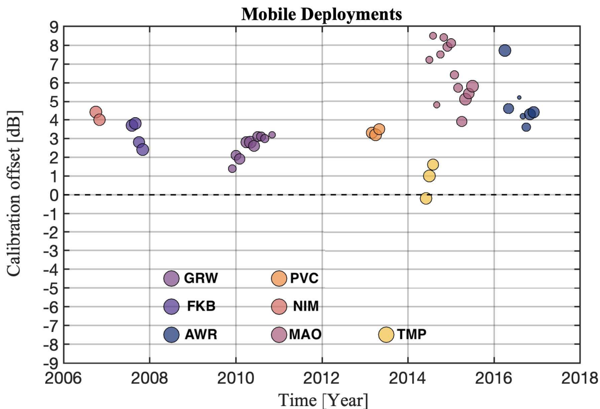
Figure 11: The radar calibration offset we should add to the reported ARM cloud radar reflectivities in order to minimize their differences with those reported by the CloudSat CPR at the ARM Mobile Facilities (AMF) sites. The size of the circles indicates the ratio of the sample size of the CloudSat columns for any given calibration offset estimate relative to the maximum sample size of CloudSat columns observed during the same period by the same mode.
