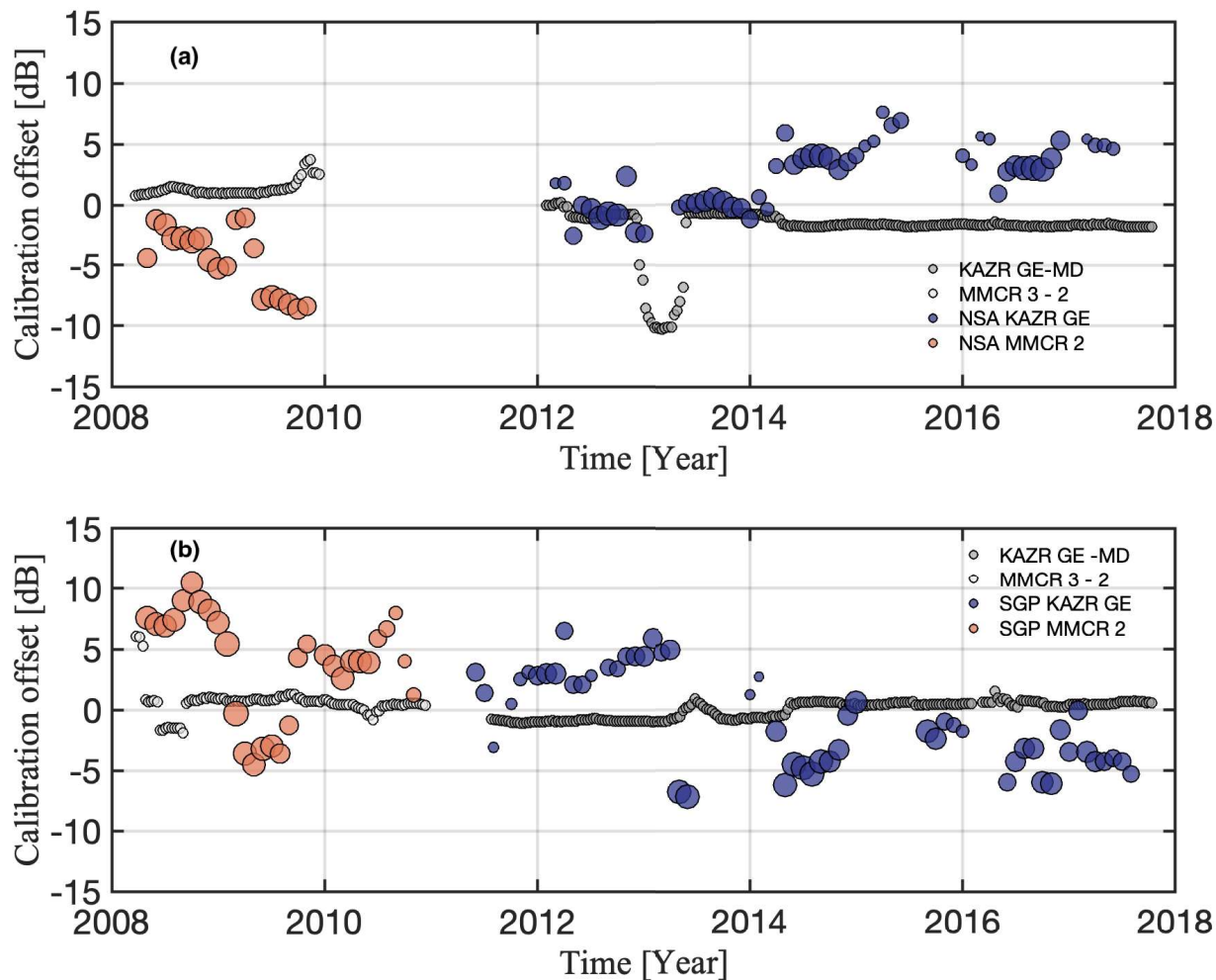
Figure 10: The calibration offset for the MMCR mode 2 and KAZR GE mode at (a) NSA and (b) SGP sites based on the ARM – CloudSat comparison. The size of the circles indicates the ratio of the sample size of the CloudSat columns for any given calibration offset estimate relative to the maximum sample size of CloudSat columns observed during the same period by the same mode. The gray circles indicate the ARM MMCR mode 3 -mode 2 and KAZR GE -MD mode difference as estimated from the ARM radar mode intercomparison.
