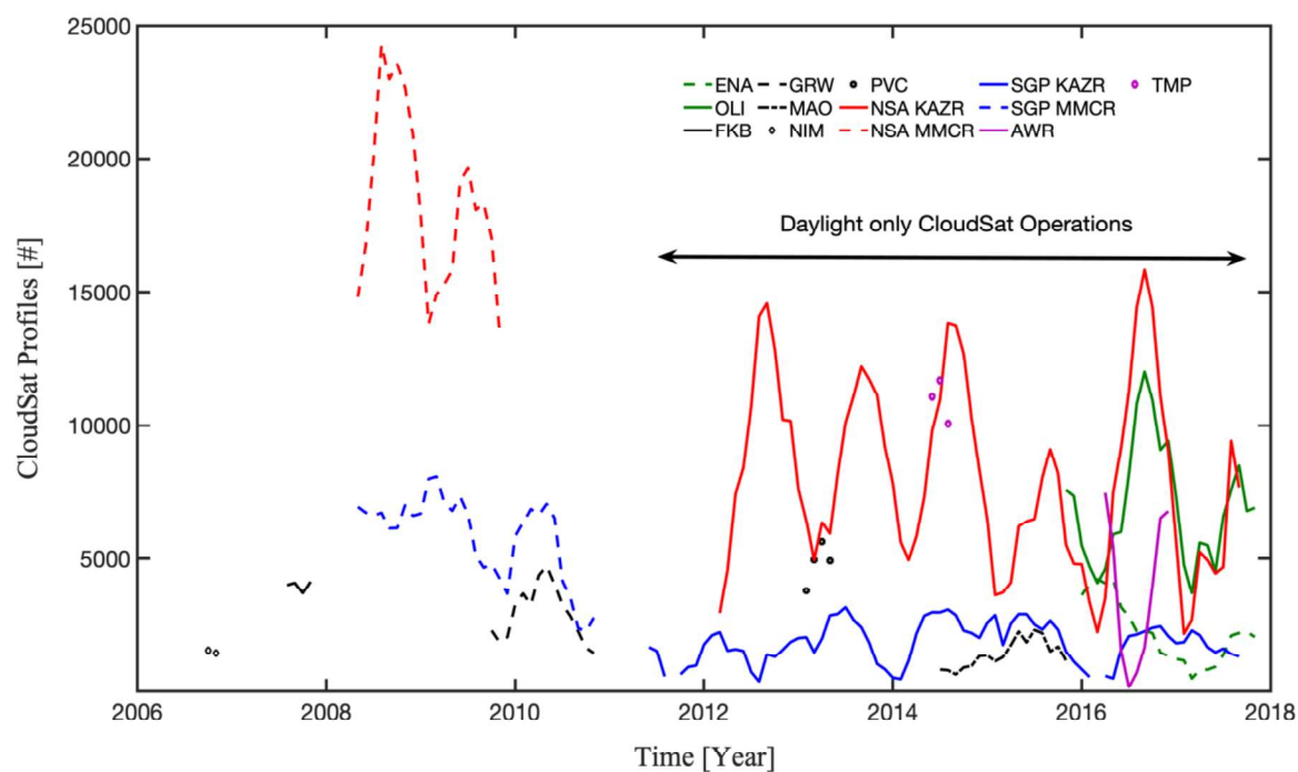
Figure 5: The number of CloudSat profiles found within a \pm 3 month window to be suitable for calibrating the ARM cloud radars as a function of time for the different ARM sites.
