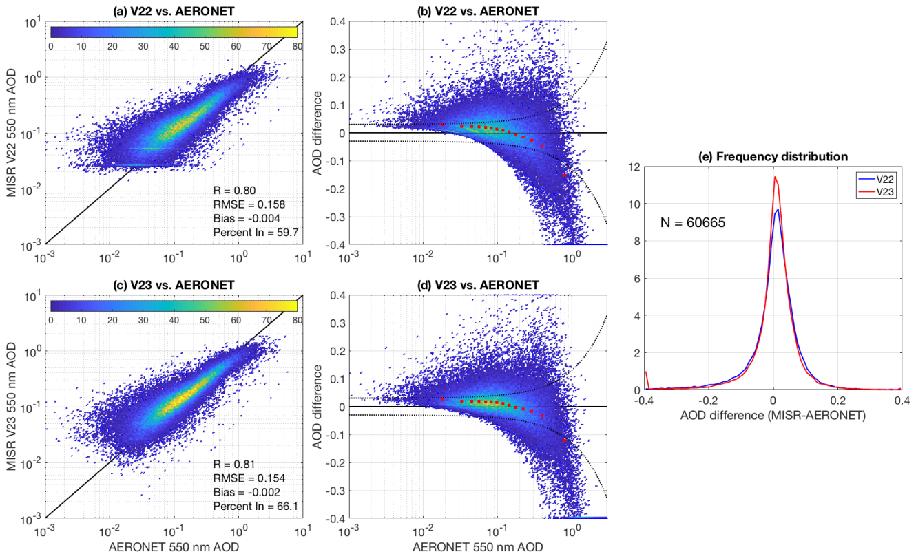
15 Figure 15 MISR V22 and V23 retrieval comparisons against AERONET observations. (a) Density plot of MISR V22/AERONET collocations including overall statistics; (b) density plot of AOD difference (MISR V22-AERONET) as a function of AERONET AOD; points outside of the y-axis limits are grouped on edges; red squares denote the median values for data split into 14 equally populated bins; the black dotted lines mark the EE of \pm(0.03+10\%) ; (c) similar to (a) but for MISR V23/AERONET collocations; (d) similar to (b) but for MISR V23 retrievals; (e) histograms of the MISR-AERONET AOD difference for V22 (blue line) and V23 (red line) retrievals. The number of joint V22/V23/AERONET collocations is 60,665.
