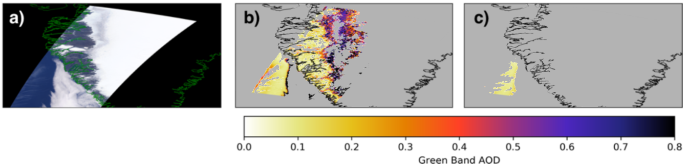
5 Figure 2 MISR V23 aerosol retrievals over Greenland for 15 August 2017 (Orbit 93932, Path 006). (a) MISR An camera RGB; (b) map of unscreened Aerosol_Optical_Depth_Raw retrievals; (c) map of screened Aerosol_Optical_Depth retrievals showing geographic exclusion over land as well as filtering of lower quality retrievals over the water.
