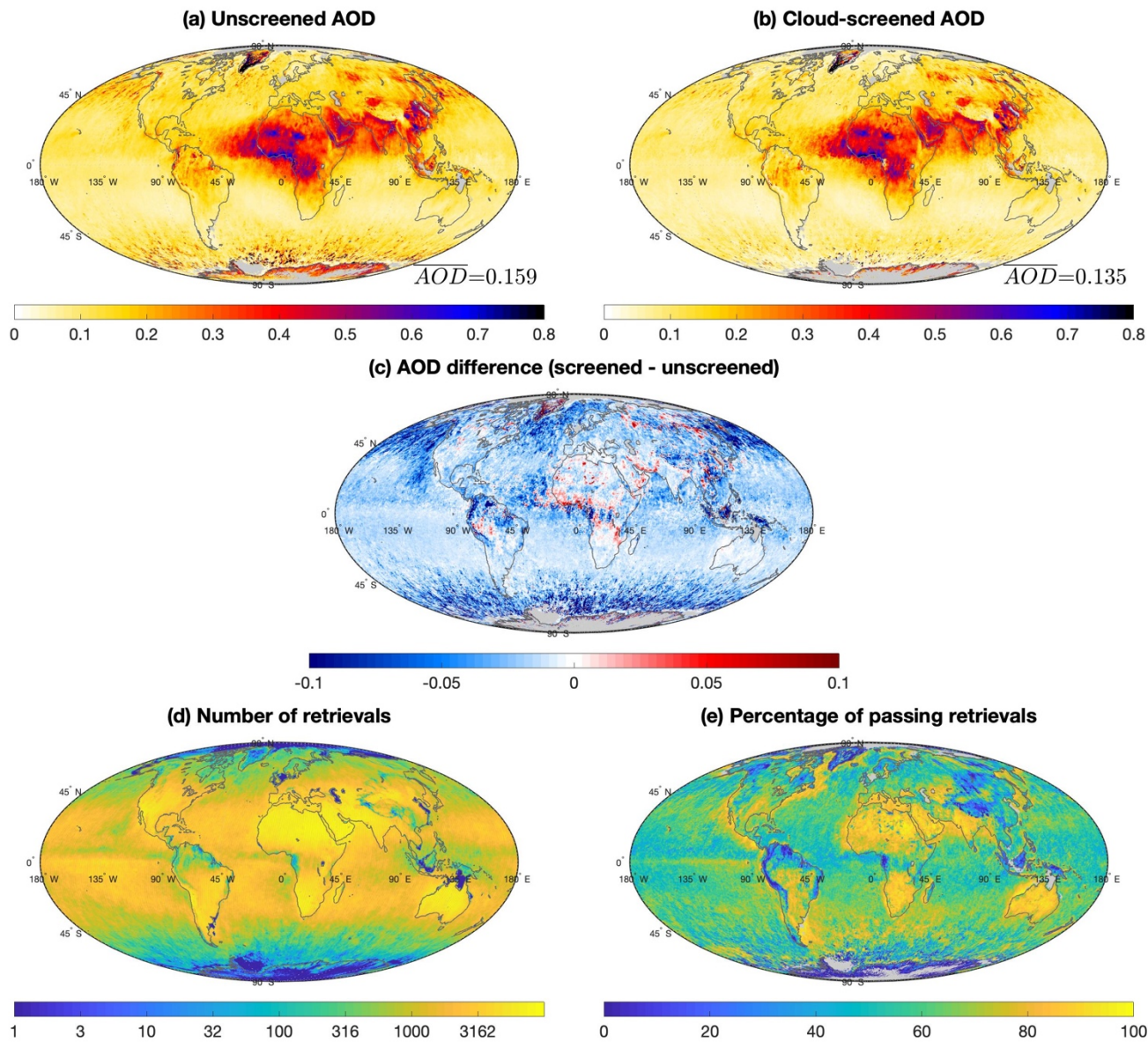
5 Figure 1 Effects of additional cloud screening implemented operationally in V23 shown using 0.5-degree gridded retrievals from 2012. (a) global AOD distribution prior to additional cloud screening; (b) global AOD distribution with operational cloud screening; (c) AOD difference between the screened and unscreened data; (d) number of retrievals (unscreened) in each grid box; (e) percentage of retrievals remaining after cloud screening. Average AOD values in (a) and (b) are area-weighted.
