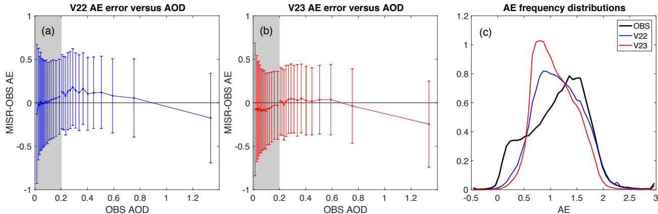
20 Figure 17 V22 and V23 AE comparisons against AERONET+MAN observations (OBS). (a) AE difference (MISR V22 – OBS) as a function of OBS AOD; data are split into two AOD regimes, OBS AOD \leq 0.2 and OBS AOD > 0.2 , and divided into 15 equally populated bins within each of the AOD regimes. The shaded area marks the smaller AOD regime. The markers represent the median AE difference values within each AOD bin and the error bars are one standard deviation of AE difference within each bin. (b) Same as (a) but for MISR V23 – OBS AE difference. (c) Normalized frequency distributions of AE obtained from the three collocated data sets. The total number of analyzed collocations is 61,015; 17,027 of collocations have OBS AOD > 0.2 .
