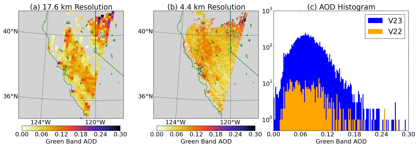
5 Figure 5 Comparison of V22 and V3 AOD retrievals for 5 July 2016 (orbit 88022). (a) V22 AOD map; (b) V3 AOD map; (c) AOD histograms.
