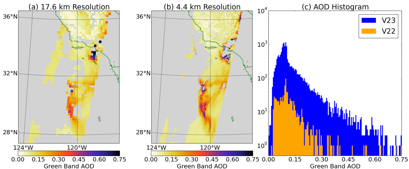
Figure 4 Comparison of V22 and V3 AOD retrievals for 23 July 2016 (orbit 88284). (a) V22 AOD map; (b) V3 AOD map; (c) AOD histograms.
