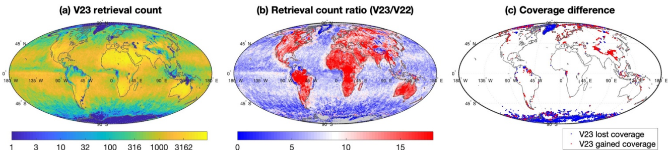
Figure 6 (a) Number of MISR V23 retrievals from 2012, gridded at 0.5-degree resolution, the color scale in decimal logarithm. (b) Ratio between the number of V23 retrievals and V22 retrievals; the average ratio, represented by white color in the color scale, is \sim 9.0 . (c) Locations of grid points where V23 loses (blue) or gains (red) coverage in comparison to V22.
