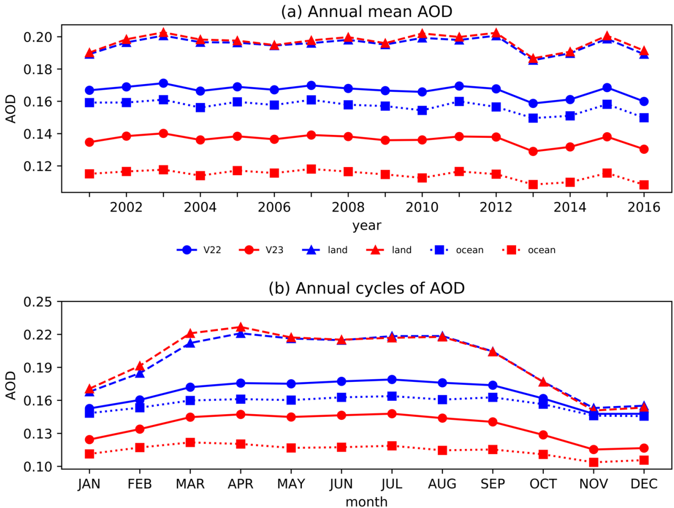
5 Figure 3 (a) Time series of area-weighted annual mean AODs from V22 (blue) and V23 (red) between 2001 and 2016. Solid lines with circles, triangles with dashed lines, and squares with dotted lines represent global mean AOD, AOD averaged over land, and AOD averaged over ocean respectively. (b) Annual cycles of AOD. AOD for each month is averaged for the 16 years.
