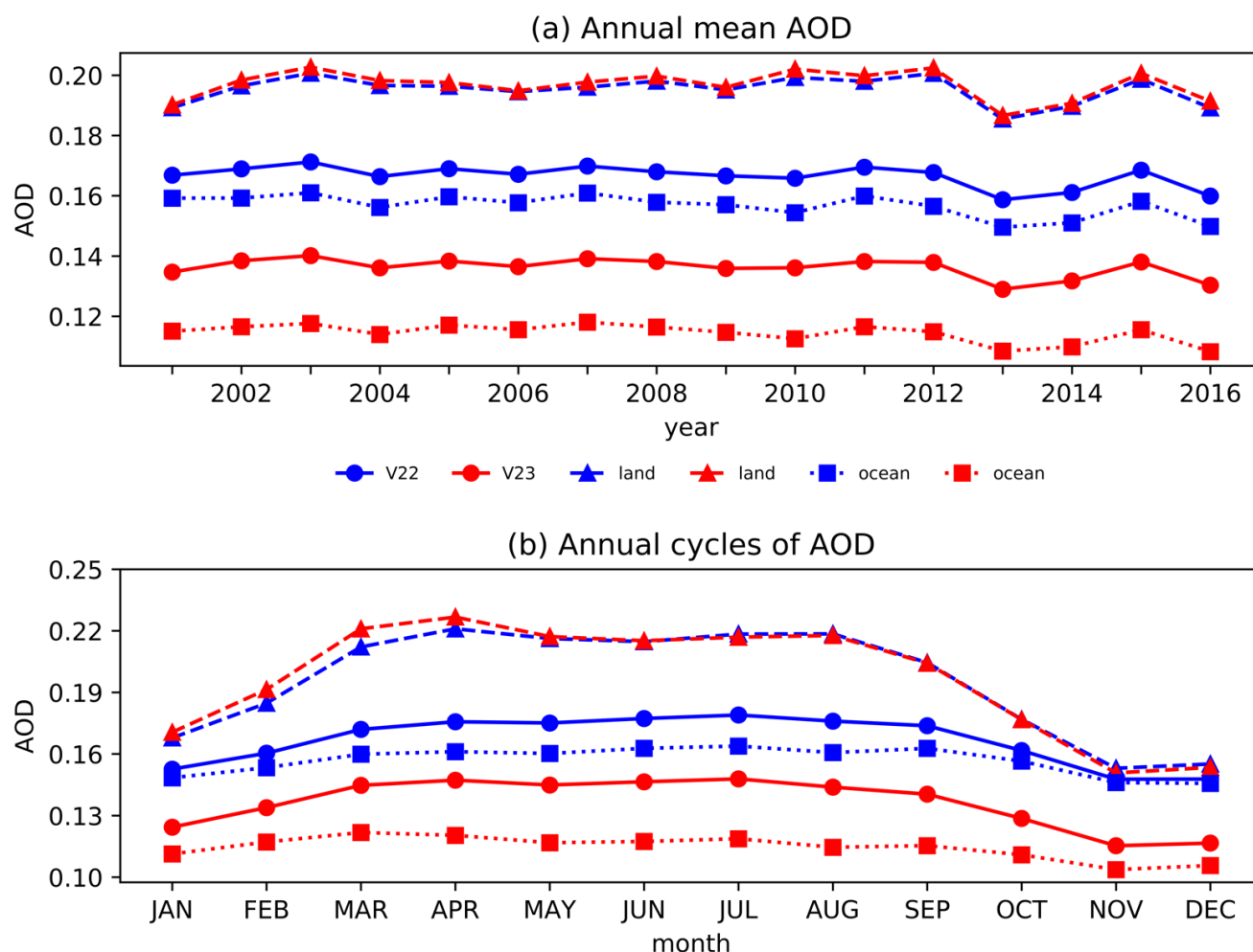
Figure 3 (a) Time series of annual mean AODs from V22 (blue) and V23 (red) between 2001 and 2016. Solid lines with circles, triangles with dashed lines, and squares with dotted lines represent global mean AOD, AOD averaged over land, and AOD averaged over ocean respectively. (b) Annual cycles of AOD. AOD for each month is averaged for the 16 years.
