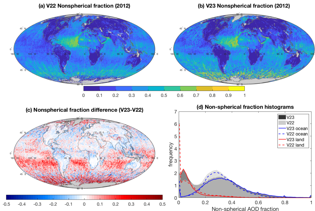
Figure 11 As in Figure 7 except for the MISR retrieved AOD fraction of nonspherical aerosol. AOD weighting is applied in nonspherical fraction averaging at each grid box.
