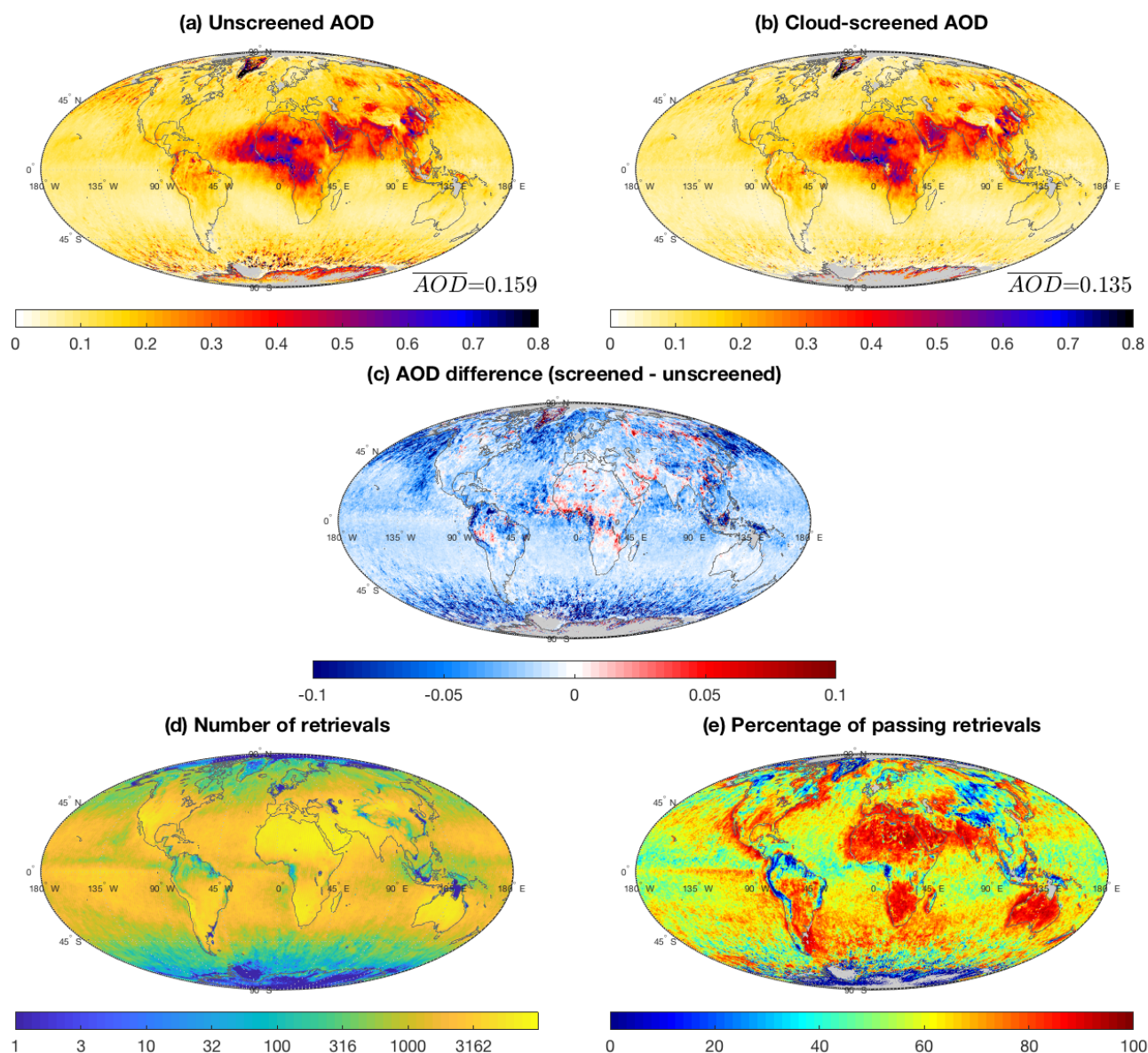
Figure 1 Effects of additional cloud screening implemented operationally in V23 shown using 0.5-degree gridded retrievals from 2012. (a) global AOD distribution prior to additional cloud screening; (b) global AOD distribution with operational cloud screening; (c) AOD difference between the screened and unscreened data; (d) number of retrievals (unscreened) in each grid box; (e) percentage of retrievals remaining after cloud screening. Average AOD values in (a) and (b) are area-weighted.
