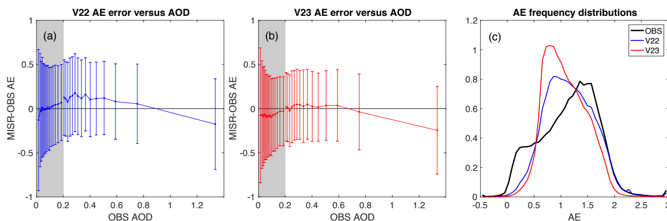
Figure 17 V22 and V23 AE comparisons against AERONET+MAN observations (OBS). (a) AE difference (MISR V22 – OBS) as a function of OBS AOD; data are split into two AOD regimes, \text{OBS AOD} \leq 0.2 and \text{OBS AOD} > 0.2 , and divided into 15 equally populated bins within each of the AOD regimes. The shaded area marks the smaller AOD regime. The markers represent the median AE difference values within each AOD bin and the error bars are one standard deviation of AE difference within each bin. (b) Same as (a) but for MISR V23 – OBS AE difference. (c) Normalized frequency distributions of AE obtained from the three collocated data sets. The total number of analyzed collocations is 61,015; 17,027 of collocations have \text{OBS AOD} > 0.2 .
