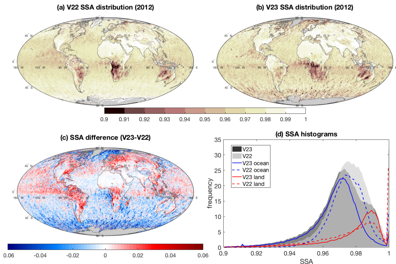
Figure 10 As in Figure 7 except for the MISR retrieved SSA. AOD weighting is applied in SSA averaging at each grid box.
