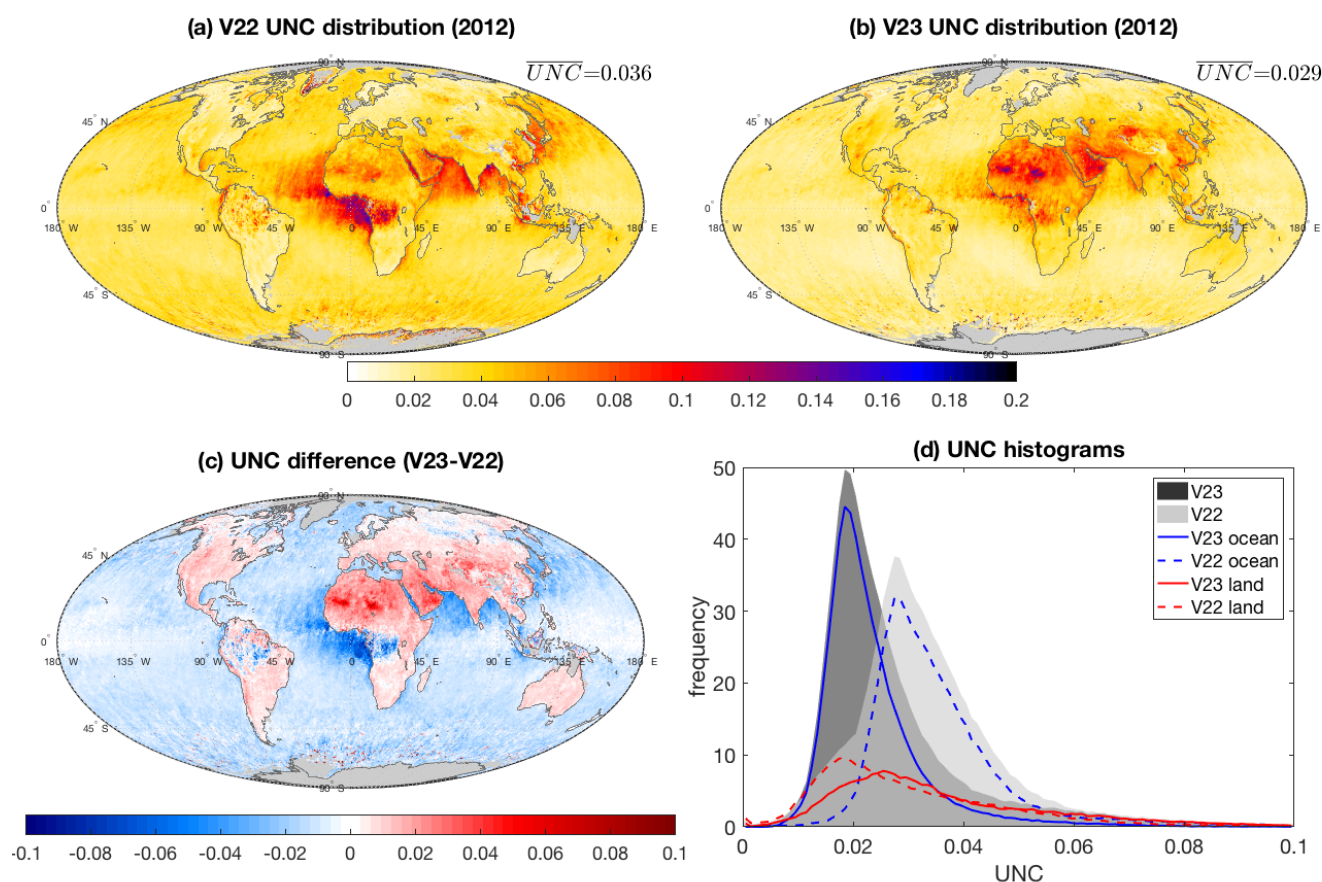
Figure 8 As in Figure 7 except for the MISR reported pixel-level AOD uncertainties (UNC). Because of the uncertainties related to extrapolating V22 UNC values from MISR 558 nm band to 550 nm band, the values from V22 are analysed at the 558 nm wavelength.
