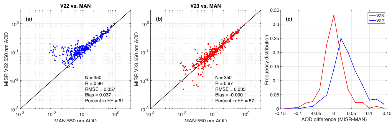
Figure 16 Scatter plots and statistical comparison between collocated MISR V22, MISR V23, and MAN observations. (a) Scatter plot of MISR V22/MAN collocations including overall statistics; (b) scatter plot of MISR V23/MAN collocations including overall statistics; (c) histograms of the MISR-MAN AOD difference for V23 (red) and V22 (blue) retrievals.
