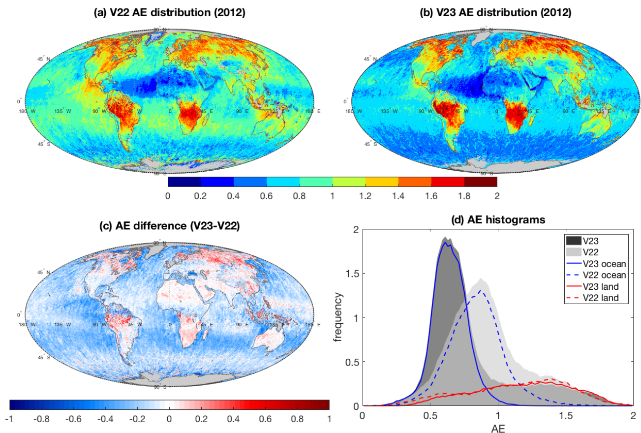
Figure 9 As in Figure 7 except for the MISR retrieved AE. AOD weighting is applied in AE averaging at each grid box.
