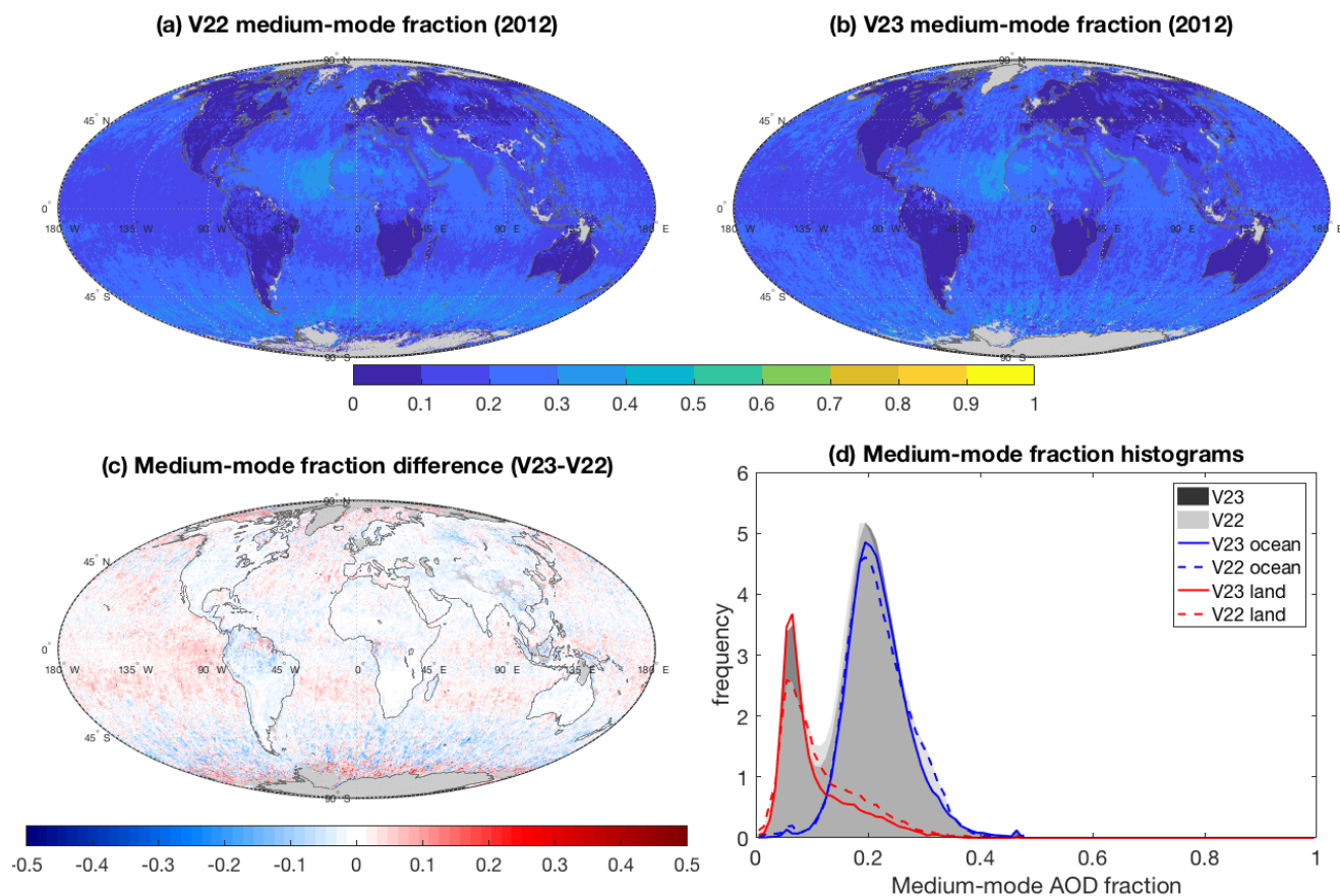
Figure 13 As in Figure 7 except for the MISR retrieved medium-mode AOD fraction. AOD weighting is applied in data averaging.
