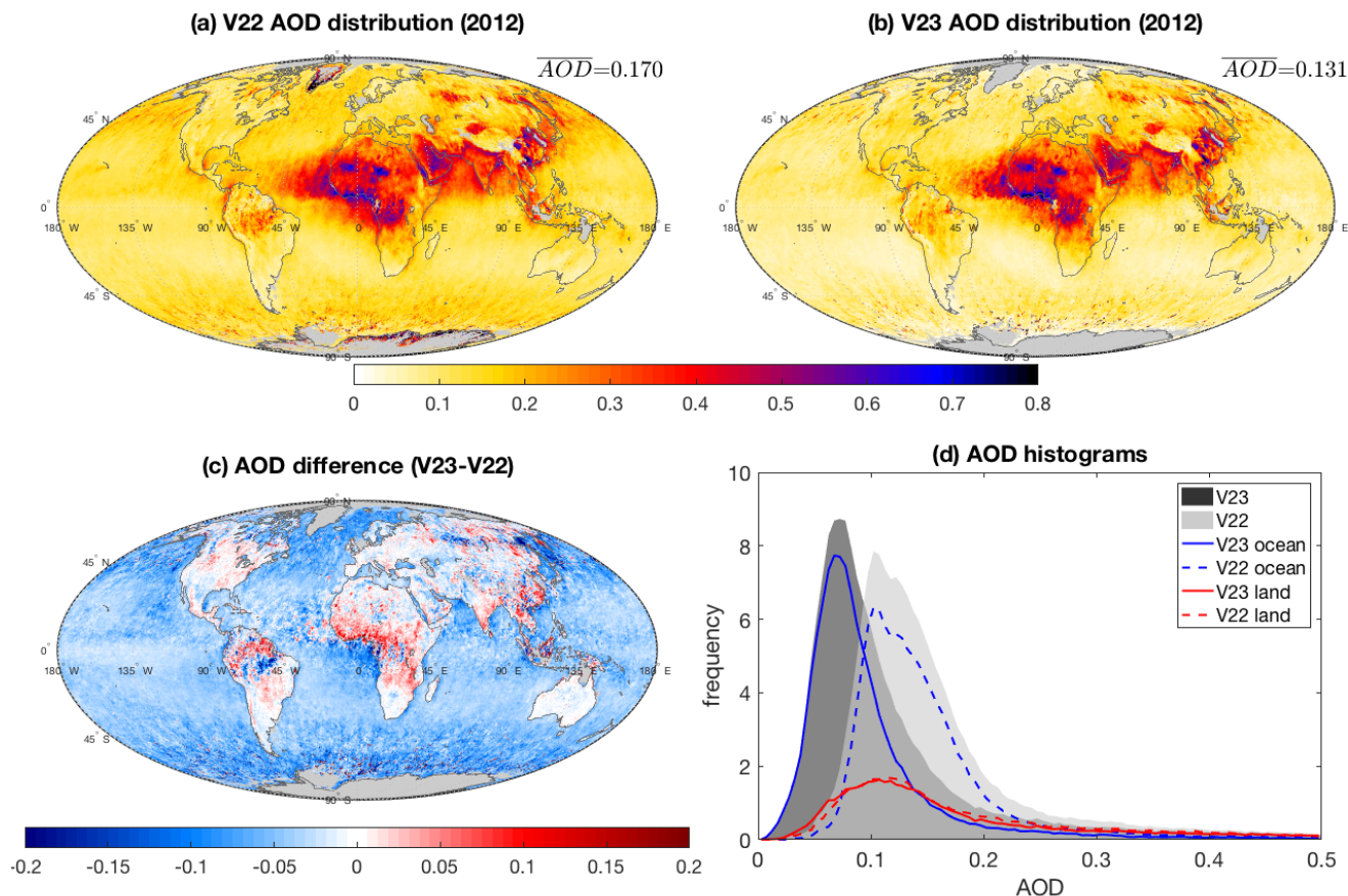
Figure 7 (a) Global distribution of AOD in 2012 from V22 retrievals gridded at 0.5-degree resolution; (b) same as (a) but using V23 retrievals; (c) AOD difference between V23 and V22. (d) Histograms of gridded AODs: the dark grey shading shows V23 data, the light grey shading shows V22 data, the solid lines show V23 retrievals over ocean (solid blue) and land (solid red), whereas the dashed lines show V22 retrievals over ocean (dashed blue) and land (dashed red).
