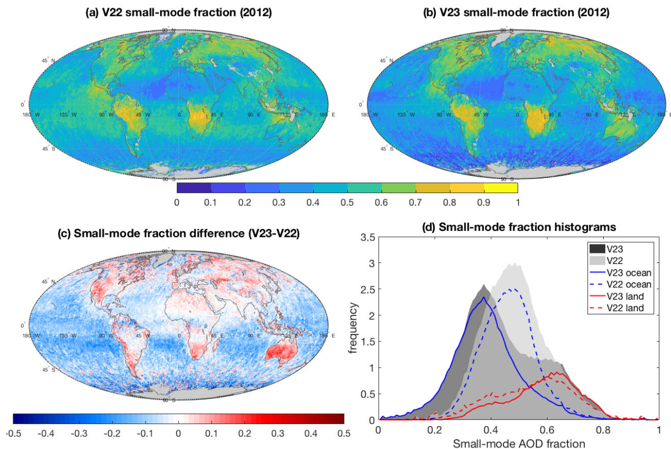
Figure 12 As in Figure 7 except for the MISR retrieved small-mode AOD fraction. AOD weighting is applied in data averaging.
