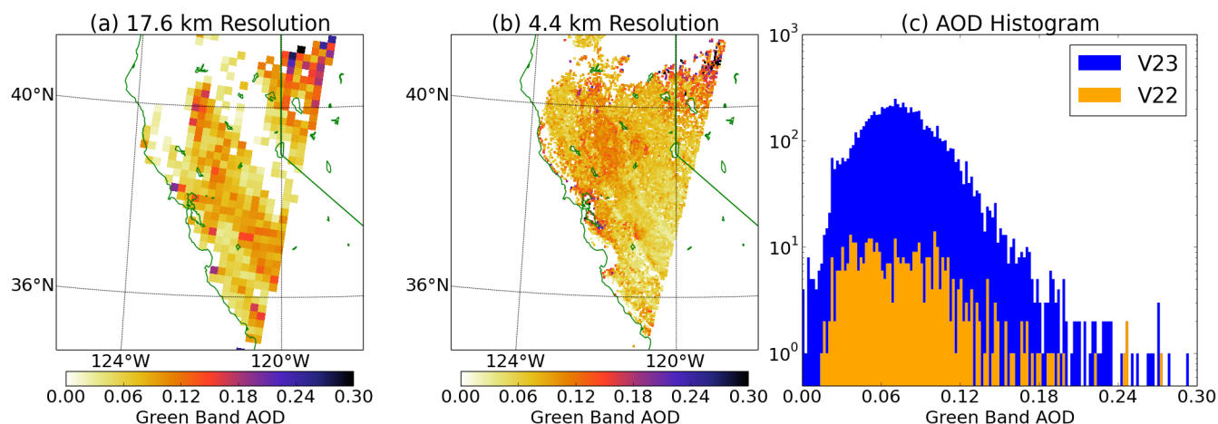
Figure 5 Comparison of V22 and V23 AOD retrievals for 5 July 2016 (Orbit 88022, Path 044). (a) V22 AOD map; (b) V23 AOD map; (c) AOD histograms.
