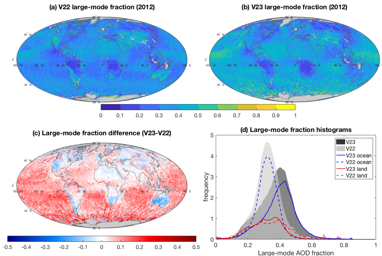
Figure 14 As in Figure 7 except for the MISR retrieved large-mode AOD fraction. AOD weighting is applied in data averaging.
