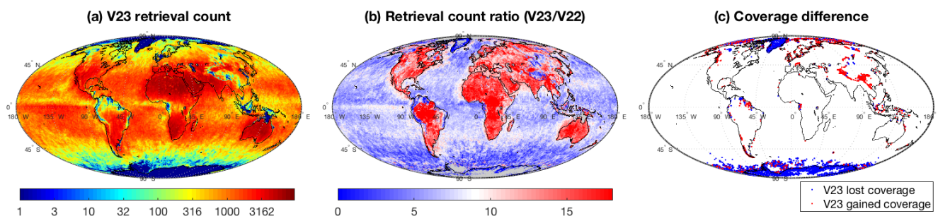
Figure 6 (a) Number of MISR V23 retrievals from 2012, gridded at 0.5-degree resolution, the color scale in decimal logarithm. (b) Ratio between the number of V23 retrievals and V22 retrievals; the average ratio, represented by white color in the color scale, is \sim 9.0 . (c) Locations of grid points where V23 loses (blue) or gains (red) coverage in comparison to V22.
