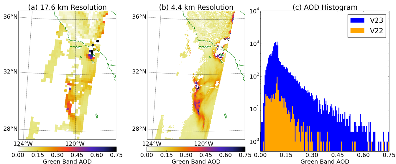
Figure 4 Comparison of V22 and V23 AOD retrievals for Orbit 88284, 23 July 2016. (a) V22 AOD map; (b) V23 AOD map; (c) AOD histograms.
