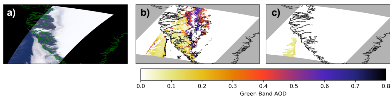
Figure 2 MISR V23 aerosol retrievals over Greenland for 15 August 2017 (Orbit 93932, Path 006). (a) MISR An camera RGB; (b) map of unscreened Aerosol_Optical_Depth_Raw retrievals; (c) map of screened Aerosol_Optical_Depth retrievals showing geographic exclusion over land as well as filtering of lower quality retrievals over the water.
