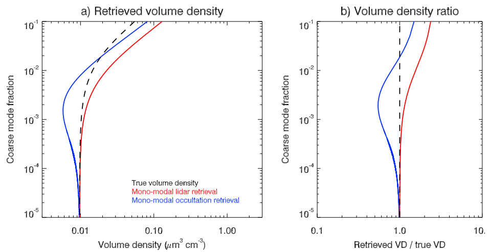
Figure 8. Similar to Fig. 3 but for volume density.
