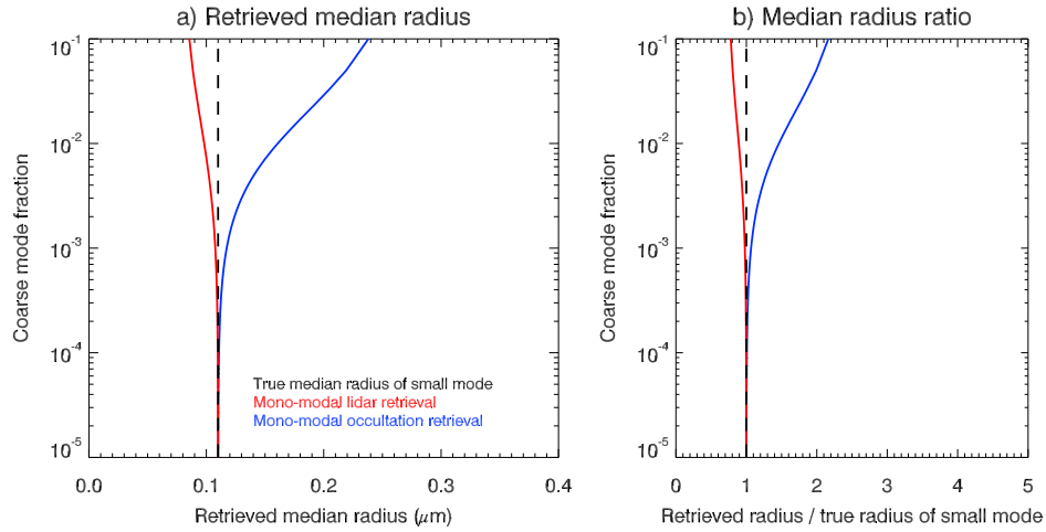
Figure 11. Similar to Fig. 3, but for a different set of parameters of the bi-modal particle size distribution ( r_1 = 110 \text{ nm} , S_1 = 1.4 , r_2 = 350 \text{ nm} , S_2 = 1.2 , i.e., case 3 in Table 1.
