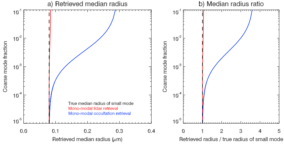
Figure 3. Left panel: The coarse mode fraction dependence of retrieved stratospheric aerosol median radius r_m is shown for an assumed mono-modal log-normal particle size distribution with S = 1.4 based on simulated lidar (red line) and satellite occultation (blue line) measurements. The actual aerosol particle size distribution is a bi-modal log-normal distribution. The black dashed line corresponds to the true median radius of the small mode. Note that the distribution width of the mono-modal distribution assumed for the retrievals was chosen to be identical to the width of the main mode of the bi-modal log-normal distribution used for the forward simulations. For the smallest coarse mode fractions, the median radius of the small mode can be well retrieved for all measurement geometries, as expected. Right panel: Ratio of the retrieved radii and the true median radius of the small mode of the bi-modal log-normal distribution.
