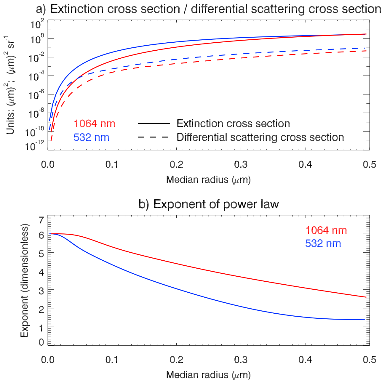
Figure 1. Top panel: The solid lines correspond to the median radius dependence of the Mie extinction cross section at 1064 nm (red line) and 532 nm (blue line) for a mono-modal log-normal particle size distribution with S = 1.4 . The dashed lines display the median radius dependence of the differential scattering cross section for a lidar backscatter geometry. Bottom panel: Dependence of the power law exponent (see Eq. (4)) of the dependence of the aerosol extinction cross section on median radius.
