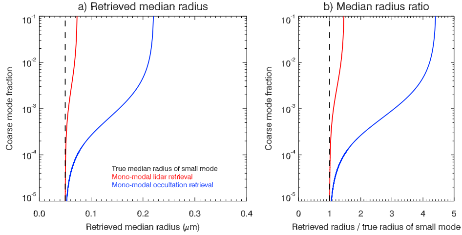
Figure 10. Similar to Fig. 3, but for a different set of parameters of the bi-modal particle size distribution ( r_1 = 50 \text{ nm} , S_1 = 1.4 , r_2 = 300 \text{ nm} , S_2 = 1.2 , i.e., case 2 in Table 1.
