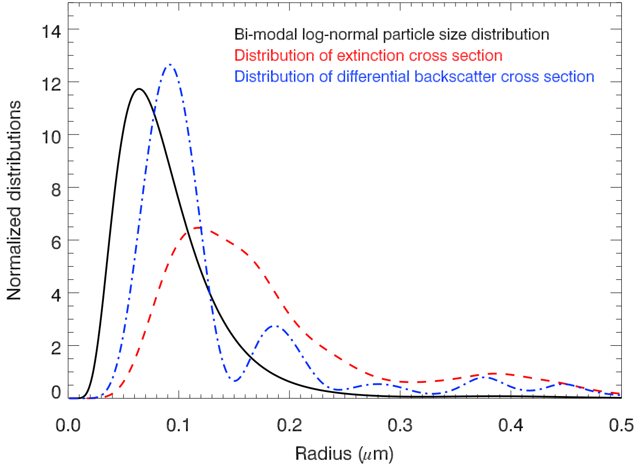
Figure 2. The black line shows the assumed bi-modal particle size distribution with two log-normal modes and the following parameters: r_1 = 80 \text{ nm} , S_1 = 1.6 , r_2 = 400 \text{ nm} , S_2 = 1.15 and a coarse mode fraction of \chi = 10^{-2} . The red dashed line corresponds to the particle size distribution multiplied by the Mie-extinction cross section \sigma_{ext}(\lambda = 532 \text{ nm}, r) . The blue dash-dotted line corresponds to the particle size distribution multiplied by the differential scattering cross section for a lidar backscatter geometry and also for a wavelength of 532 nm. Note that all functions are normalized.
