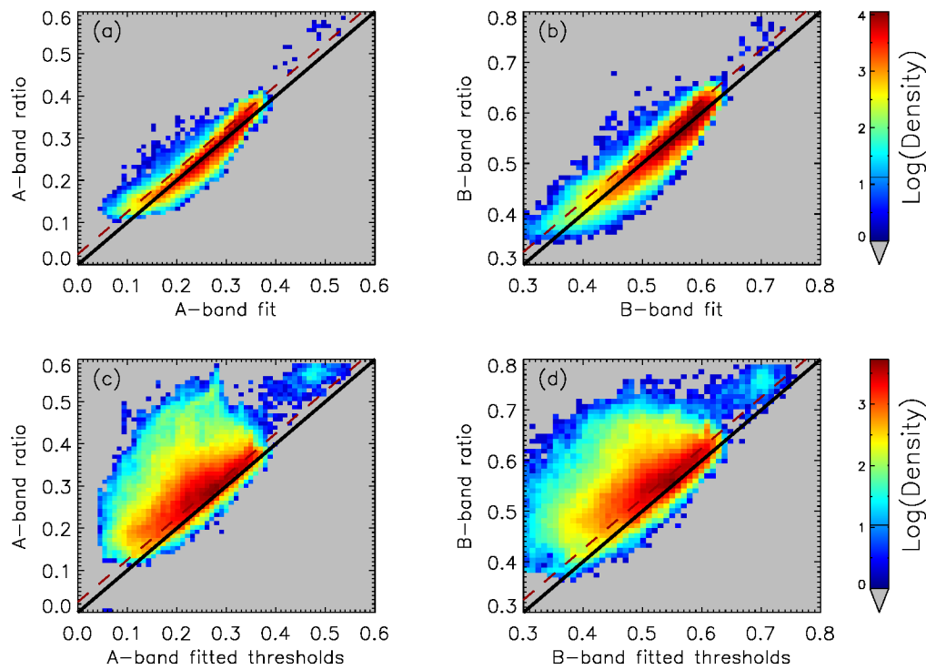
5 Figure 5. Scatter plot of regression fit versus A-band (left) and B-band (right) ratios for clear sky (a, b) and cloudy sky (c, d) pixels from EPIC measurements over global snow and ice surfaces in January and July 2017. The regression is derived with clear sky oxygen band ratio as a function of surface elevation and airmass. The pixels on the left (right) side of black lines could be identified as cloudy (clear) as the observed ratios is larger (smaller) than the predicted threshold. The dashed lines (increase the predicted ratios by 0.025) provide better division of clear and 10 cloudy pixels.
