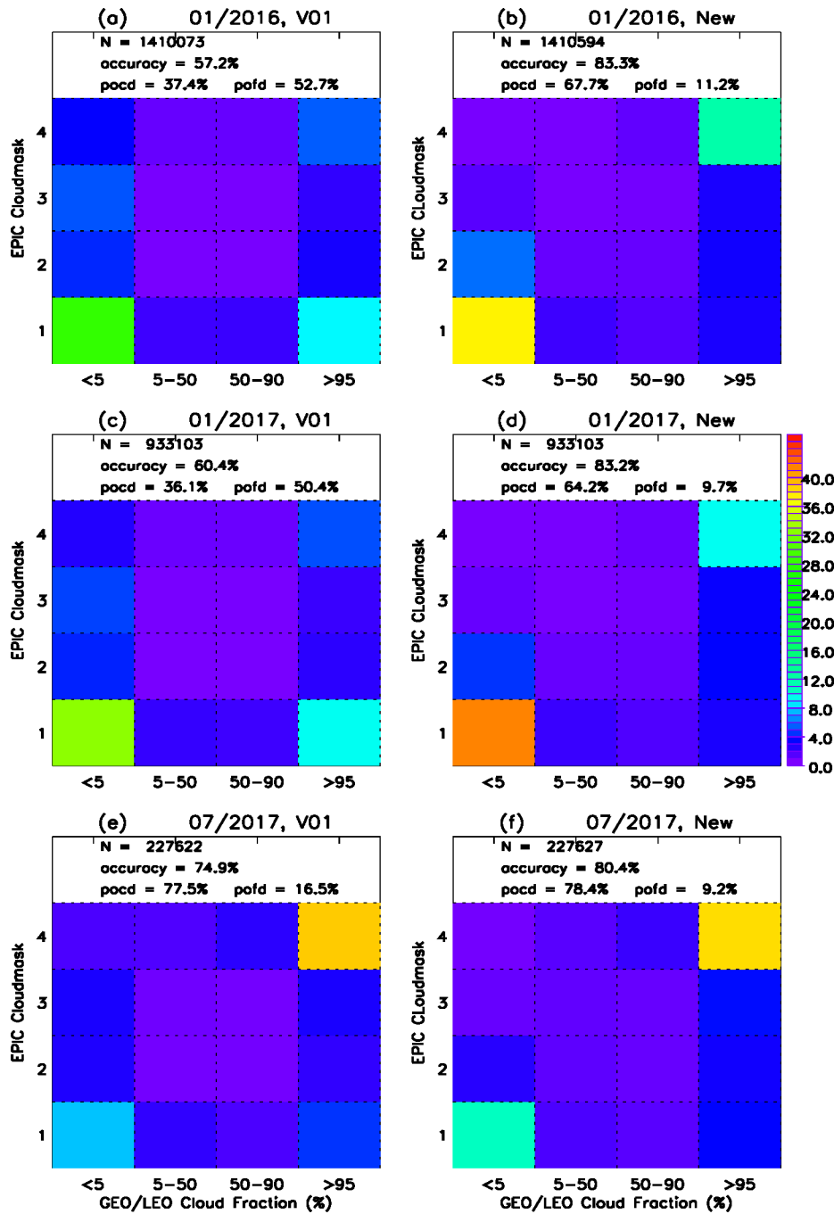
Figure 7. Percentage of pixels in each pixel-by-pixel matchup category between cloud mask from EPIC and GEO/LEO composite cloud fraction over snow and ice surfaces for January 2016 (a, b), January 2017 (c, d), and July 2017 (e, f). Left is from the current EPIC cloud mask algorithm and the right is from the new algorithm. The diagonal squares represent agreement between GEO/LEO and EPIC cloud mask, while the off-diagonal squares represent disagreement between
