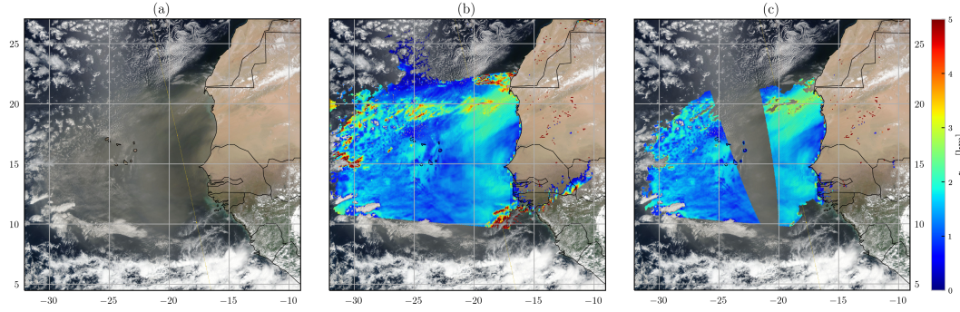
Figure 1. (a) A VIIRS corrected reflectance image over the West African coast on the 8 th of June, 2018. (b) All successful TROPOMI retrievals within a certain bounding box. (c) Same as (b) but with all pixels that possibly fall within the sun glint region or are cloud contaminated are removed (using cloud_warning flag and sun_glnt_warning from Table 1).
