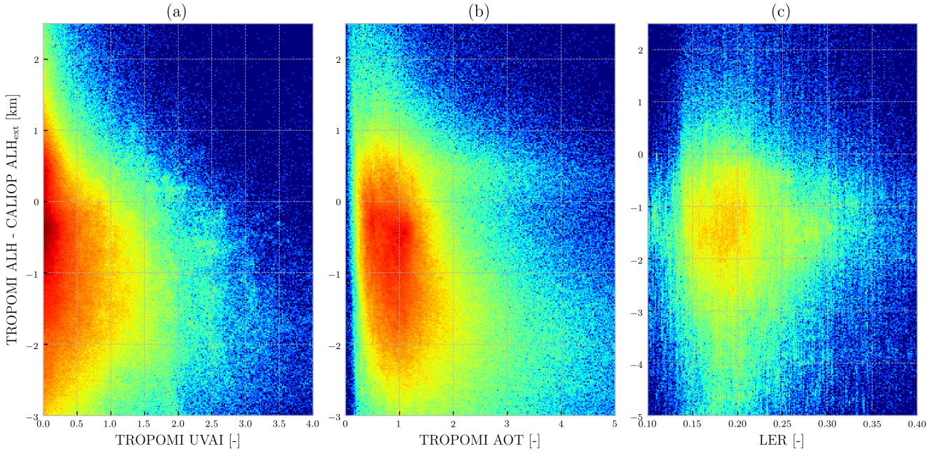
Figure 4. Scatter density plots of the difference between TROPOMI ALH and CALIOP ALH ext as a function of (a) TROPOMI UVAI, (b) TROPOMI AOT and (c) GOME-2 LER for the oxygen A-band used for the TROPOMI retrievals for cases over land (with a minimum surface albedo of 0.1). The colors represent density of plots. The y axis is optimised for each plot. The data is filtered in the same fashion as in Figure 2, with data over the ocean and land combined for plots (a) and (b), and data only over land for plot (c).
