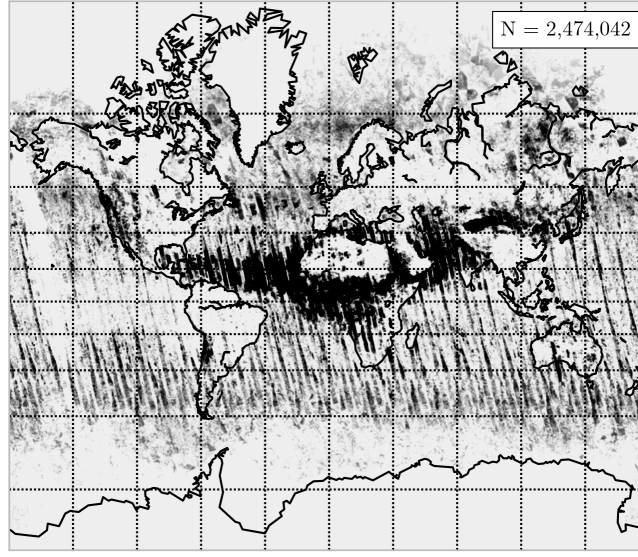
Figure 8. A map of all TROPOMI-CALIOP collocations considered for Figure 2 (data filtering discussed in Appendix A).
