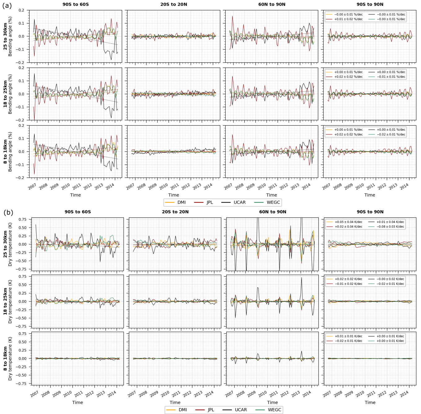
Figure 5. F3C bending angle (a) and dry temperature (b): De-seasonalized anomaly difference time series based on 10^\circ -zonal medians of each center to the all-center mean for latitude bands 90^\circ\text{S} to 60^\circ\text{S} , 20^\circ\text{S} to 20^\circ\text{N} , 60^\circ\text{N} to 90^\circ\text{N} and globally 90^\circ\text{S} to 90^\circ\text{N} (left to right) for altitude layers 8–18 km, 18–25 km, 25–30 km (bottom to top). Time series from DMI (orange), JPL (red), UCAR (black), and WEGC (green) are shown.
