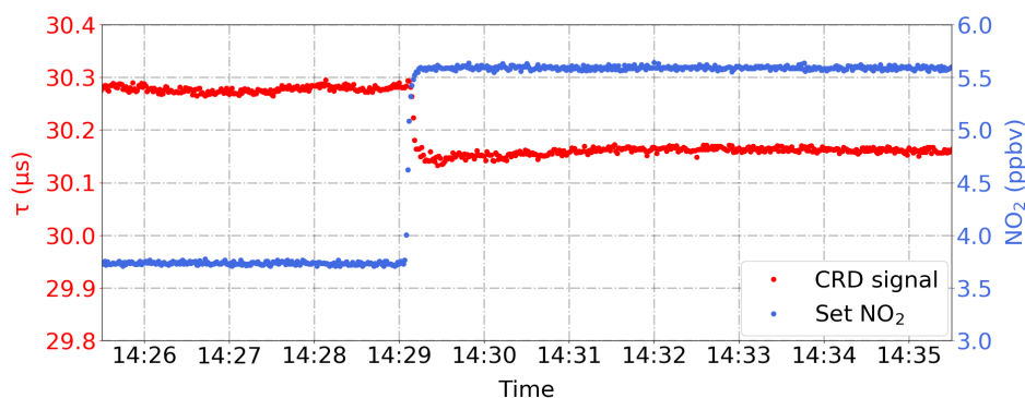
Fig. 1. Figure RC1_1: PeRCEAS response to a step change in sampled NO 2 mixing ratio
