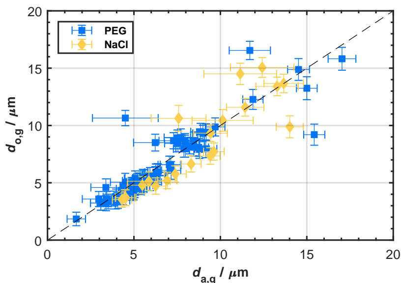
Figure 4. Particle sizing of PPD-HS and APS for spherical (PEG) and aspherical (NaCl) particles, showing the geometric mean of the optical diameter determined by PPD-HS as a function of the geometric mean of the aerodynamic diameter obtained from the APS, using the calibration setup shown in Fig. 3. Vertical and horizontal error bars indicate the geometric standard deviation of the optical and aerodynamic mean size, respectively. Data points outside the size range of the APS are not shown. A complete list of the individual data sets, including those covering sizes > 20 \mu\text{m} , is given in SI Tab. S1.
