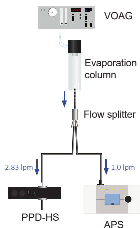
Figure 3. Experimental set up used for PPD-HS calibration measurements. A VOAG was used to generate both spherical and aspherical particles of different sizes. An APS was operated in parallel to PPD-HS, in order to monitor the particle size distribution (see example size distribution in SI Fig. S12). A vacuum pump, attached downstream of PPD-HS, is used to draw air through PPD-HS.
