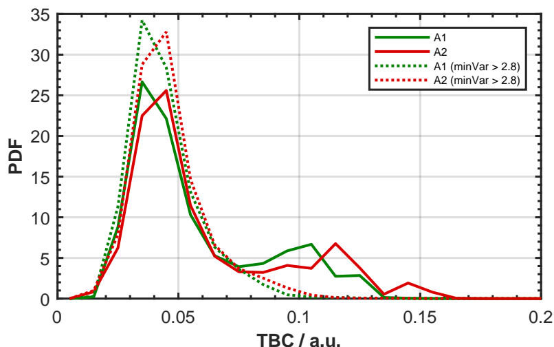
Figure A3. Example comparison of TBC distributions of a VOAG data set of spherical particles ( 5\ \mu\text{m} PEG) when the minimum variance criterion of 2.8 is (dotted) and is not (solid) applied. Green lines correspond to array 1 and red to array 2.
