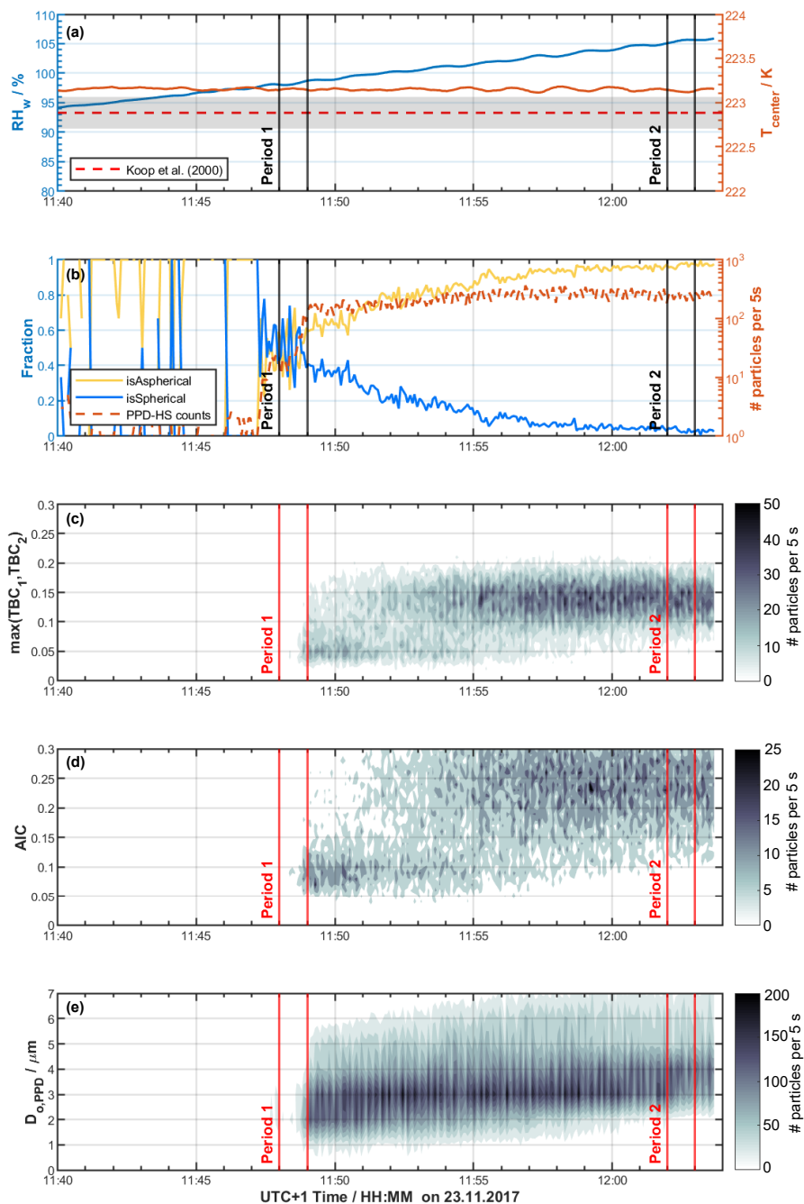
Figure 7. Freezing experiments of \text{NH}_4\text{NO}_3 aerosol using HINC at T = 223 K and a residence time \tau = 22 s. (a) RH_w (blue line, left-hand ordinate) along with T_{center} at HINC center line (orange line, right-hand ordinate), where aerosol particles are injected and hydrometeors are formed. (b) classification of particles detected by PPD-HS (left-hand ordinate) using random forest model (see Sect. 3.2) along with total number of detected particles (dashed, orange line, right-hand ordinate). (c) distribution of maximum TBC value and (d) AIC value of PPD-HS scattering patterns. (e) PPD-HS optical particle size distribution obtained from RT-electronics. Vertical solid lines indicate starting and end times of periods of interest, respectively.
