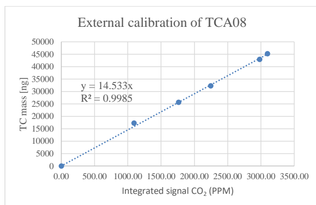
Figure 5 External calibration of TCA08 - determination of carbon calibration constant
