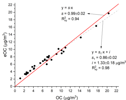
10 Figure 8: Comparisons of offline measurements of OC (laboratory filter analysis) using the EUSAAR_2 thermal protocol, to the 24-hour average of online measurement of OC=TC- b BC data taken by the AE33 Aethalometer and TCA08 Total Carbon Analyzer. Linear orthogonal regression results (n=31) are shown with s as the slope (red line) for the model without an intercept and with s 1 as slope and i as intercept (dashed gray line) for the model with an intercept. R 2 xy is the square of the Pearson correlation coefficient.
