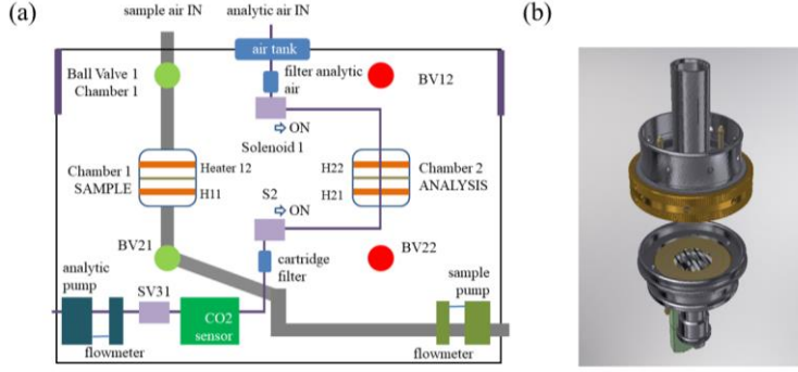
Figure 6: (a) The TCA08 flow diagram. While chamber 1 collects a new atmospheric sample on the quartz-fiber filter, chamber 2 performs a thermal analysis of the previously collected sample. The system of ball valves (BV11, BV21, BV12, BV22) and solenoids (S1 and S2) change the airflows after the sample time-base. (b) The analytical chamber of the TCA08 Total Carbon Analyzer is made of stainless steel. It supports the quartz-fiber aerosol collection filter between two closely-spaced heating elements, one above and one below.
