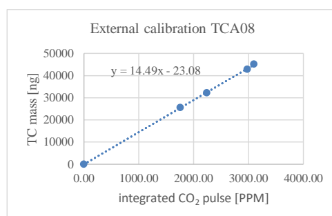
Figure 1 External calibration of TCA08 - TC mass calibration range
