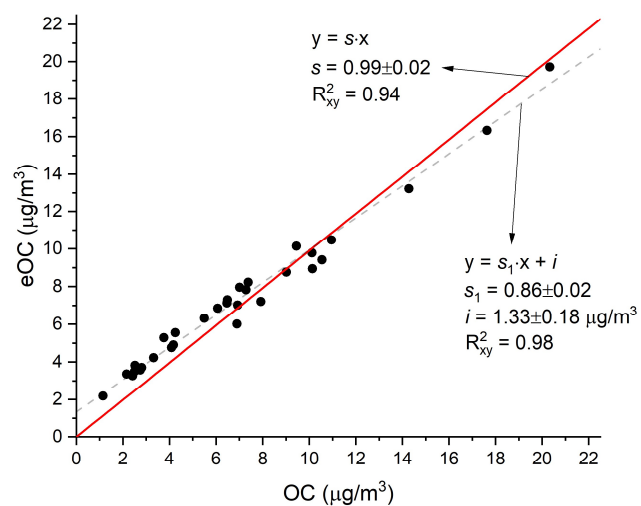
Figure 8: Comparisons of offline measurements of OC (laboratory filter analysis) using the EUSAAR_2 thermal protocol, to the 24-hour average of online measurement of OC=TC-bBC data taken by the AE33 Aethalometer and TCA08 Total Carbon Analyzer. Linear orthogonal regression results (n=31) are shown with s as the slope (red line) for the model without an intercept and with s_1 as slope and i as intercept (dashed gray line) for the model with an intercept. R^2_{xy} is the square of the Pearson correlation coefficient.
