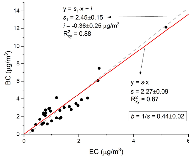
Figure 7: Comparisons of offline measurements of EC (laboratory filter analysis) using the EUSAAR_2 thermal protocol, to the 24-hour average of online measurements of BC data taken by the AE33 Aethalometer. Linear orthogonal regression results are shown with s as the slope (red line) for the model without an intercept and with s_1 as slope and i as intercept (dashed gray line) for the model with an intercept. R^2_{xy} is the square of the Pearson correlation coefficient. 31 samples were collected for analysis during the campaign.
