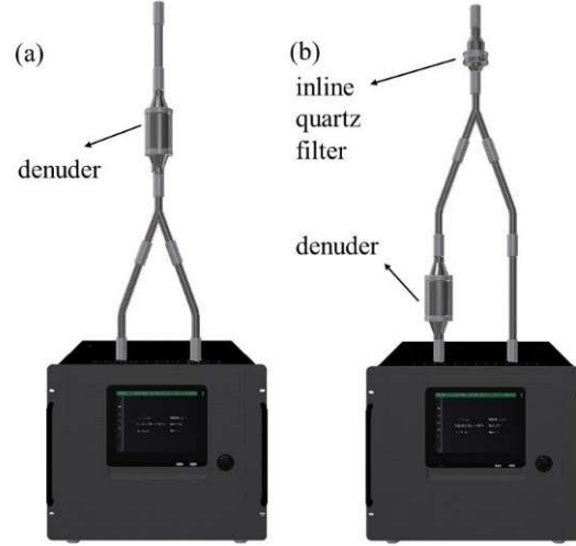
Figure 3: TCA08 setup when (a) sampling and (b) performing denuder efficiency test. Note that the tubing length is identical in both setups. This permits the test to be performed at a permanent installation without disturbing the inlet plumbing.
