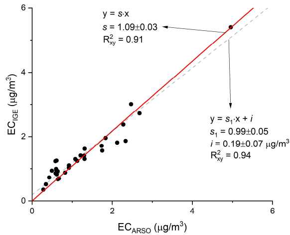
Figure 4: Comparisons of offline measurements of (a) TC, (b) OC and (c) EC from the ARSO and IGE laboratory analyses. OC and EC were measured using the EUSAAR 2 thermal protocol. Linear orthogonal regression results are shown with s as the slope (red line) for the model without an intercept and with s_1 as slope and i as intercept (dashed gray line) for the model with an intercept. R_{xy}^2 is the square of the Pearson correlation coefficient. 31 samples were collected for analysis during the campaign.
