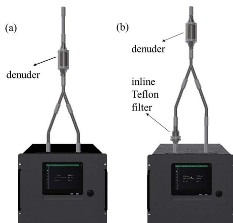
Figure S1. TCA08 setup when (a) sampling and (b) performing semi-continuous denuder breakthrough measurement. Note that the tubing length is identical in both setups. This permits the test to be performed at a permanent installation without disturbing the inlet plumbing.
