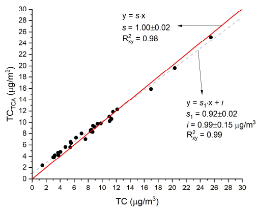
Figure 6: Comparison of offline measurements of TC (laboratory filter analyses), to the 24-hour average of 1-hour online measurements of TC from the TCA08. Linear orthogonal regression results are shown with s as the slope (red line) for the model without an intercept and with s_1 as slope and i as intercept (dashed gray line) for the model with an intercept. R_{xy}^2 is the square of the Pearson correlation coefficient. 31 samples were collected for analysis during the campaign.
