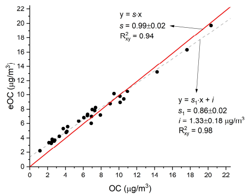
Figure 8: Comparison of offline measurements of OC (laboratory filter analysis) using the EUSAAR_2 thermal protocol, to the 24-hour average of online measurement of OC=TC-bBC data taken by the AE33 Aethalometer and TCA08 Total Carbon Analyzer. Linear orthogonal regression results (n=31) are shown with s as the slope (red line) for the model without an intercept and with s_1 as slope and i as intercept (dashed gray line) for the model with an intercept. R^2_{xy} is the square of the Pearson correlation coefficient.
