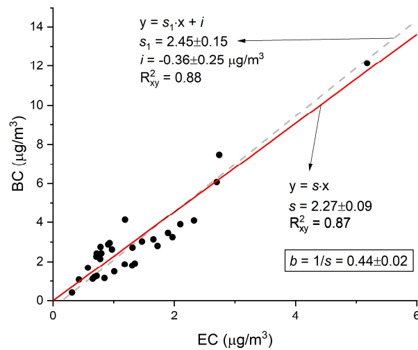
Figure 7: Comparison of offline measurements of EC (laboratory filter analysis) using the EUSAAR_2 thermal protocol, to the 24-hour average of online measurements of BC data taken by the AE33 Aethalometer. Linear orthogonal regression results are shown with s as the slope (red line) for the model without an intercept and with s_1 as slope and i as intercept (dashed gray line) for the model with an intercept. R^2_{xy} is the square of the Pearson correlation coefficient. 31 samples were collected for analysis during the campaign.
