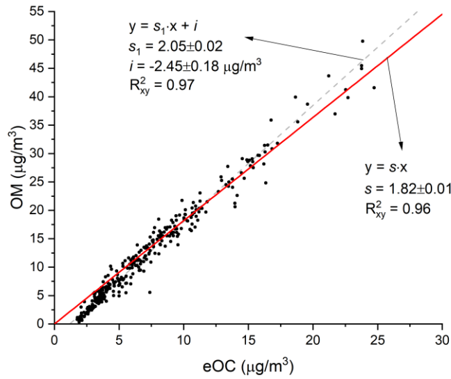
Figure 11: (a) Comparison of offline measurements of OC (laboratory filter analysis) using the EUSAAR_2 thermal protocol, to the 24-hour average of online measurement of OM data taken by the ACSM. A total of 31 filter samples were collected for analysis during the campaign. Please note that red trendline completely covers dashed trendline ( s=s_1 ). (b) Comparison of 3h eOC data derived as eOC = TC - bBC , to OM data measured by ACSM. Linear orthogonal regression results are shown with s as the slope (red line) for the model without an intercept and with s_1 as slope and i as intercept (dashed gray line) for the model with a intercept. R^2_{xy} is the square of the Pearson correlation coefficient. 300 data points are used in the regression analysis.
