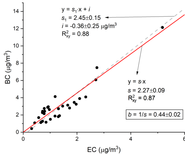
Figure 7: Comparison of offline measurements of EC (laboratory filter analysis) using the EUSAAR_2 thermal protocol, to the 24-hour average of online measurements of BC data taken by the AE33 Aethalometer. Linear orthogonal regression results are shown with s as the slope (red line) for the model without an intercept and with s_1 as slope and i as intercept (dashed gray line) for the model with an intercept. R^2_{xy} is the square of the Pearson correlation coefficient. 31 samples were collected for analysis during the campaign.
