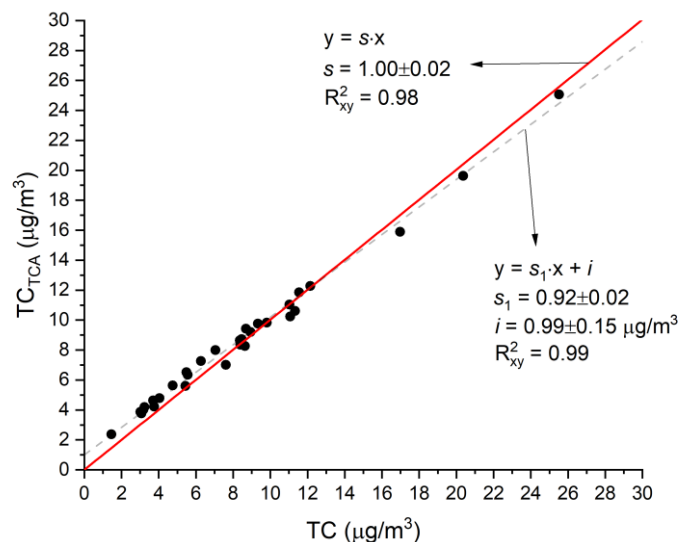
Figure 6: Comparison of offline measurements of TC (laboratory filter analyses), to the 24-hour average of 1-hour online measurements of TC from the TCA08. Linear orthogonal regression results are shown with s as the slope (red line) for the model without an intercept and with s_1 as slope and i as intercept (dashed gray line) for the model with an intercept. R_{xy}^2 is the square of the Pearson correlation coefficient. 31 samples were collected for analysis during the campaign.
