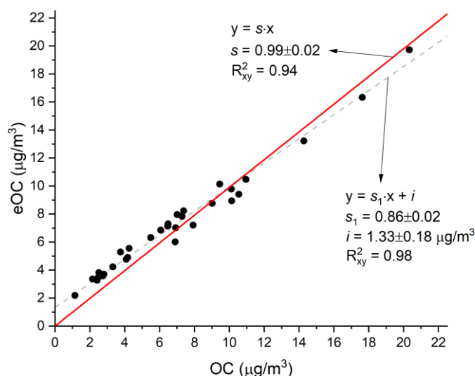
Figure 8: Comparison of offline measurements of OC (laboratory filter analysis) using the EUSAAR_2 thermal protocol, to the 24-hour average of online measurement of OC=TC- b BC data taken by the AE33 Aethalometer and TCA08 Total Carbon Analyzer. Linear orthogonal regression results ( n=31 ) are shown with s as the slope (red line) for the model without an intercept and with s_1 as slope and i as intercept (dashed gray line) for the model with an intercept. R^2_{xy} is the square of the Pearson correlation coefficient.
