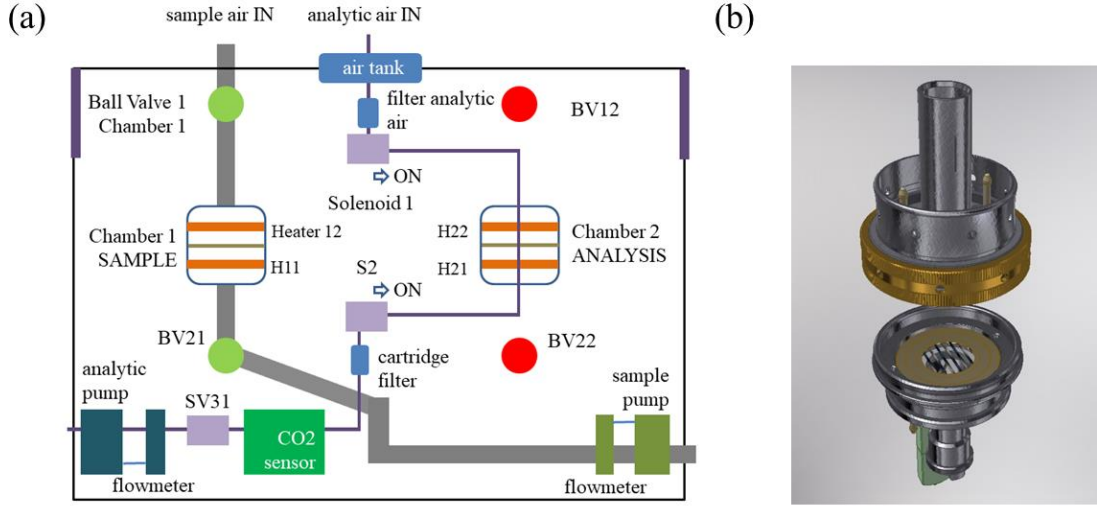
5 Figure 1: (a) The TCA08 flow diagram. While chamber 1 collects a new atmospheric sample on the quartz-fiber filter, chamber 2 performs a thermal analysis of the previously collected sample. The system of ball valves (BV11, BV21, BV12, BV22) and solenoids (S1 and S2) change the airflows after the sample time-base. (b) The analytical chamber of the TCA08 Total Carbon Analyzer is made of stainless steel. It supports the quartz-fiber aerosol collection filter between two closely-spaced heating elements, one above and one below.
