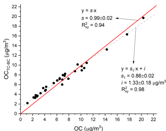
25 Figure 8: Comparisons of offline measurements of OC (laboratory filter analysis) using the EUSAAR_2 thermal protocol, to the 24-hour average of online measurement of OC=TC-bBC data taken by the AE33 Aethalometer and TCA08 Total Carbon Analyzer. Linear orthogonal regression results ( n=31 ) are shown with s as the slope (red line) for the model without an intercept and with s_1 as slope and i as intercept (dashed gray line) for the model with an intercept. R^2_{xy} is the square of the Pearson correlation coefficient.
