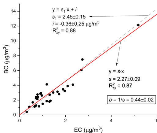
Figure 7: Comparisons of offline measurements of EC (laboratory filter analysis) using the EUSAAR_2 thermal protocol, to the 24-hour average of online measurements of BC data taken by the AE33 Aethalometer. Linear orthogonal regression results are shown with s as the slope (red line) for the model without an intercept and with s_1 as slope and i as intercept (dashed gray line) for the model with an intercept. R^2_{xy} is the square of the Pearson correlation coefficient. 31 samples were collected for analysis during the campaign.
