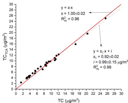
5 Figure 6: Comparison of offline measurements of TC (laboratory filter analyses), to the 24-hour average of 1-hour online measurements of TC from the TCA08. Linear orthogonal regression results are shown with s as the slope (red line) for the model without an intercept and with s_1 as slope and i as intercept (dashed gray line) for the model with an intercept. R_{xy}^2 is the square of the Pearson correlation coefficient. 31 samples were collected for analysis during the campaign.
