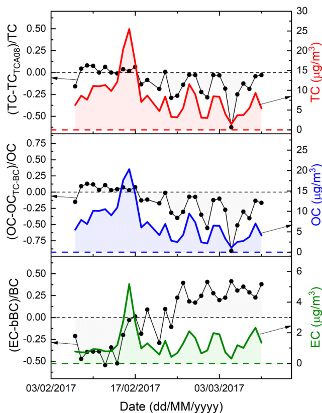
Figure 9: Left y-axis: Relative difference between TC, OC and EC (see Eq. 7) measured on 24 h filters by conventional OC-EC method and TC_{TCA08} , TC-bBC and bBC measured online by TCA08 on 1 h time resolution and AE33 on 1 min time resolution and then averaged on 24 h. Right y-axis: The absolute concentrations of TC, OC and EC (red, blue and green line, respectively) is shown for easier comparison.
