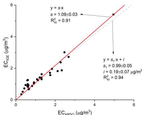
5 Figure 4: Comparisons of offline measurements of (a) TC, (b) OC and (c) EC from the ARSO and IGE laboratory analyses. OC and EC were measured using the EUSAAR_2 thermal protocol. Linear orthogonal regression results are shown with s as the slope (red line) for the model without an intercept and with s_1 as slope and i as intercept (dashed gray line) for the model with an intercept. R_{xy}^2 is the square of the Pearson correlation coefficient. 31 samples were collected for analysis during the campaign.
