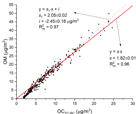
Figure 11: (a) Comparison of offline measurements of OC (laboratory filter analysis) using the EUSAAR_2 thermal protocol, to the 24-hour average of online measurement of OM data taken by the ACSM. A total of 31 filter samples were collected for analysis during the campaign. (b) Comparison of 3h OC data derived as OC = TC - bBC , to OM data measured by ACSM. Linear orthogonal regression results are shown with s as the slope (red line) for the model without an intercept and with s_1 as slope and i as intercept (dashed gray line) for the model with a intercept. R_{xy}^2 is the square of the Pearson correlation coefficient. 300 data points are used in the regression analysis.
