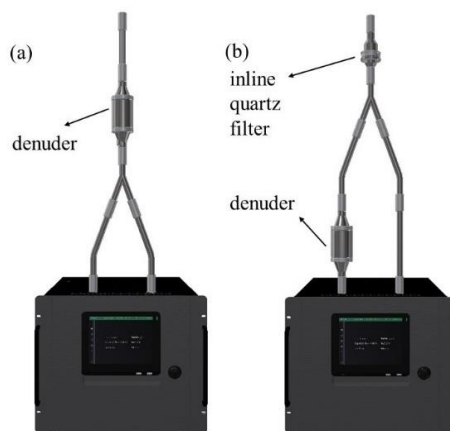
10 Figure 3: TCA08 setup when (a) sampling and (b) performing denuder efficiency test. Note that the tubing length is identical in both setups. This permits the test to be performed at a permanent installation without disturbing the inlet plumbing.
