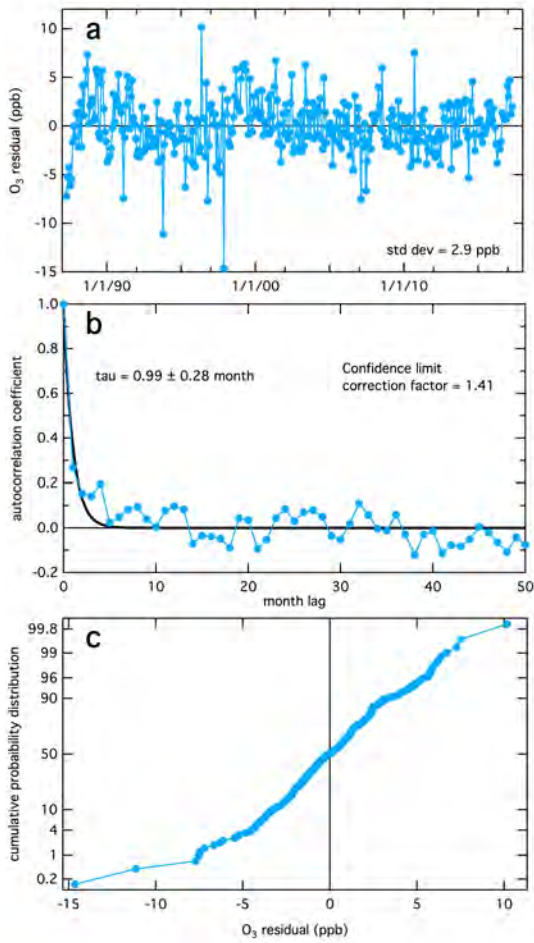
5 | Figure 6. Analysis of the deviations between the monthly mean baseline ozone concentrations and the fit of Eq. 4 to these means (i.e. the fit residuals) illustrated in Figure 4. a) Time series of the residuals. b) The time lag autocorrelation of the residuals. The fitted curve is an exponential decrease from unity at a lag of 0 month, with the time constant, \tau , annotated. c) Cumulative probability distribution of the residuals, plotted on an ordinate scale that gives a linear fit for a Gaussian distribution.
