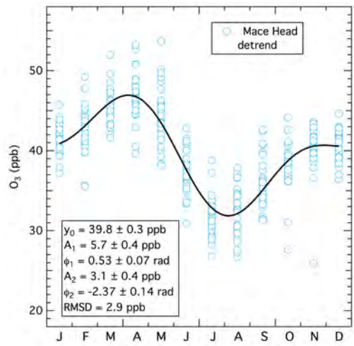
5 | Figure 3. Results of the fit of Eq. 3 to the detrended monthly mean concentrations. The black curve is the non-linear regression fit to the plotted points.
