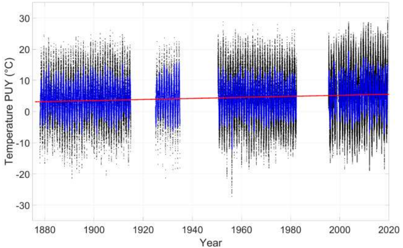
Figure 4: Long series of temperature at PUY station. The hourly means are in black, the monthly means are in blue and the linear regression line is in red (slope: +1.4 \pm 0.7 °C per century).
