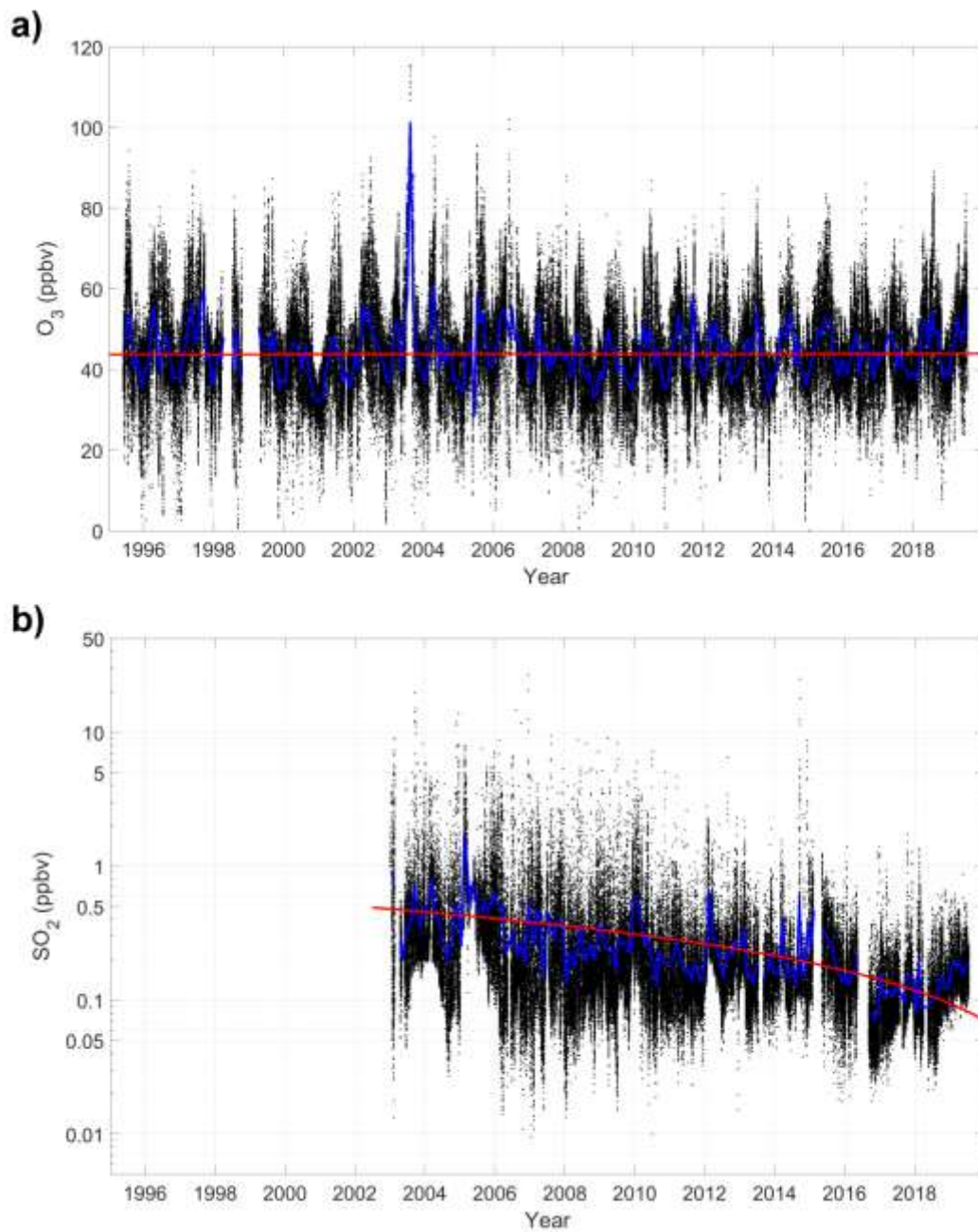
1350 Figure 8: Long series of reactive gases at PUY station: O_3 (a, slope: -0.1 \pm 1.2 ppbv per decade) and SO_2 (b, slope: -0.23 \pm 0.05 ppbv per decade). The SO_2 values have been plotted on a logarithmic y axis. The color code is the same as Figures 4 and 7.
