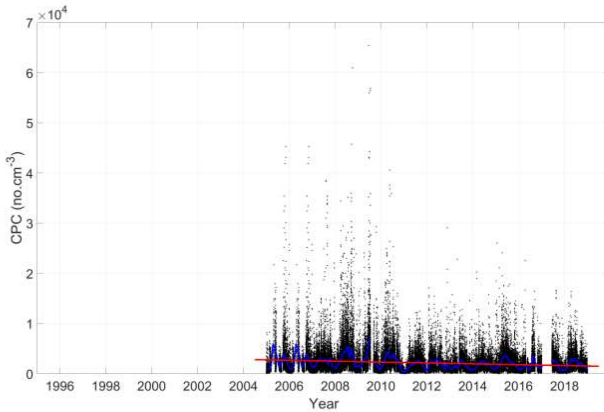
1355 Figure 9: Long series of aerosol particles number at PUY station (slope: -9 \pm 5 \cdot 10^2 \text{ cm}^{-3} per decade). The color code is the same as Figure 4, 7 and 8.
