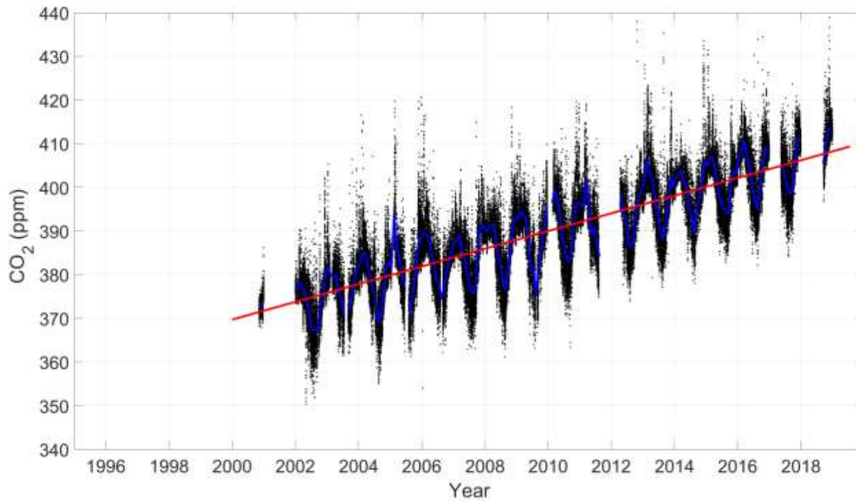
1345 Figure 7: Long series of CO 2 at PUY station (slope: +20.2 \pm 1.7 ppm per decade). The hourly means are in black, the monthly means are in blue and the linear regression line is in red.
