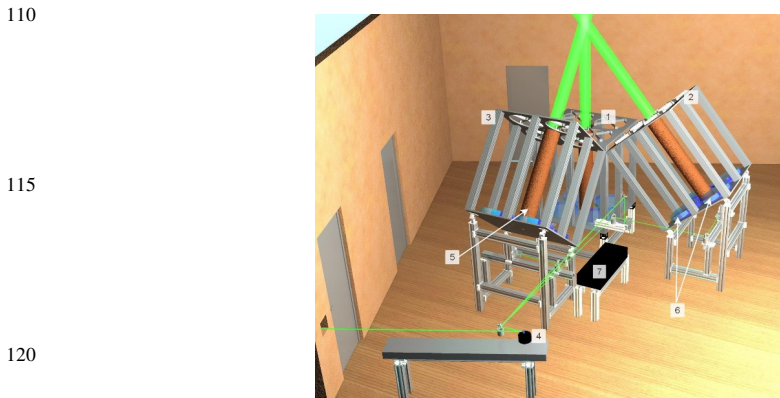
125 Figure 1. Three-dimensional representation of the transmitter-receiver system of LIOvent lidar comprising three telescope assemblies for zenith (1), north (2) and east (3) lines-of-sight with four collecting mirrors (6) and a beam expander (5) each. The emitted laser beam is commuted between the telescopes using rotating scanner mirror (4). The backscattered light collected by each mirror is transferred via fibers into the optical commutation chamber (7) for aggregating the fluxes from the four mirrors of each telescope assembly.
