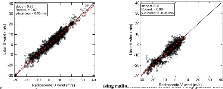
Fig. 5. Comparison of the zonal (a) and meridional (b) wind velocities measured by the lidar and the radiosondes. The solid black line is shown in solid black, the linear regression line is shown in dashed red.
