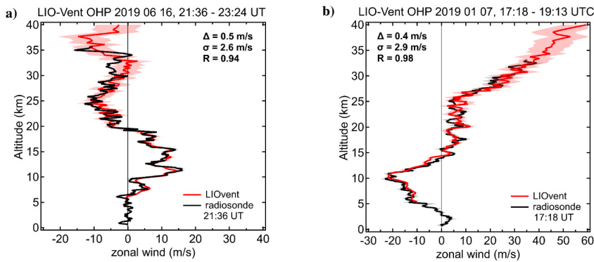
Figure 6. Selected cases of the lidar-radiosonde intercomparison of the zonal wind profiles in June (a) and January (b) 2019. The lidar measurement dates and times are given above the panels, the time of radiosonde launch on the same date is provided in the legend.
