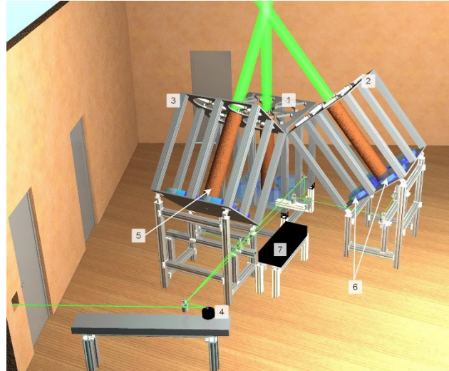
115 Figure 1. Three-dimensional representation of the transmitter-receiver system of LIOvent lidar comprising three telescope assemblies for zenith (1), north (2) and east (3) lines-of-sight with four collecting mirrors (6) and a beam expander (5) each. The emitted laser beam is commuted between the telescopes using rotating scanner mirror (4). The backscattered light collected by each mirror is transferred via fibers into the optical commutation chamber (7) for aggregating the fluxes from the four mirrors of each telescope assembly.
