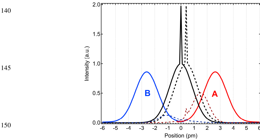
Figure 2. Spectral shapes of the thermally-broadened Rayleigh backscatter line with the thin Mie line on top of it (solid black) and the FPI bandpasses A and B (solid red and blue). The Doppler-shifted backscatter line (corresponding to an imaginary wind speed of 175 m/s) is shown as black dashed curve. The signals transmitted through the A and B bandpasses for the Doppler-shifted backscattering are illustrated by the dashed red and blue curves.
