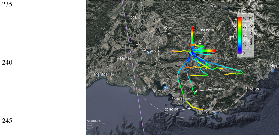
250 Figure 4. OHP wind lidar sampling location along north and east lines-of-sight (thick lines) and trajectories of 12 radiosondes launched from OHP for wind lidar validation (thinner curves) color-coded by the altitude a.s.l. Grey circles indicate the distance from OHP. Particular radiosonde flights are tagged by white arrows with indication of the flight date. The magenta line shows the ground track of Aeolus lidar (see Sect. 5).
