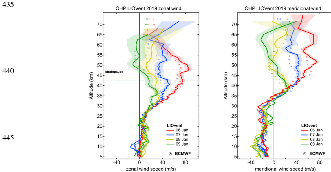
Figure 8. Ensembles of nightly-mean vertical profiles of zonal (left) and meridional (right) wind profiles obtained by LIOvent in January 2019 (solid curves) with statistical uncertainty shown as shading and the corresponding ECMWF Integrated Forecast System profiles (cross-circles). Horizontal dashed lines in the left panel indicate the stratopause altitude obtained from simultaneous temperature lidar measurements.
