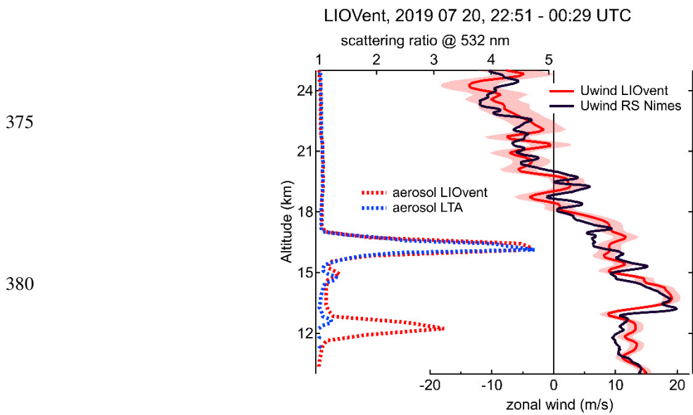
Figure 7. Zonal wind profiles (bottom axis) measured by the LIOvent wind lidar (red solid) and by MeteoFrance routine radiosounding launched from Nimes airport (100 km away from OHP, see Fig. 4) at 00 UT on 21.07.2019 (black solid). The date and time of LIOvent measurement is shown at the panel top. The aerosol scattering ratio profiles obtained using LIOvent zenith pointing (red dashed) and LTA lidar (blue dashed), showing volcanic aerosol layer at 16.2 km are plotted versus top axis. See text for details.
