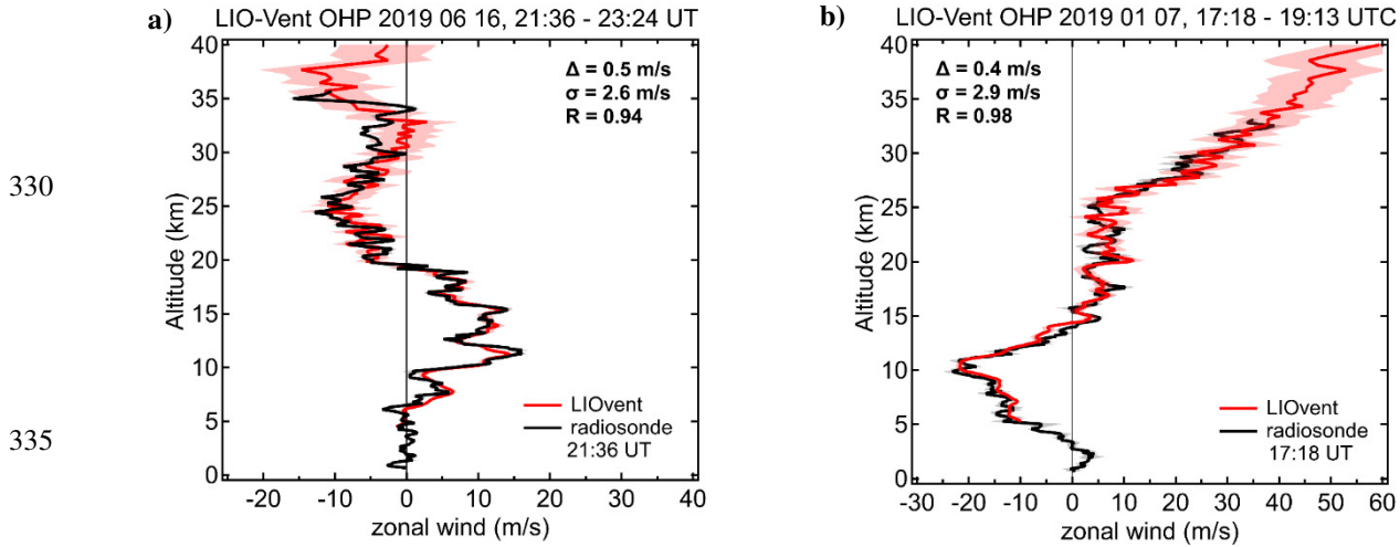
330 335 340 Figure 6. Selected cases of the lidar-radiosonde intercomparison of the zonal wind profiles in June (a) and January (b) 2019. The lidar measurement dates and times are given above the panels, the time of radiosonde launch on the same date is provided in the legend.
